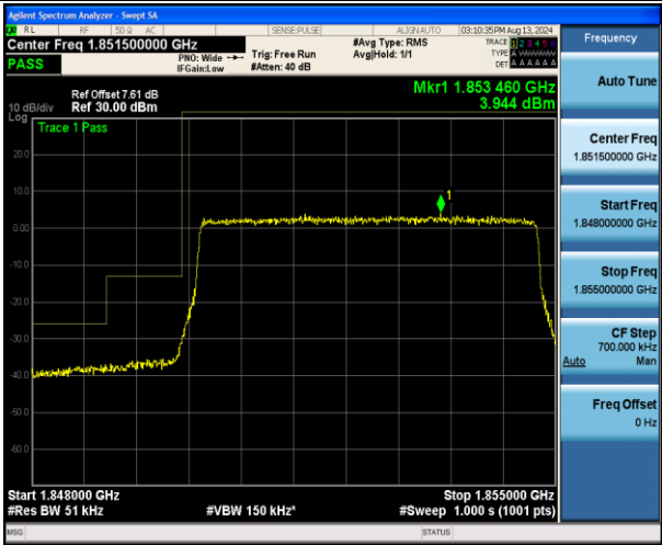
Band2_5MHz_16QAM_18625_25RB#0
