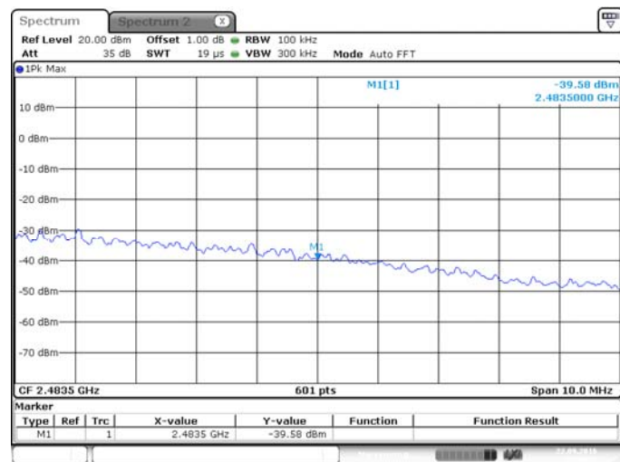
802.11n-20 MHz HIGH CHANNEL, Band Edge
