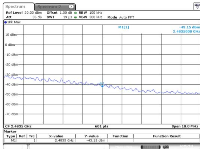
802.11g HIGH CHANNEL, Band Edge
