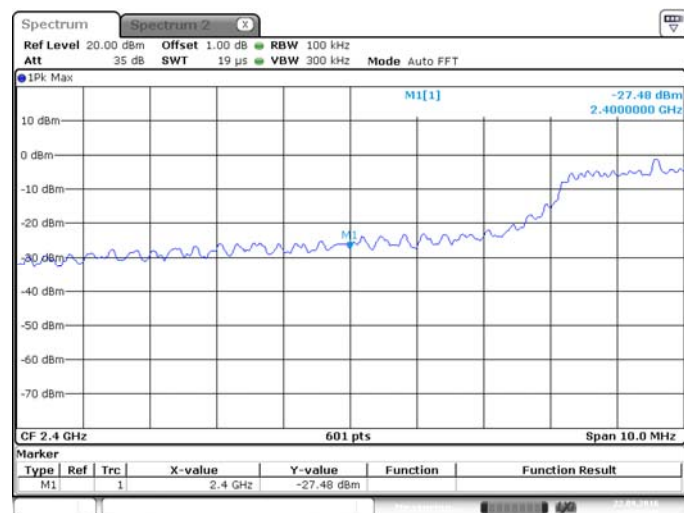
802.11n-20 MHz LOW CHANNEL, Band Edge
