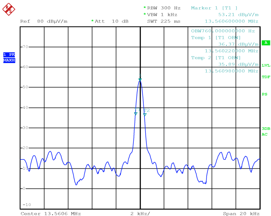
Figure 8.4-2: 99% dB bandwidth
