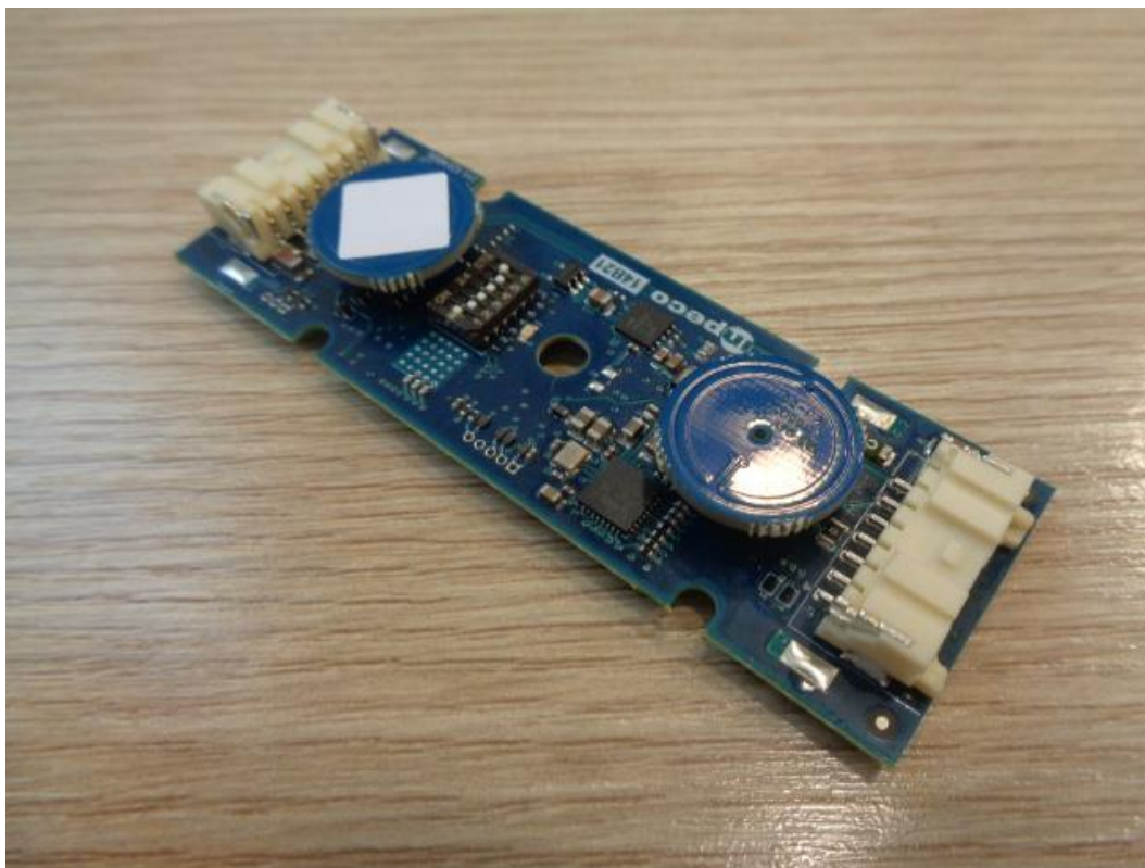
Figure 9.2-3: Internal view photo
