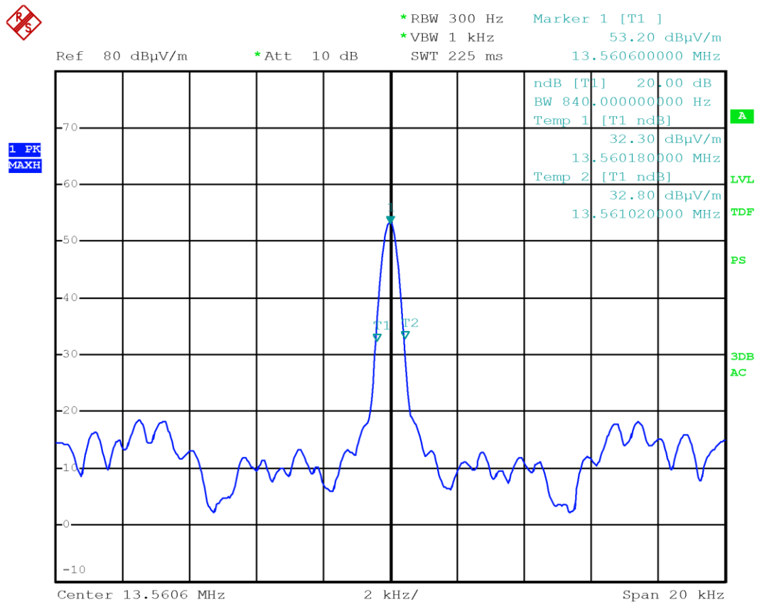
Figure 8.4-1: 20 dB bandwidth
