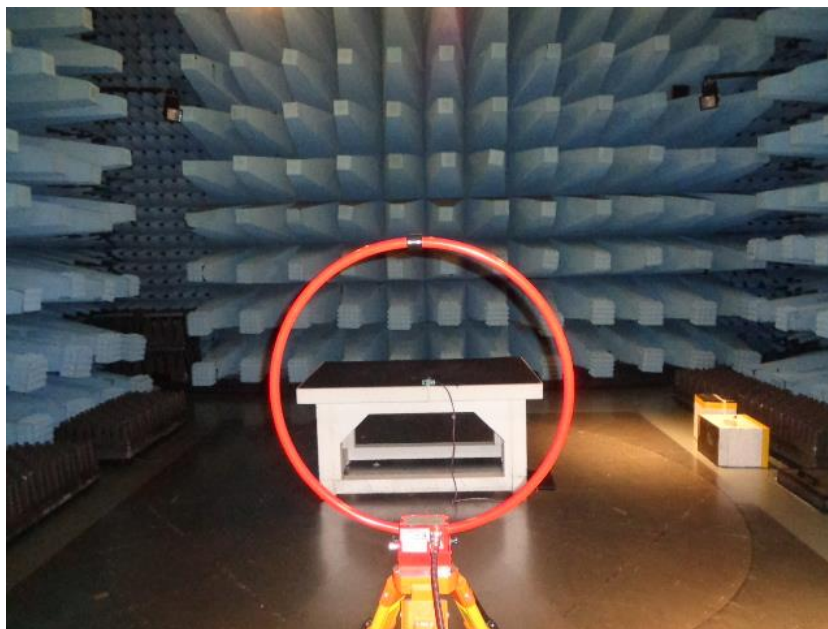
Figure 9.1-1: Radiated emissions set-up for frequencies below 30 MHz
