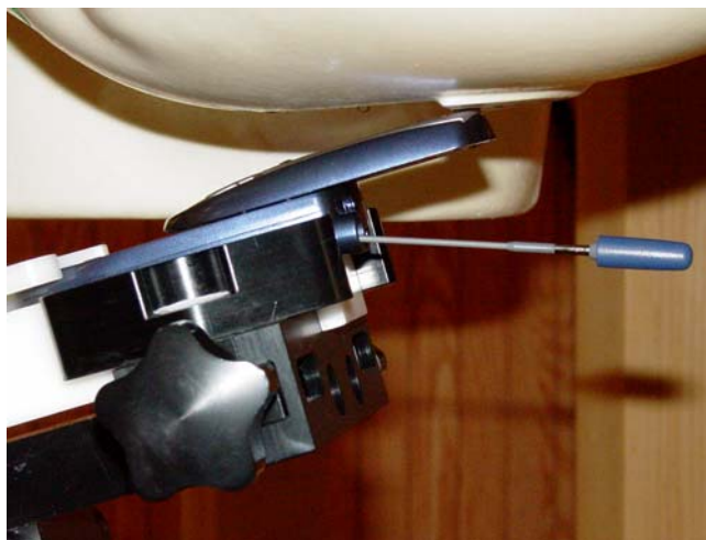
Figure 11.5 phone against the head (left tilt, slide opened, antenna extended position)
