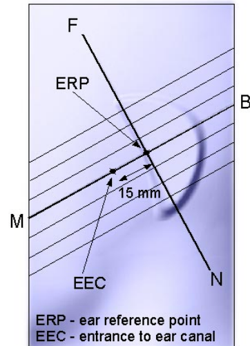
Figure 8-2 - Close up side view of phantom showing the ear region.
