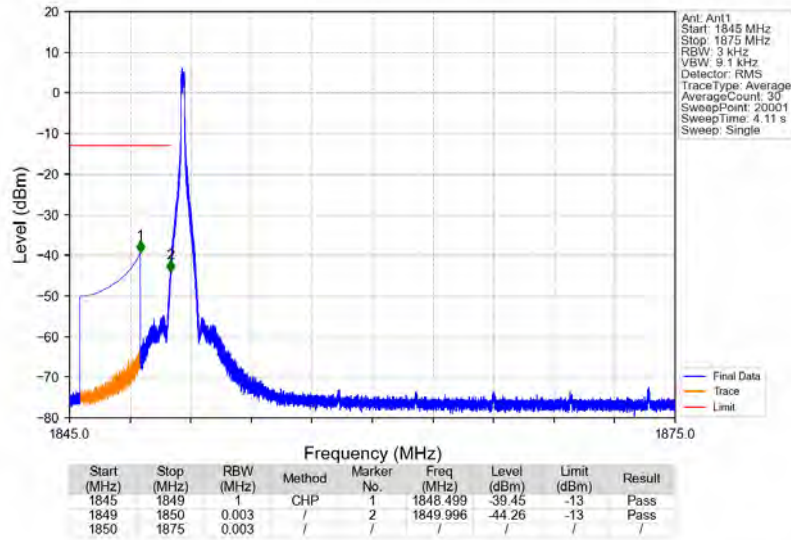
n25_15kHz_SISO_NTNV_25MHz_DFT-s-OFDM PI/2 BPSK_1862.5MHz_Edge_1RB_Left
