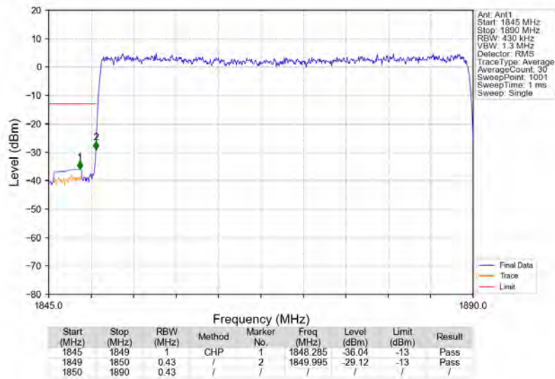
n25_15kHz_SISO_NTNV_40MHz_DFT-s-OFDM PI/2 BPSK_1870MHz_Outer_Full
