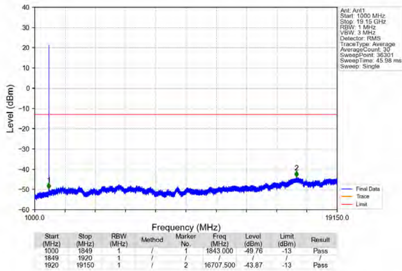
n25_15kHz_SISO_NTNV_30MHz_DFT-s-OFDM PI/2 BPSK_1865MHz_Edge_1RB_Left
