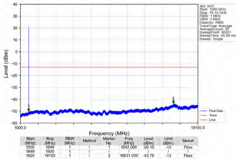
n25_15kHz_SISO_NTNV_40MHz_DFT-s-OFDM PI/2 BPSK_1870MHz_Edge_1RB_Left
