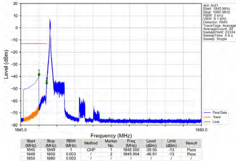
n25_15kHz_SISO_NTNV_30MHz_DFT-s-OFDM PI/2 BPSK_1865MHz_Edge_1RB_Left
