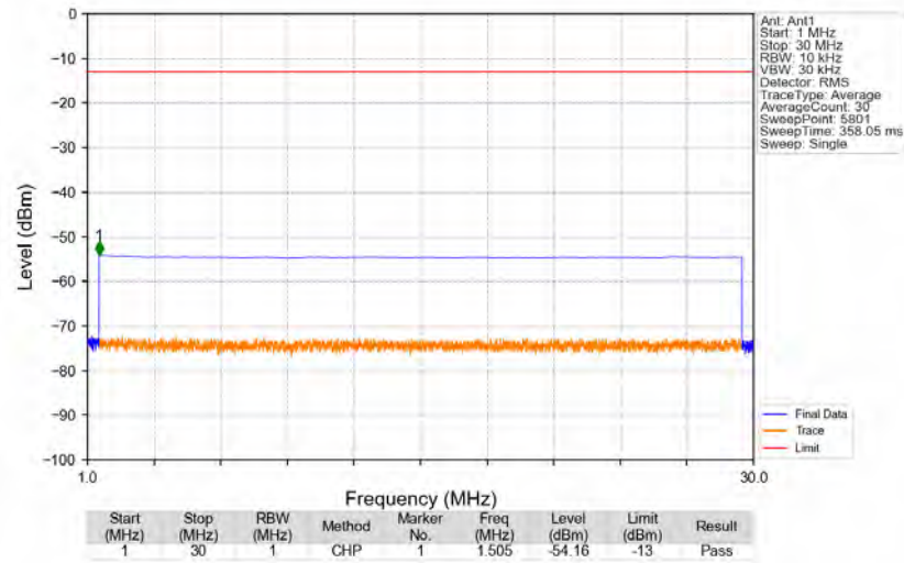
n25_15kHz_SISO_NTNV_40MHz_DFT-s-OFDM PI/2 BPSK 1882.5MHz_Edge_1RB_Left
