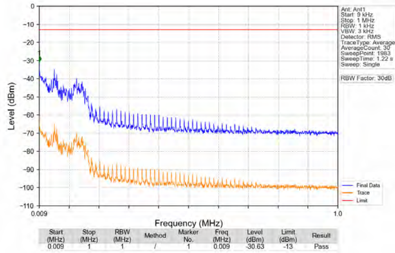
n25_15kHz_SISO_NTNV_40MHz_DFT-s-OFDM PI/2 BPSK 1882.5MHz_Edge_1RB_Left
