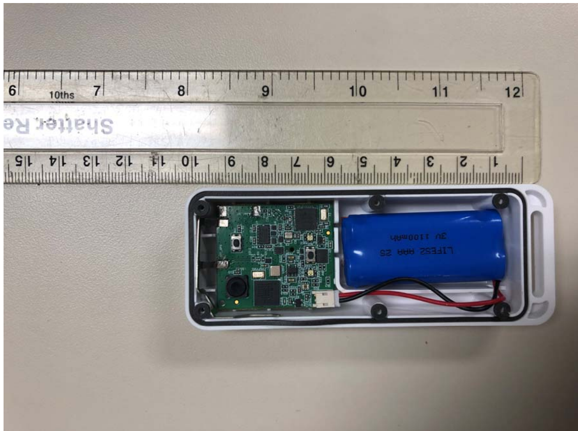
Figure 2 - Parsyl Trek - Internal View – PWB & Battery in Case with scale
