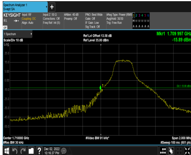
Band4-1.4MHz-QPSK-19957-1RB#5
