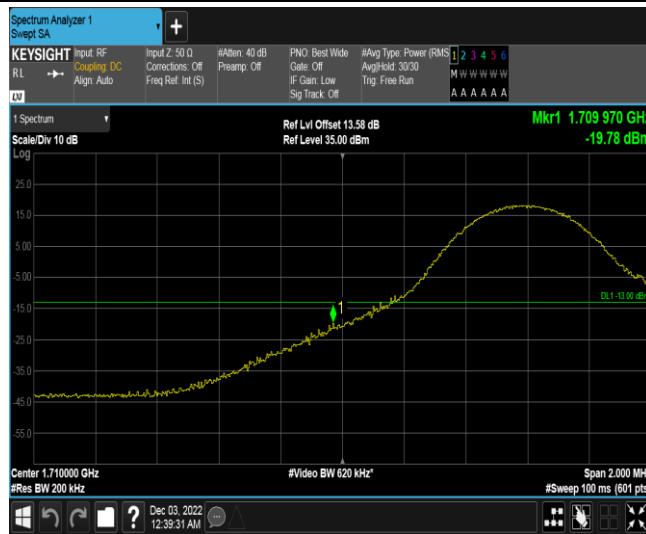
Band4-10MHz-16QAM-20000-1RB#49
