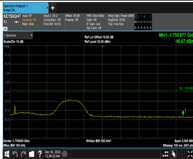
Band4-5MHz-QPSK-20375-1RB#24
