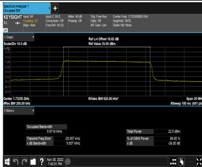
Band4-10MHz-16QAM-20350-50RB#0
