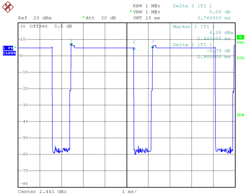
39 Channel @ 2DH5
