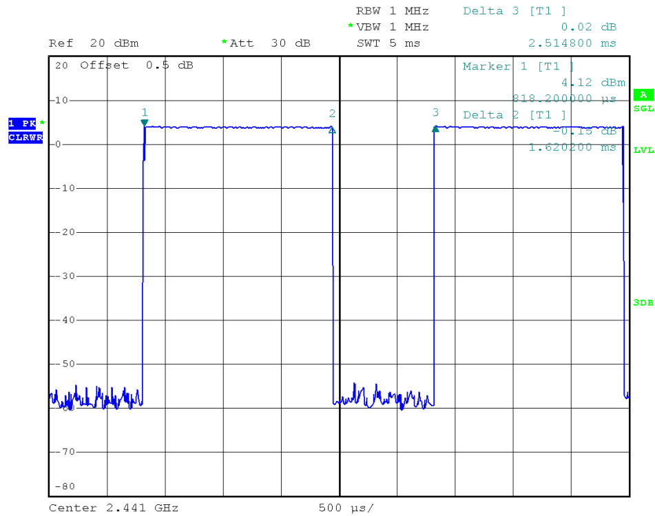
39 Channel @ DH3
