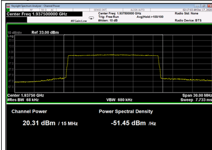
Figure 223: QPSK 15MHz B.W.; 1937.5MHz, 30kHz
