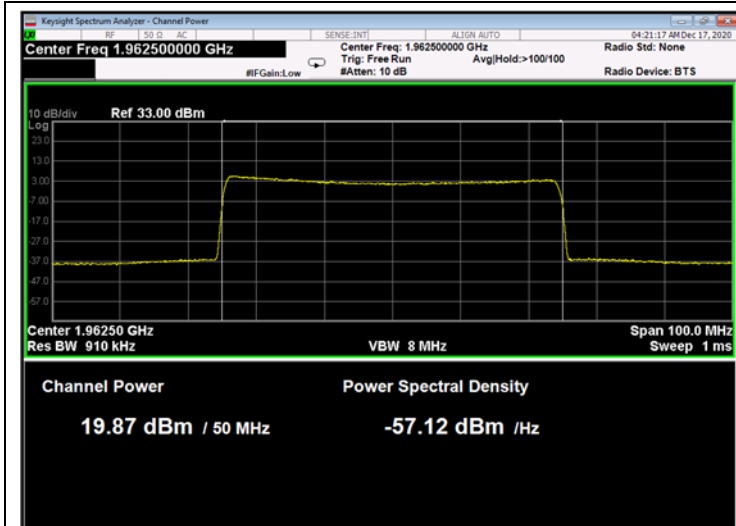
Figure 261: QPSK 50MHz B.W.; 1962.5MHz, 15kHz
