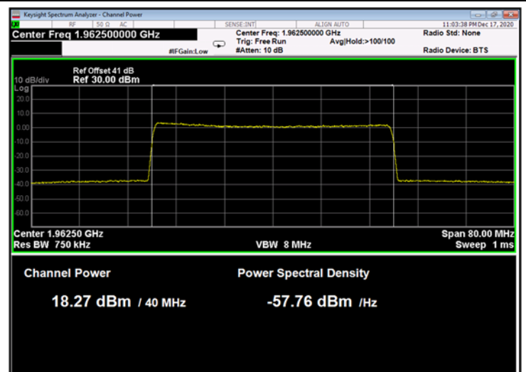
Figure 186: 256QAM 40MHz B.W.; 1962.5MHz, 15kHz
