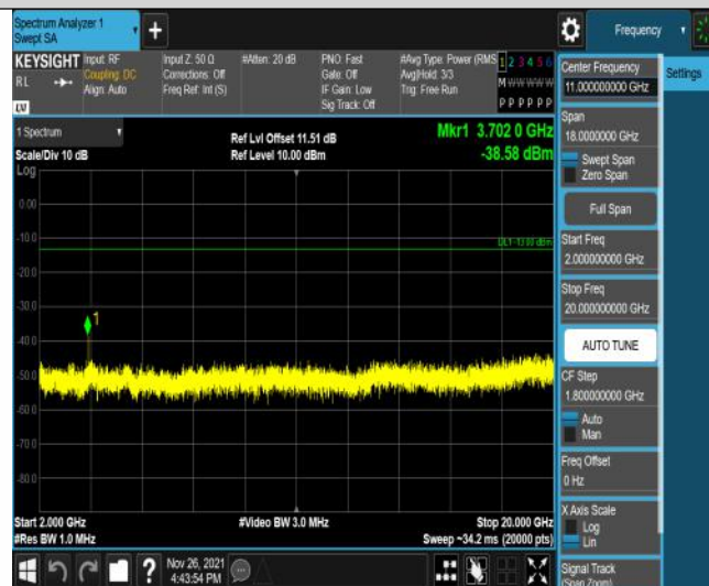
Band25-5MHz-QPSK-26065-25RB#0-Range3:2000~20000MHz
