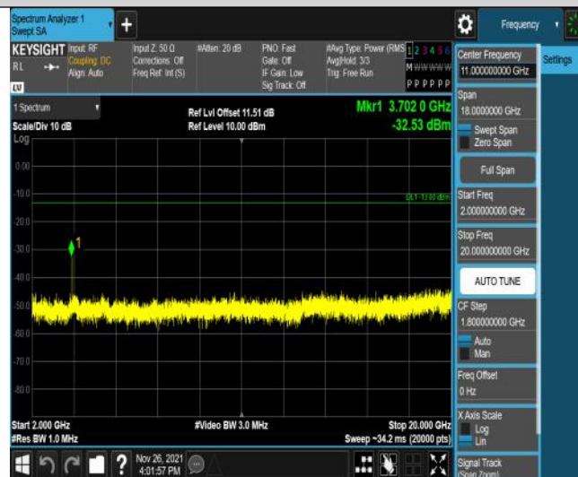
Band25-1.4MHz-16QAM-26047-6RB#0-Range3:2000~20000MHz
