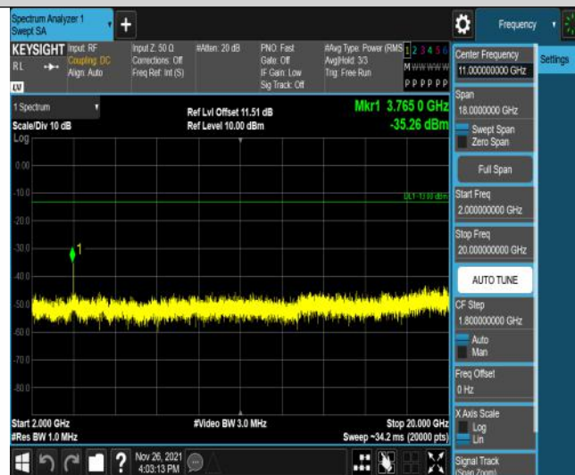
Band25-1.4MHz-16QAM-26365-6RB#0-Range3:2000~20000MHz
