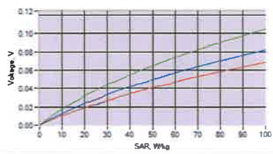
SAR @ HL1800
