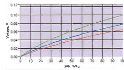
SAR @ HL2450
