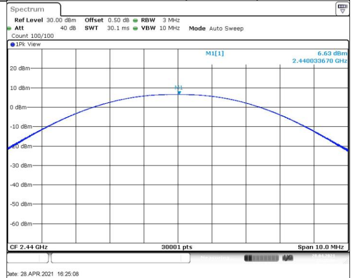
Channel 19 (2440MHz)
