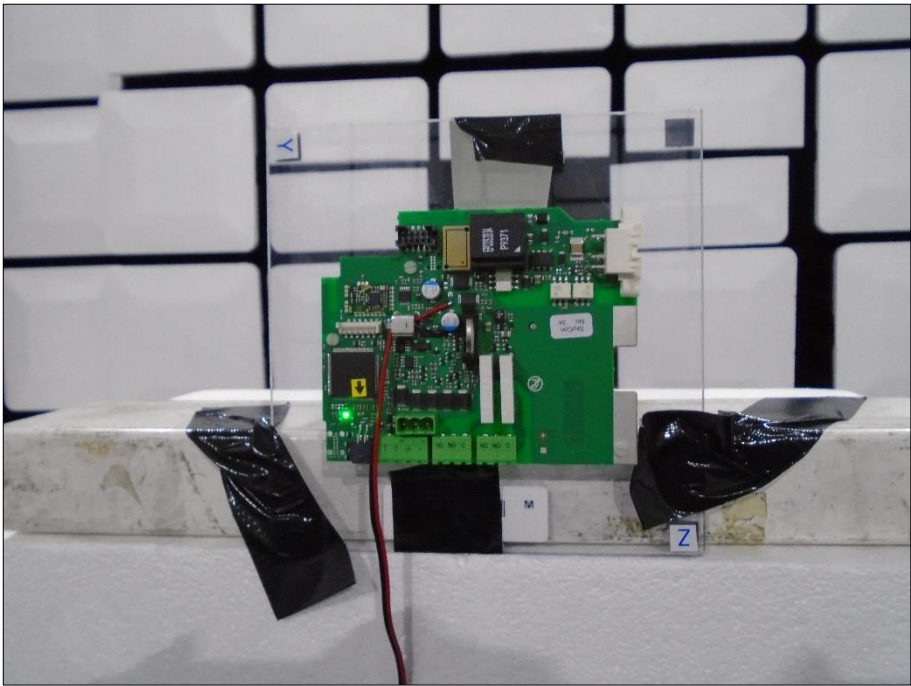
Figure 70 - Orientation Z
