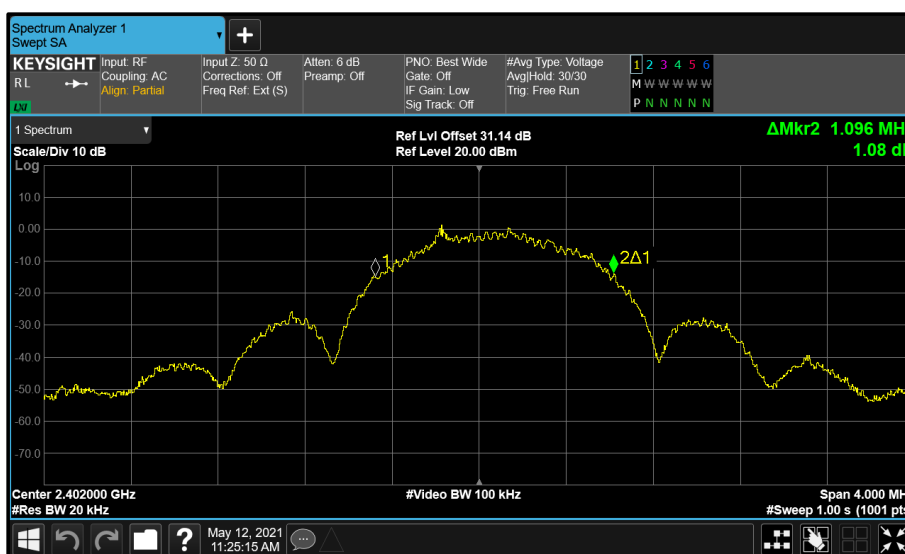
Figure 3 - BLE (A) 2402 MHz (CH37) 99% Bandwidth
