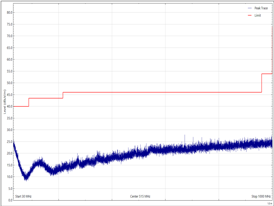
Figure 46 - 2480 MHz, 30 MHz to 1 GHz, Horizontal, EUT Orientation X
