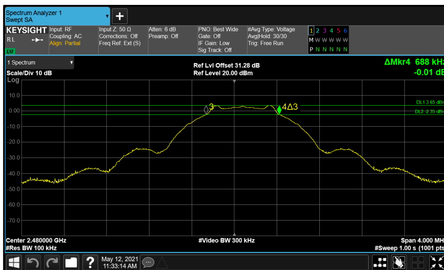
Figure 8 - BLE (A) 2480 MHz (CH39) 6 dB Bandwidth
