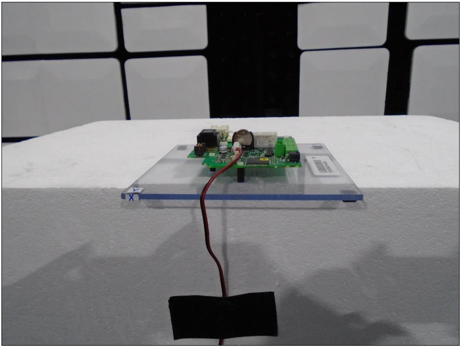
Figure 68 - Orientation X
