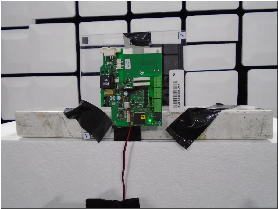
Figure 69 - Orientation Y
