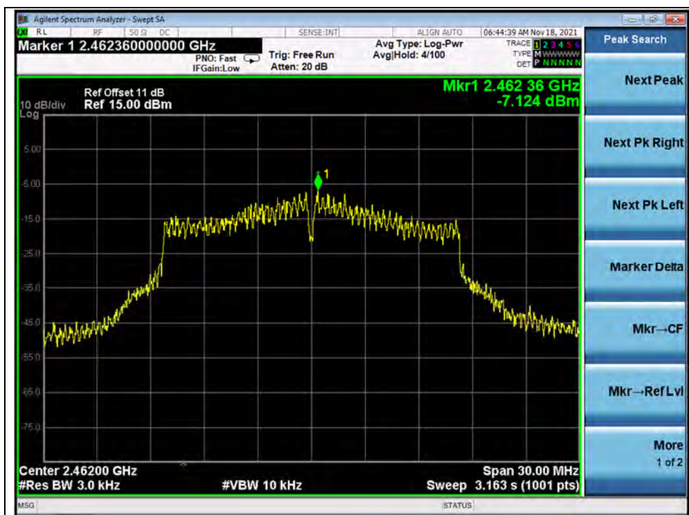
(Channel 11, 802.11g)
