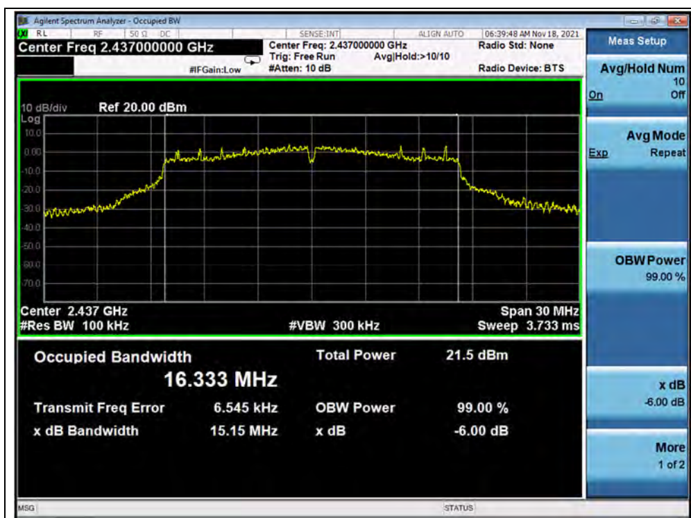
(Channel 6, 802.11g)
