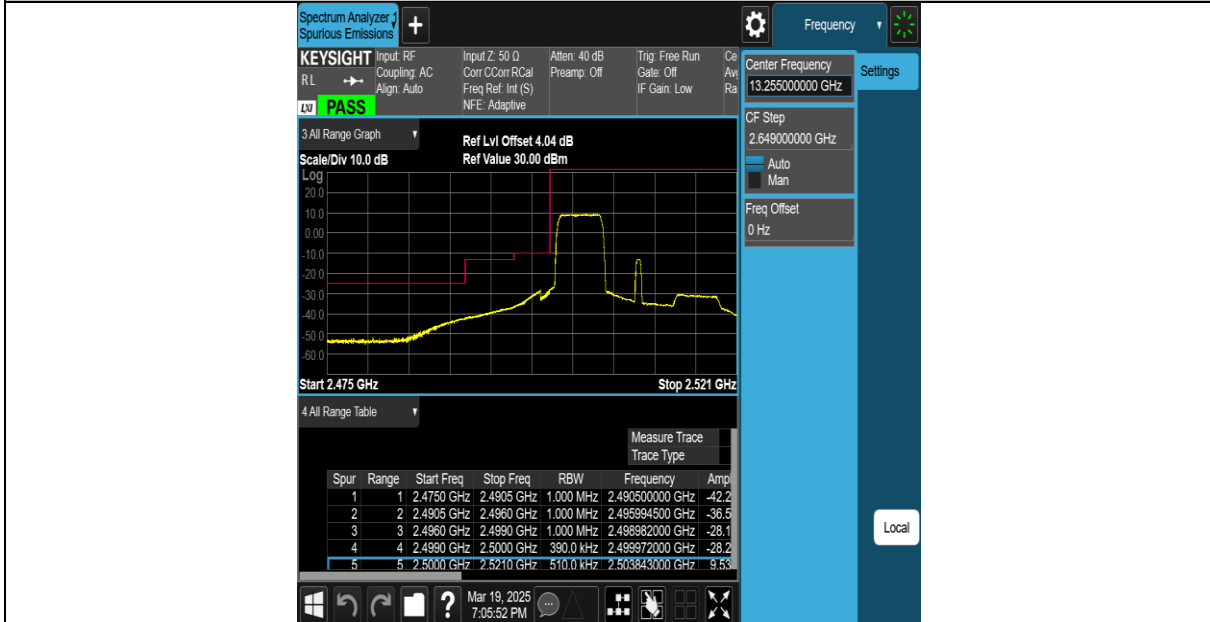
Band7-20MHz-16QAM-21350-27RB#73-PASS
