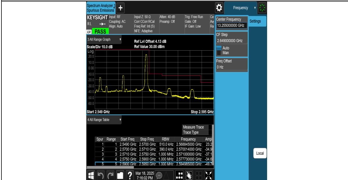
Band7-20MHz-16QAM-20850-1RB#0-PASS
