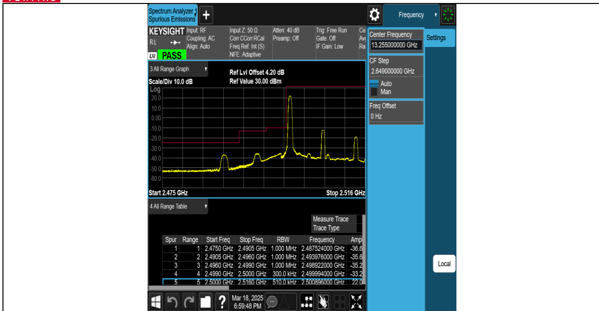
Band7-15MHz-QPSK-20825-75RB#0-PASS
