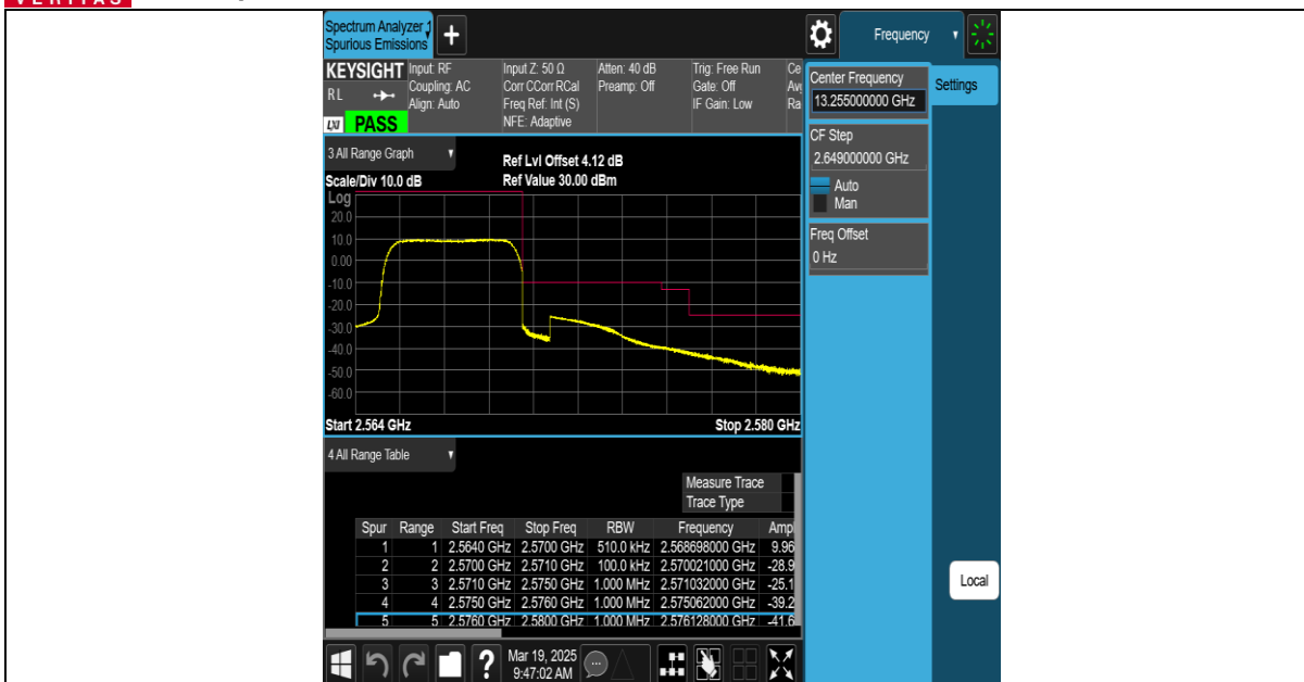
Band7-5MHz-16QAM-21425-1RB#24-PASS
