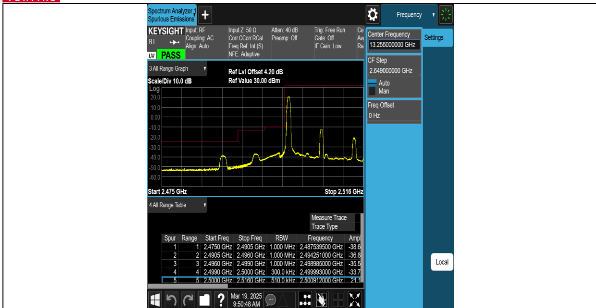
Band7-15MHz-16QAM-20825-27RB#0-PASS
