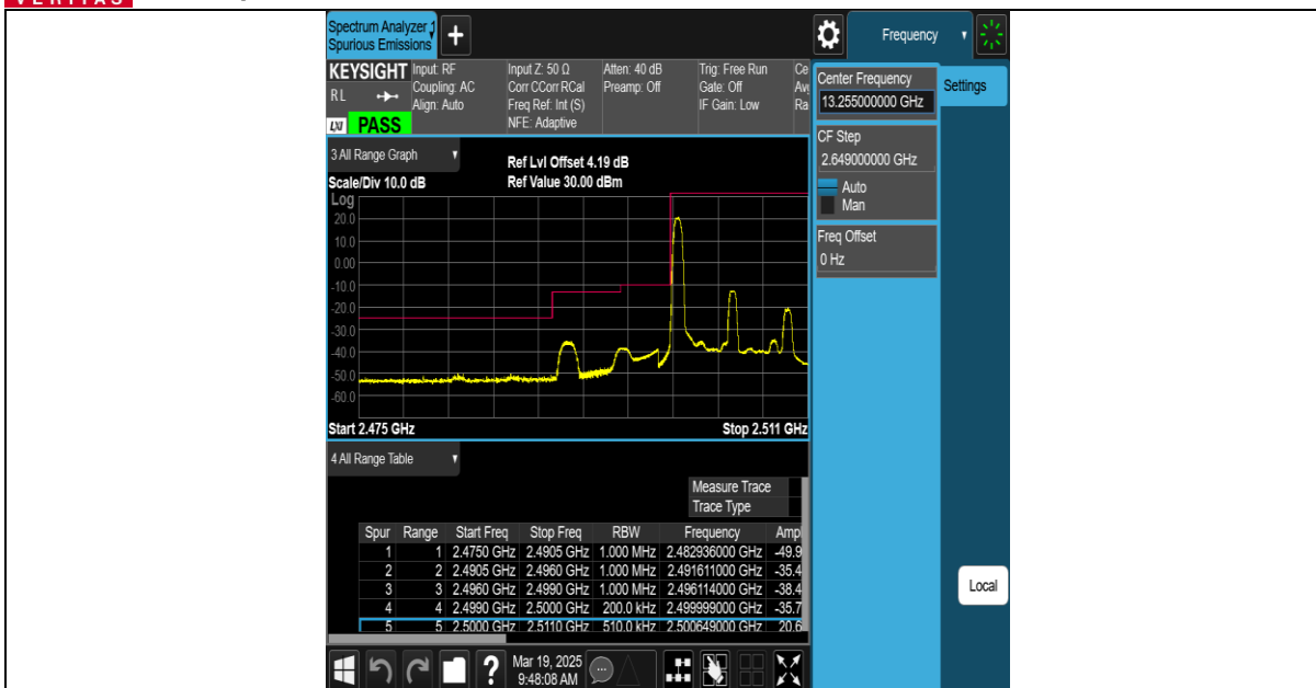
Band7-10MHz-16QAM-20800-27RB#0-PASS
