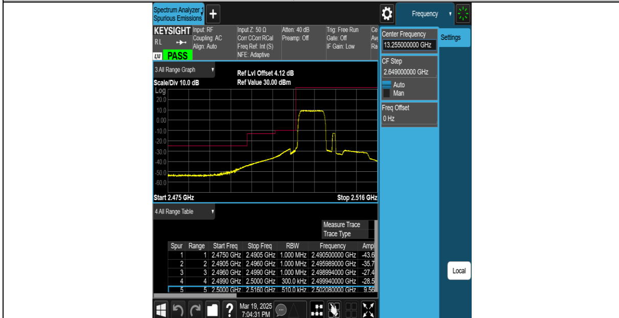
Band7-15MHz-16QAM-21375-27RB#48-PASS
