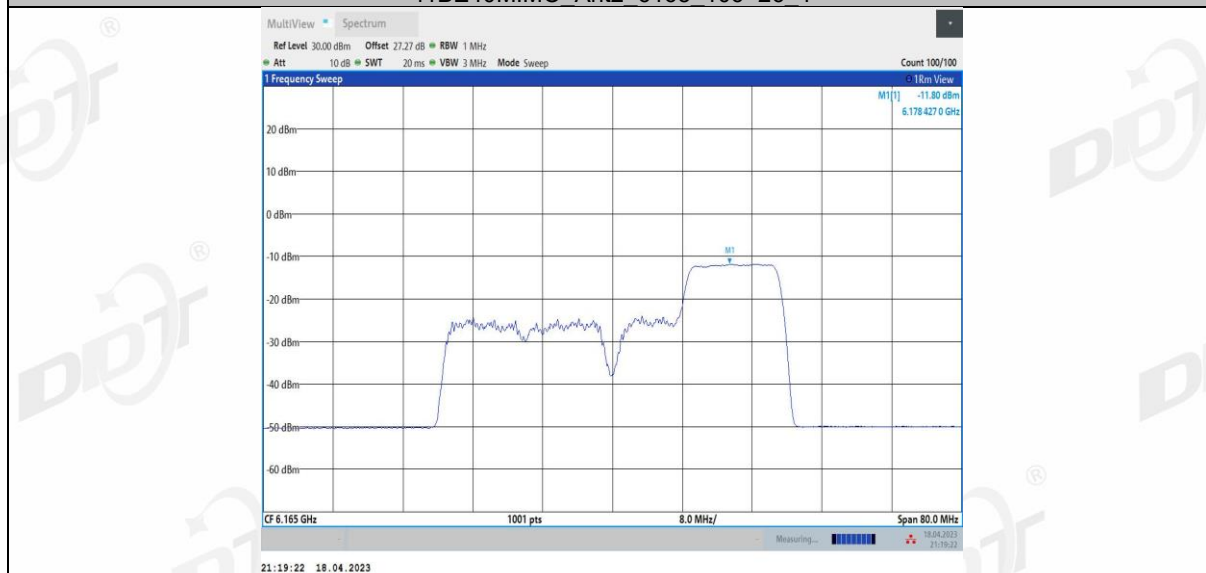
11BE40MIMO Ant3 6165 106+26 3
