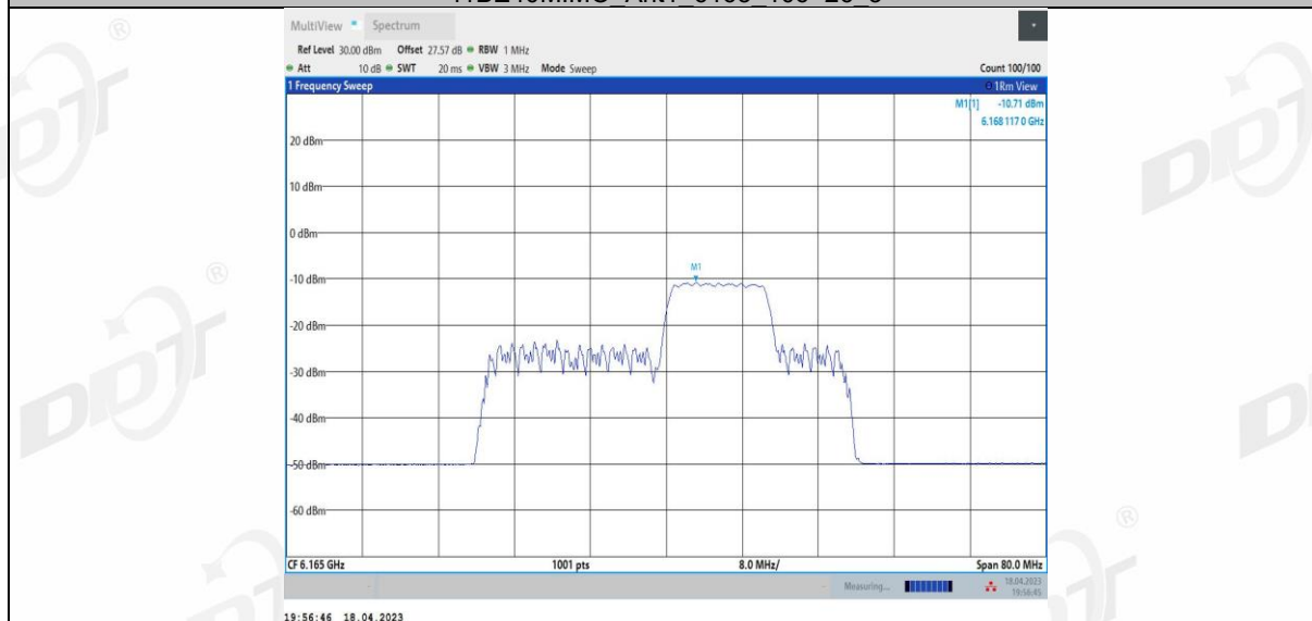
11BE40MIMO Ant1_6165_106+26_4
