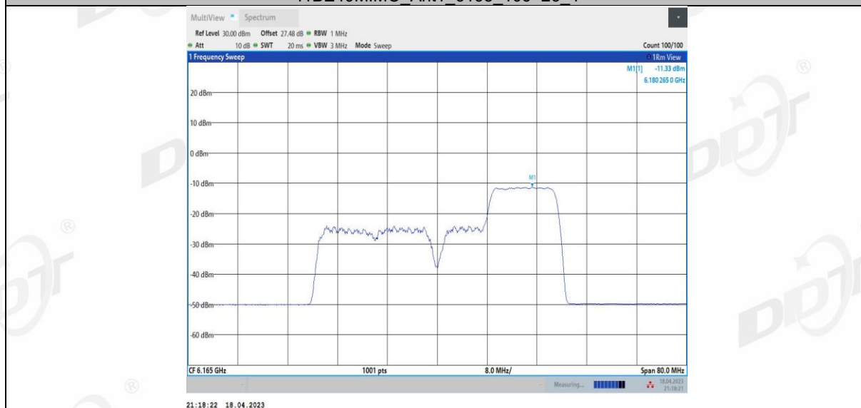
11BE40MIMO Ant2_6165_106+26_3
