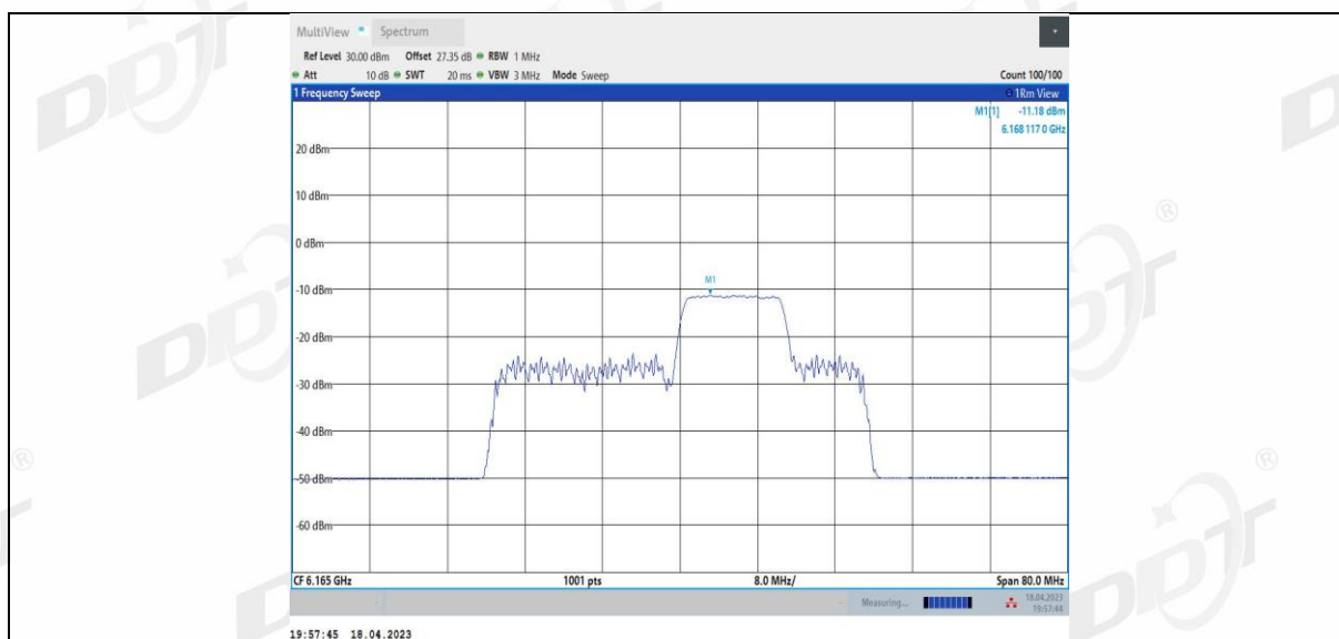
11BE40MIMO Ant2 6165 106+26 4
