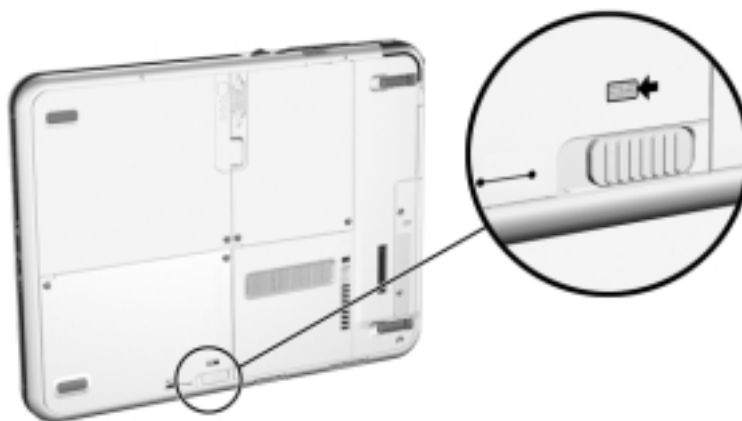
Sliding the attachment release switch on the tablet PC
