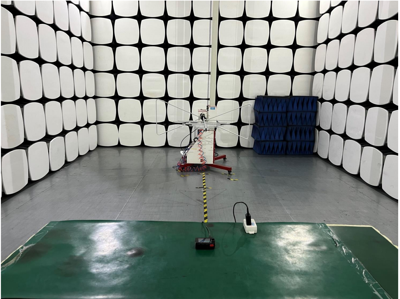
30MHz~1GHz Test setup
