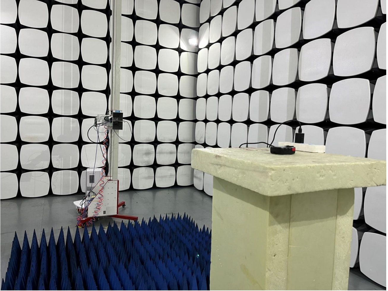
Above 1G Test setup
