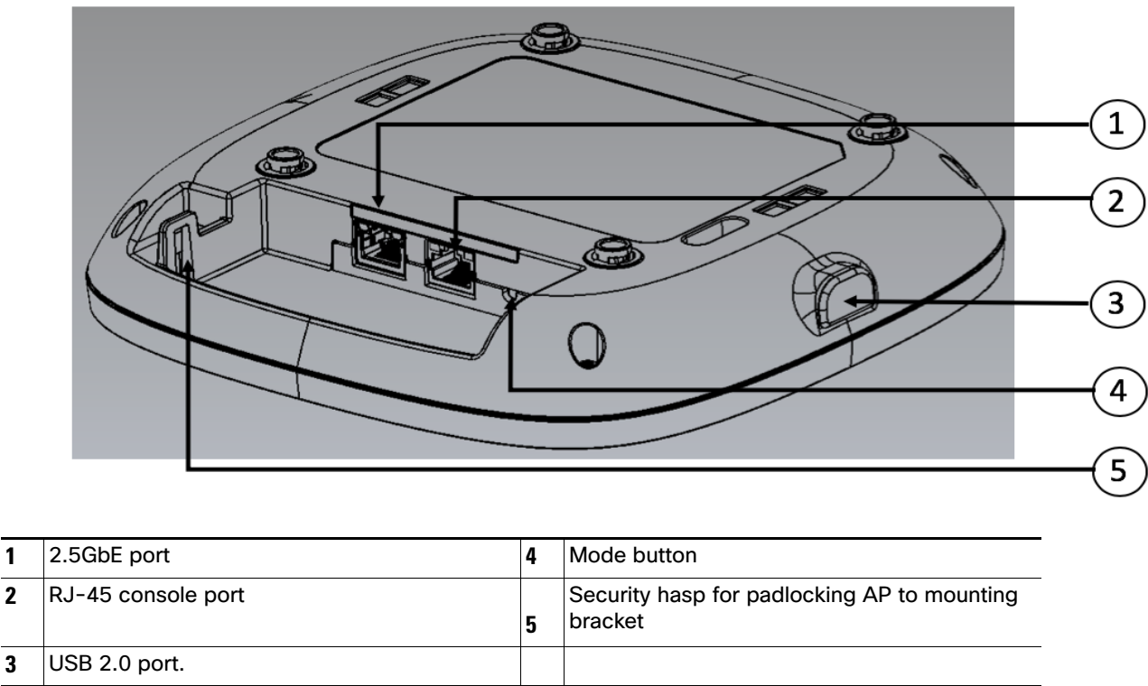
Figure 2 Ports and Connectors on the Head of the 9115AXI Model
