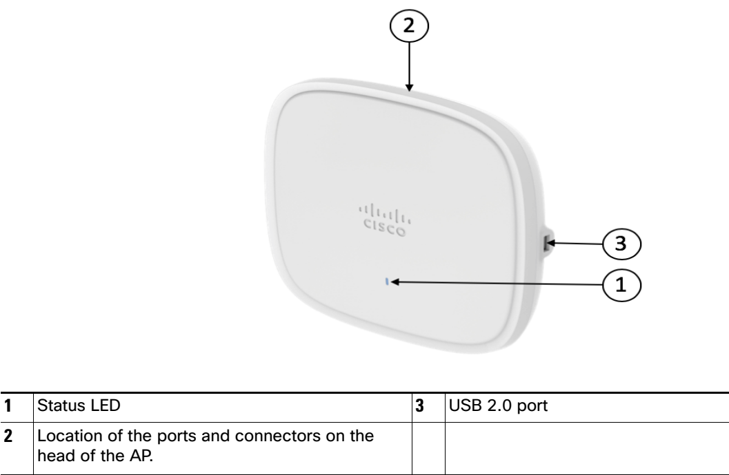
Figure 2 Ports and Connectors on the Head of the 9115AXI Model
