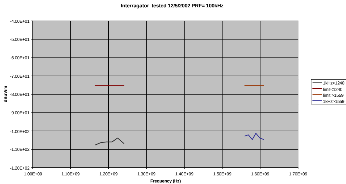
FIGURE 4.3-1 INTERRAGATOR RMS (GPS; RBW=1kHz)
