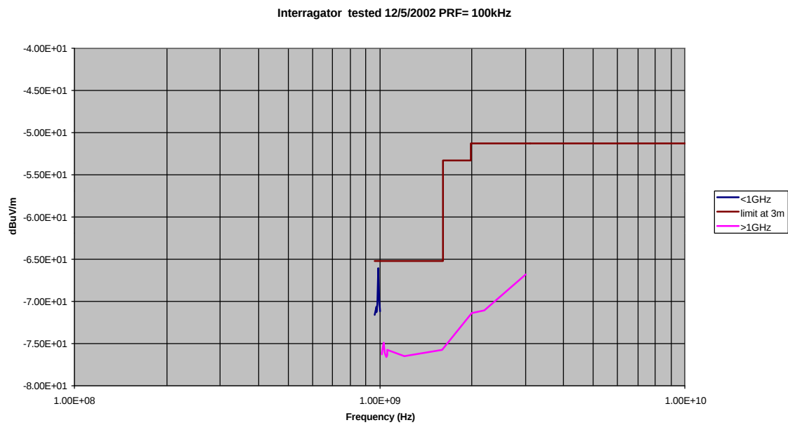
FIGURE 4.2-1 INTERRAGATOR RMS (RBW=1MHz)
