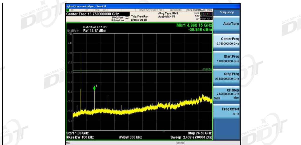
2DH5_Ant1_2402_0~Reference
