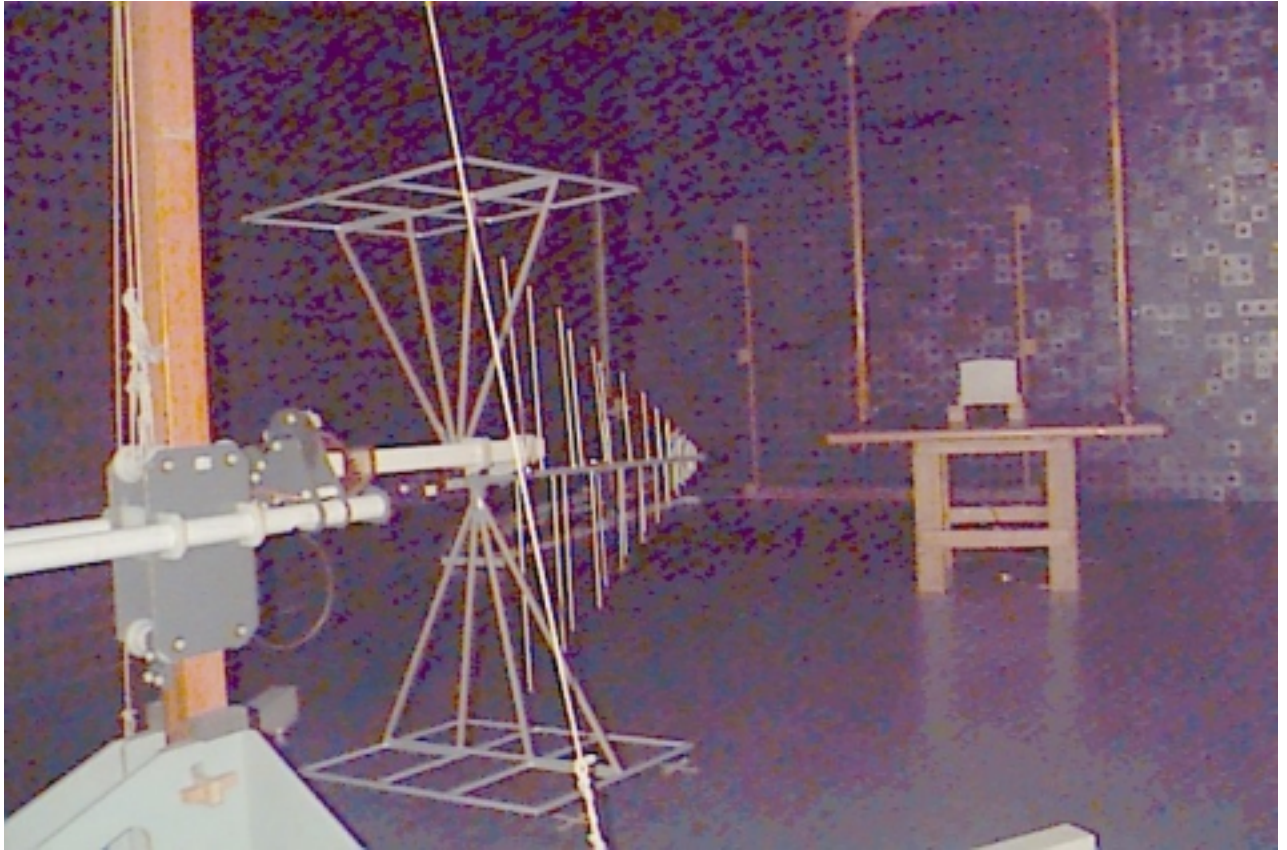
Photograph No.3 Radiated emission measurement test setup
