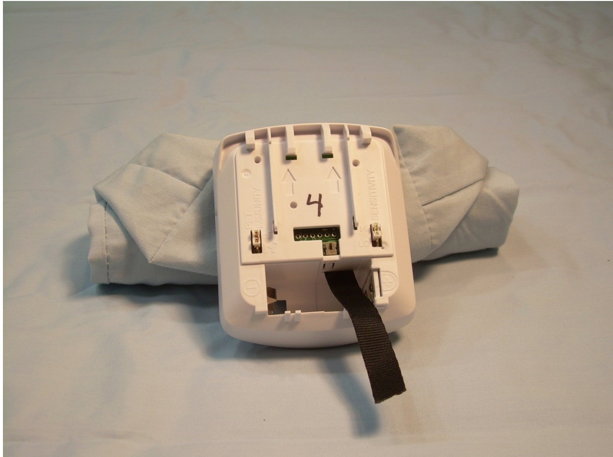
Photograph 5 – View of the EUT with Mounting Plate Removed
