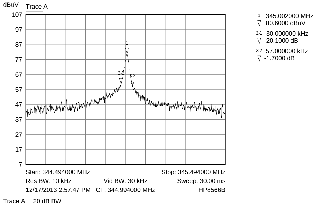
Bandwidth Plot
