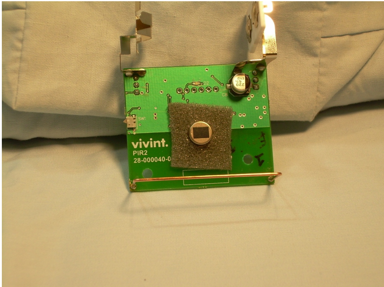
Photograph 9 – View of the Sensor/Antenna Side of the PCB
