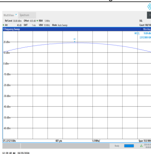
Band30-5MHz-QPSK-27735-25RB#0-PASS
