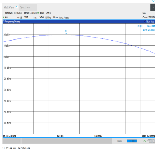
Band30-5MHz-QPSK-27735-12RB#0-PASS
