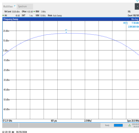
Band30-10MHz-QPSK-27710-50RB#0-PASS
