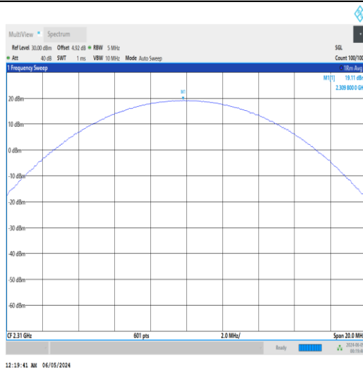
Band30-10MHz-QPSK-27710-25RB#12-PASS
