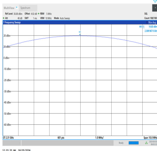
Band30-5MHz-QPSK-27710-12RB#6-PASS
