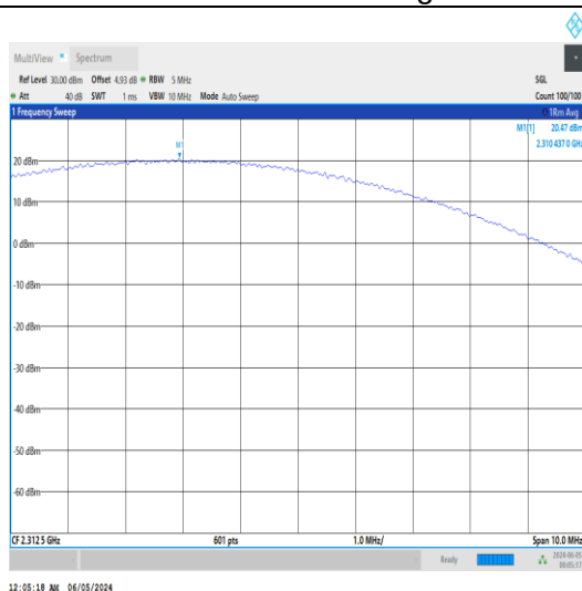
Band30-5MHz-QPSK-27735-1RB#0-PASS
