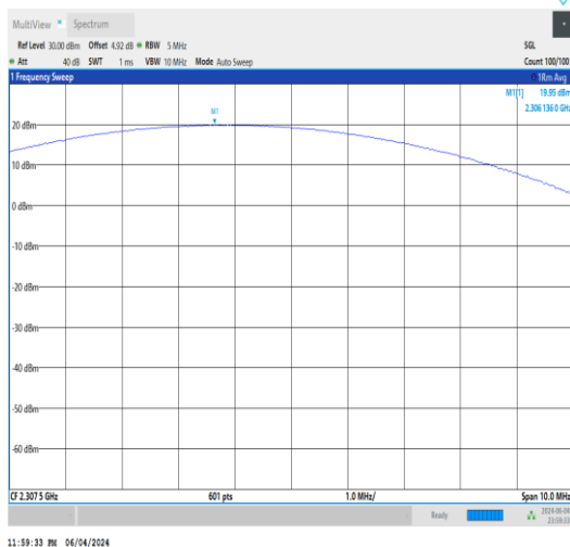
Band30-5MHz-QPSK-27685-12RB#0-PASS
