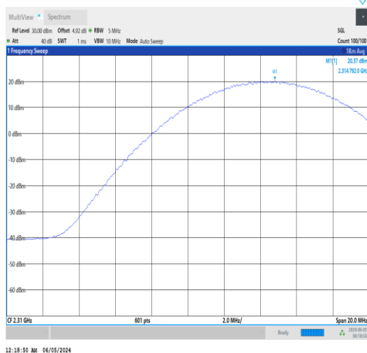
Band30-10MHz-QPSK-27710-1RB#49-PASS
