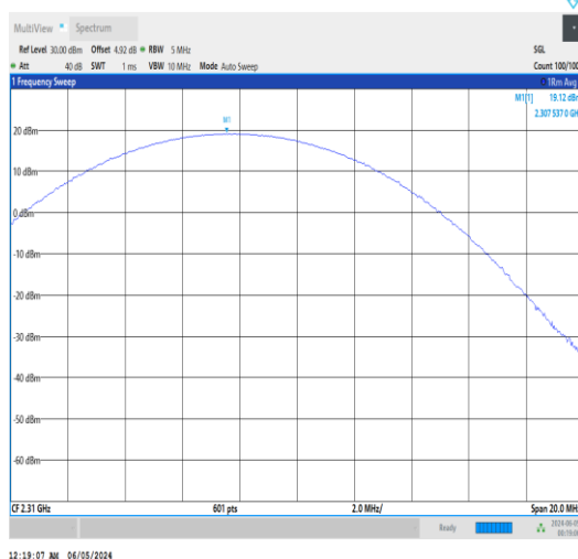
Band30-10MHz-QPSK-27710-25RB#0-PASS
