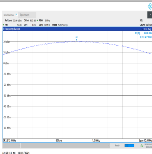
Band30-5MHz-QPSK-27735-1RB#12-PASS
