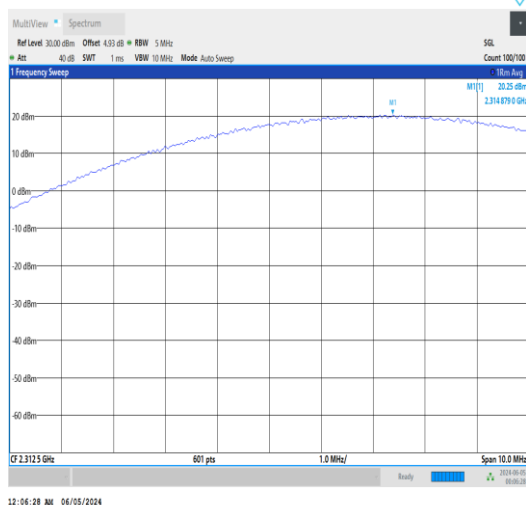
Band30-5MHz-QPSK-27735-1RB#24-PASS
