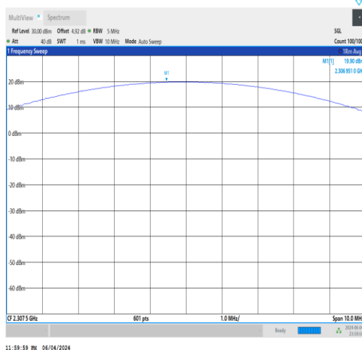
Band30-5MHz-QPSK-27685-12RB#6-PASS
