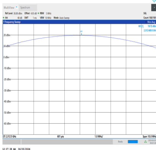
Band30-5MHz-QPSK-27735-12RB#6-PASS
