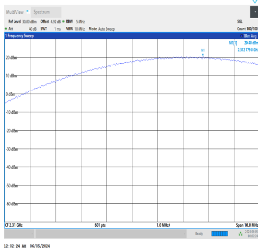
Band30-5MHz-QPSK-27710-1RB#24-PASS
