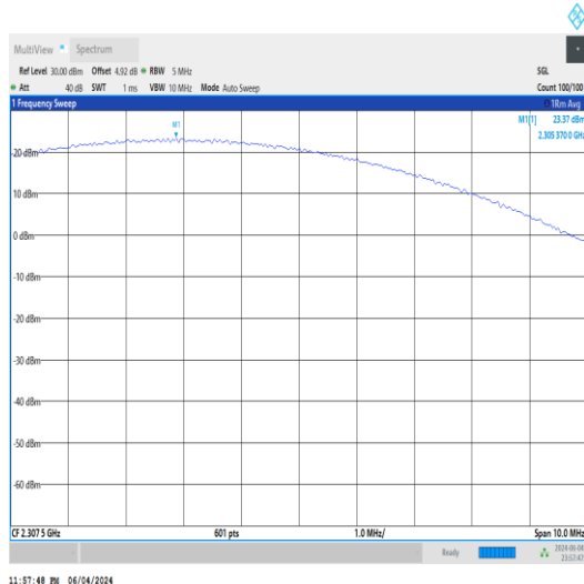
Band30-5MHz-QPSK-27685-1RB#0-PASS
