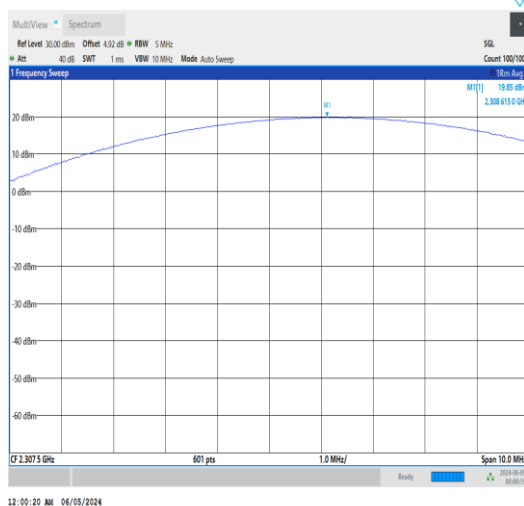
Band30-5MHz-QPSK-27685-12RB#13-PASS
