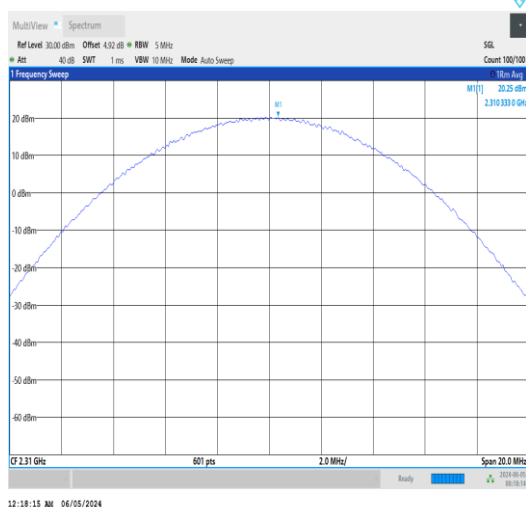
Band30-10MHz-QPSK-27710-1RB#24-PASS
