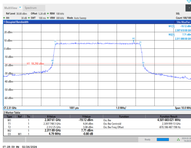
Band30-5MHz-16QAM-27710-25RB#0
