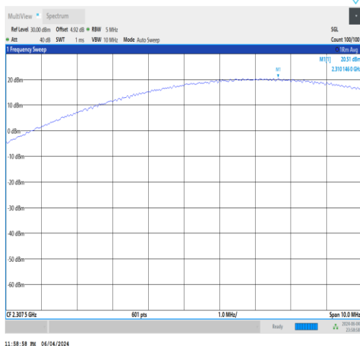
Band30-5MHz-QPSK-27685-1RB#24-PASS
