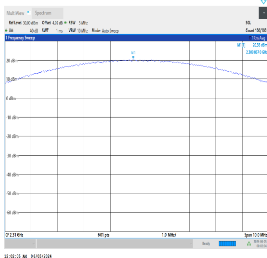
Band30-5MHz-QPSK-27710-1RB#12-PASS
