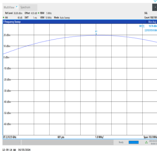
Band30-5MHz-QPSK-27735-12RB#13-PASS
