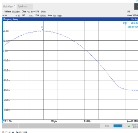
Band30-10MHz-QPSK-27710-1RB#0-PASS
