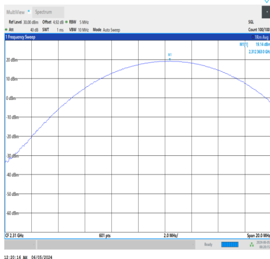
Band30-10MHz-QPSK-27710-25RB#25-PASS
