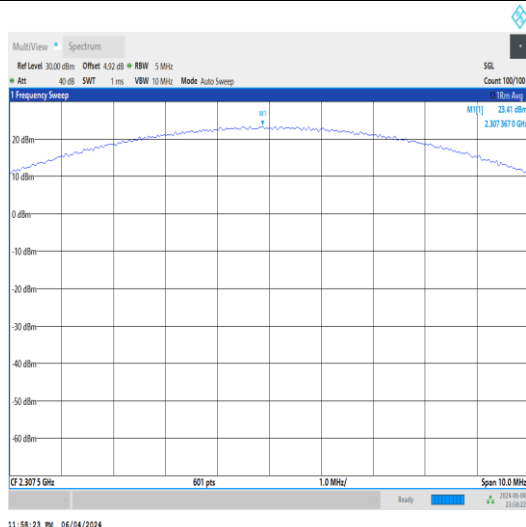
Band30-5MHz-QPSK-27685-1RB#12-PASS
