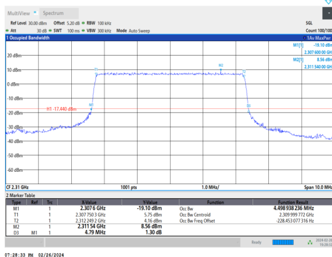
Band30-5MHz-16QAM-27710-25RB#0
