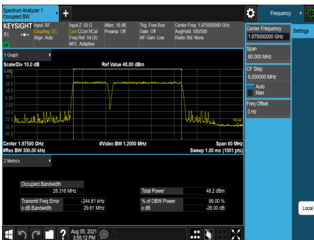
Plot 7-83. Occupied Bandwidth Plot (B2_10M+20M_2C_64QAM - High Channel, Port 3)
