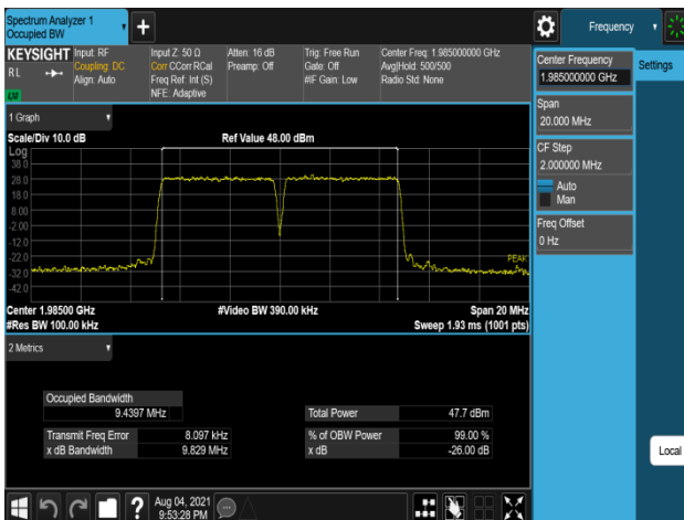
Plot 7-59. Occupied Bandwidth Plot (B2_5M+5M_2C_64QAM - High Channel, Port 0)
