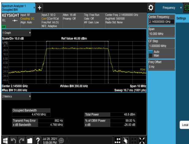
Plot 7-113. Occupied Bandwidth Plot (B66_5M_1C_QPSK - Mid Channel, Port 0)
