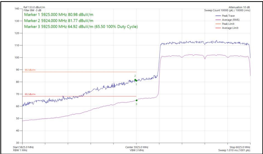
Figure 204 - 802.11ax HE80, SU, SISO, Core 1 - 5985 MHz Band Edge Frequency 5925 MHz
