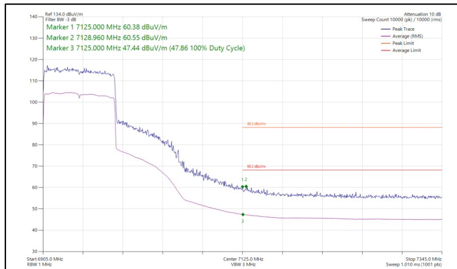
Figure 218 - 802.11ax HE80, SU, TxBF, Core 0 - Core 1 - 6945 MHz Band Edge Frequency 7125 MHz
