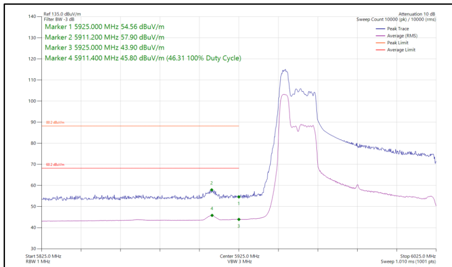
Figure 201 - 802.11ax HE80, RU 52-37, SISO, Core 0 - 5985 MHz Band Edge Frequency 5925 MHz
