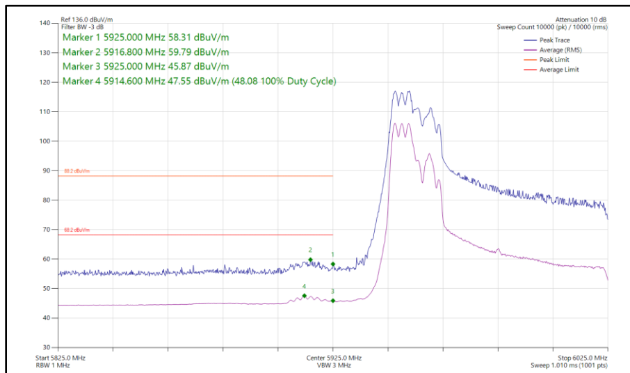
Figure 209 - 802.11ax HE80, RU 106-53, CDD, Core 0 - Core 1 - 5985 MHz Band Edge Frequency 5925 MHz
