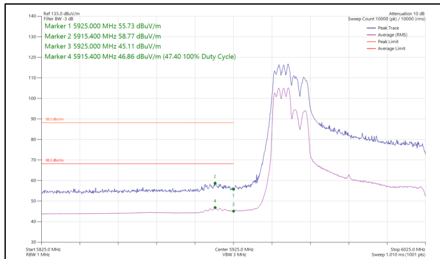
Figure 213 - 802.11ax HE80, RU 106-53, SDM, Core 0 - Core 1 - 5985 MHz Band Edge Frequency 5925 MHz
