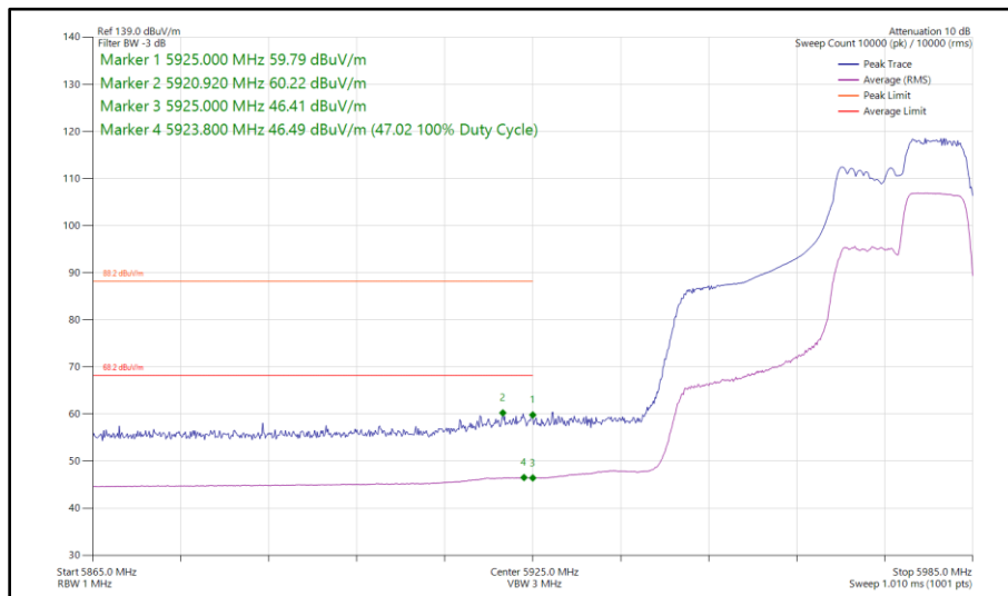
Figure 189 - 802.11ax HE40, RU 106-56, SISO, Core 1 - 5965 MHz Band Edge Frequency 5925 MHz
