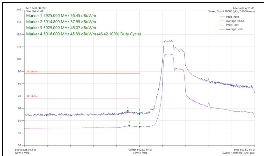
Figure 205 - 802.11ax HE80, RU 106-53, SISO, Core 1 - 5985 MHz Band Edge Frequency 5925 MHz
