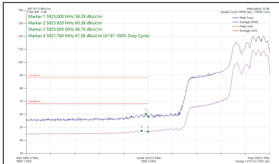
Figure 197 - 802.11ax HE40, RU 106-56, SDM, Core 0 - Core 1 - 5965 MHz Band Edge Frequency 5925 MHz
