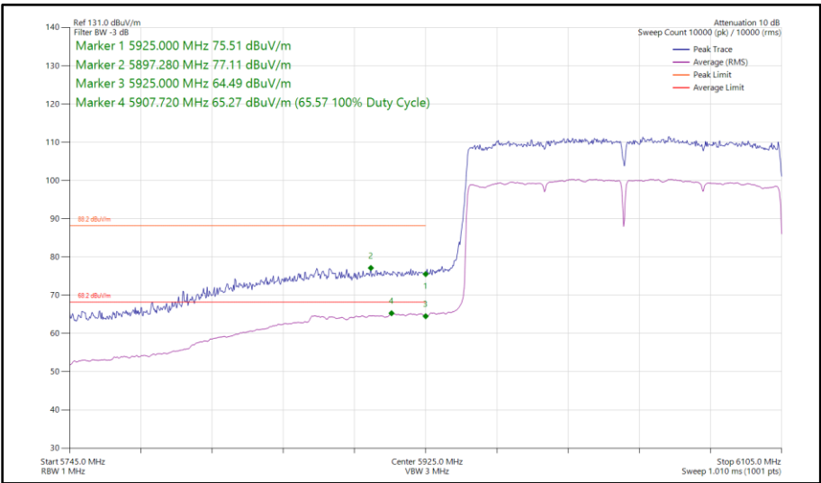
Figure 224 - 802.11ax HE160, SU, SISO, Core 1 - 6025 MHz Band Edge Frequency 5925 MHz
