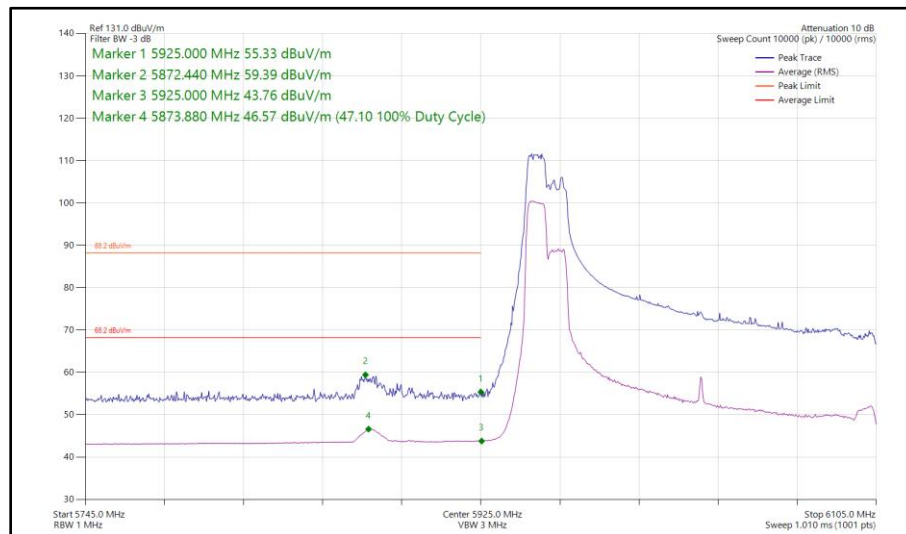
Figure 221 - 802.11ax HE160, RU 106-53P, SISO, Core 0 - 6025 MHz Band Edge Frequency 5925 MHz
