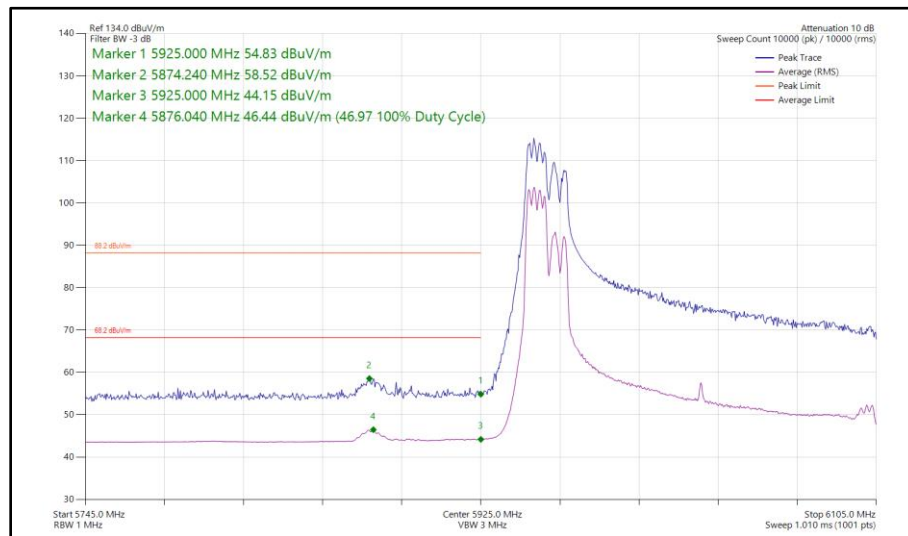
Figure 229 - 802.11ax HE160, RU 106-53P, CDD, Core 0 - Core 1 - 6025 MHz Band Edge Frequency 5925 MHz
