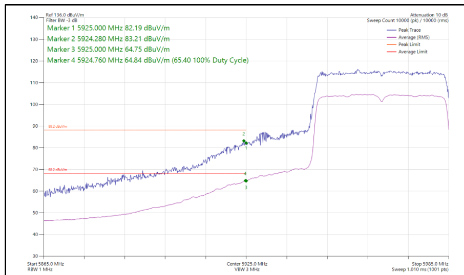
Figure 188 - 802.11ax HE40, SU, SISO, Core 1 - 5965 MHz Band Edge Frequency 5925 MHz
