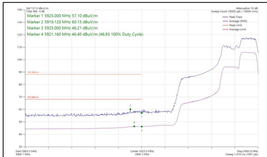
Figure 185 - 802.11ax HE40, RU 106-56, SISO, Core 0 - 5965 MHz Band Edge Frequency 5925 MHz
