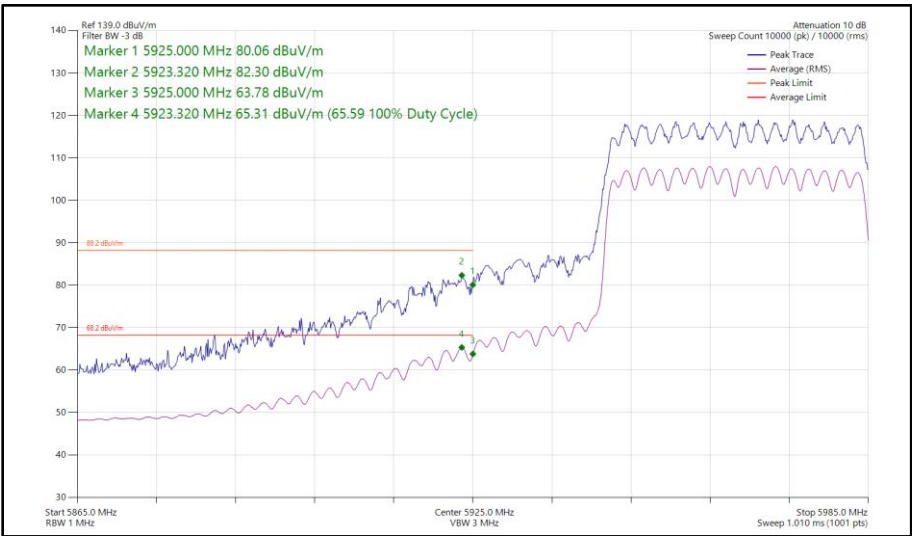
Figure 192 - 802.11ax HE40, SU, CDD, Core 0 - Core 1 - 5965 MHz Band Edge Frequency 5925 MHz
