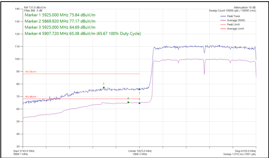
Figure 220 - 802.11ax HE160, SU, SISO, Core 0 - 6025 MHz Band Edge Frequency 5925 MHz
