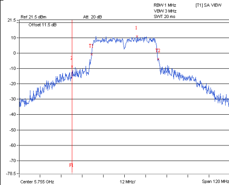
802.11ac(VHT40)_Chain2 / CH151
