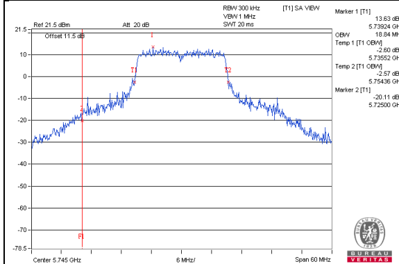
802.11ac(VHT20)_Chain2 / CH149
