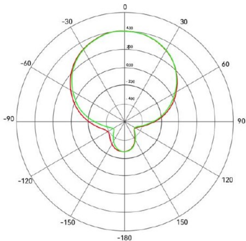
Field diagram
