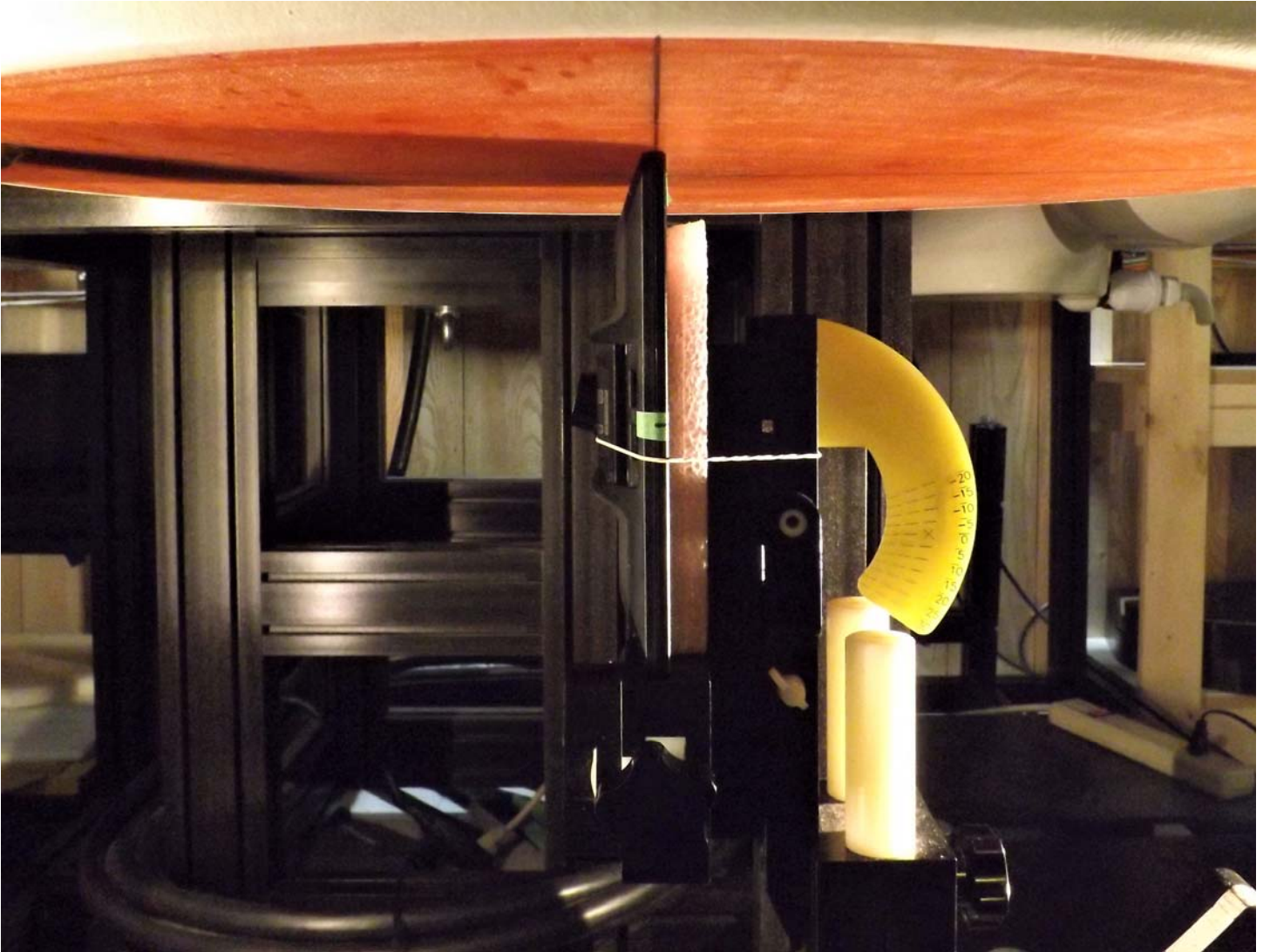
Figure C.3 – Setup Photo, Left Edge - Far
