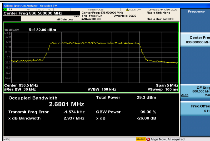
Band5-3MHz-16QAM-20525-15RB#0-2.6801
