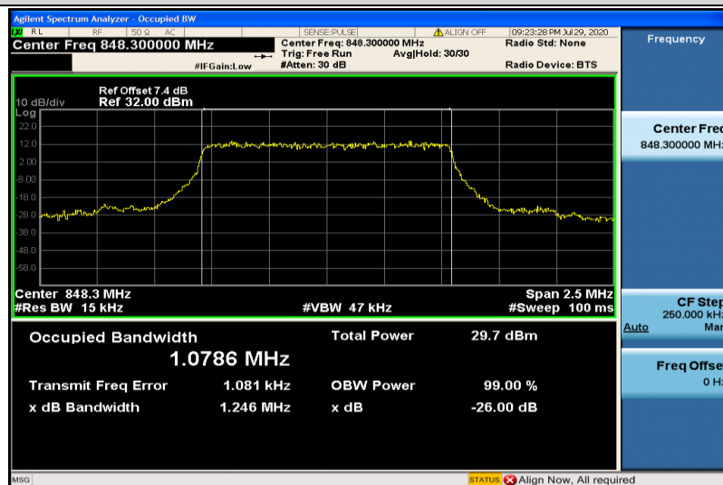
Band5-1.4MHz-QPSK-20643-6RB#0-1.0786
