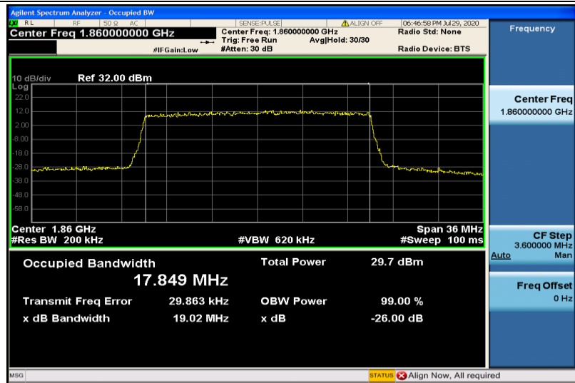
Band2-20MHz-16QAM-18700-100RB#0-17.849
