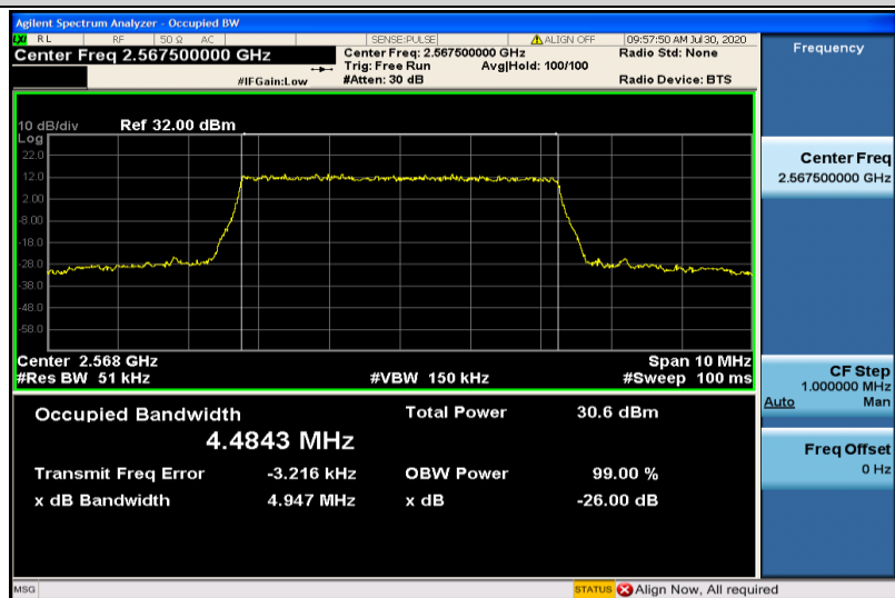
Band7-5MHz-QPSK-21425-25RB#0-4.4843
