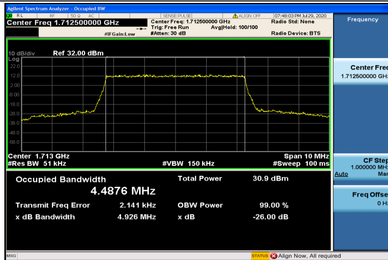
Band4-5MHz-QPSK-19975-25RB#0-4.4876
