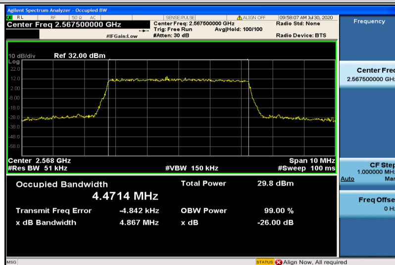
Band7-5MHz-16QAM-21425-25RB#0-4.4714
