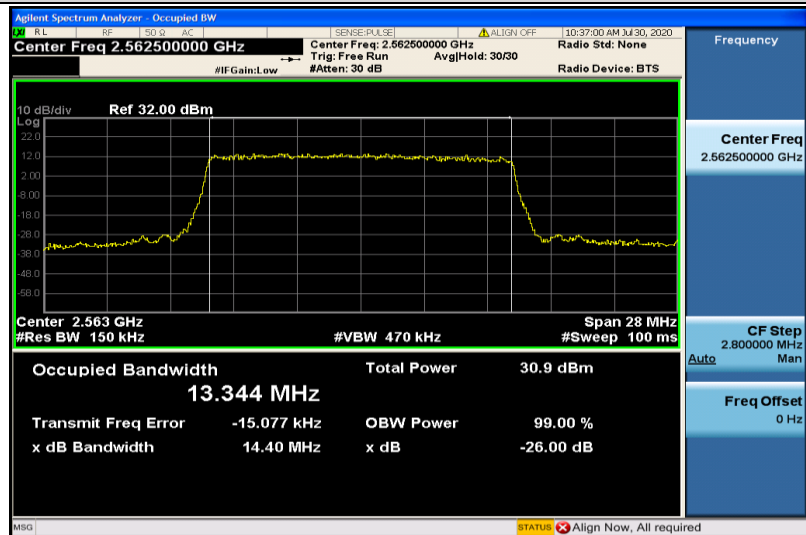
Band7-15MHz-QPSK-21375-75RB#0-13.344
