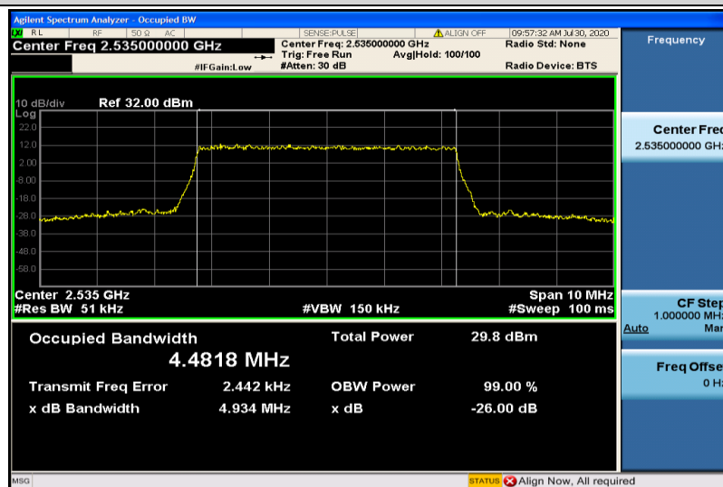
Band7-5MHz-16QAM-21100-25RB#0-4.4818
