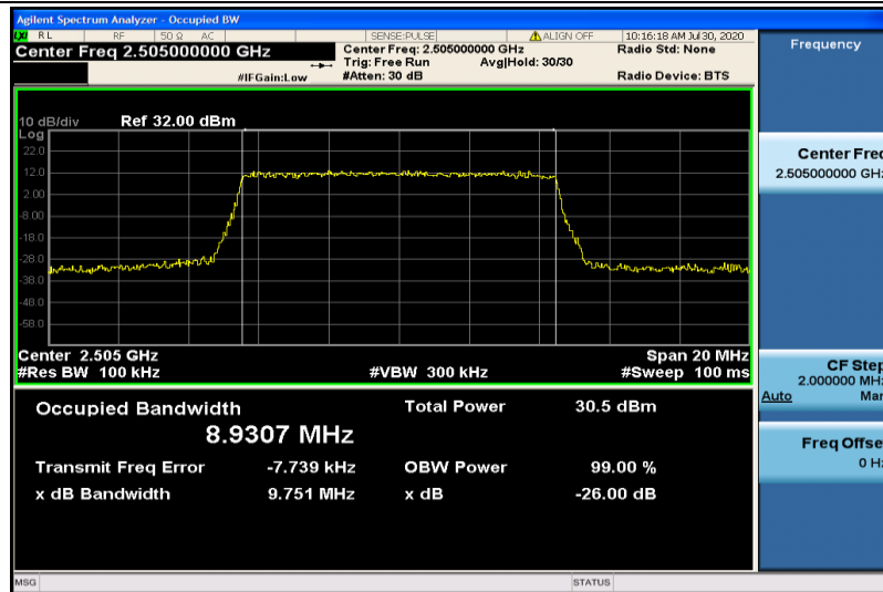
Band7-10MHz-QPSK-20800-50RB#0-8.9307
