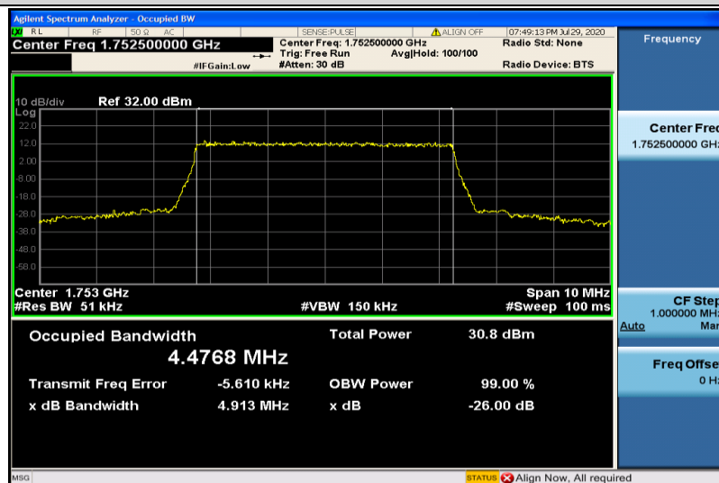
Band4-5MHz-QPSK-20375-25RB#0-4.4768
