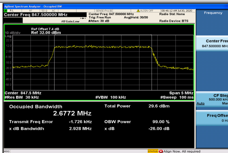
Band5-3MHz-16QAM-20635-15RB#0-2.6772
