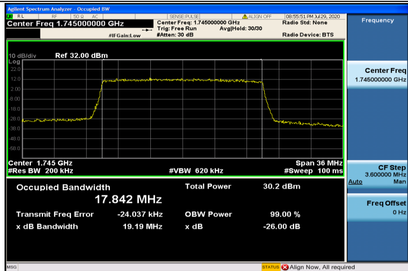
Band4-20MHz-16QAM-20300-100RB#0-17.842
