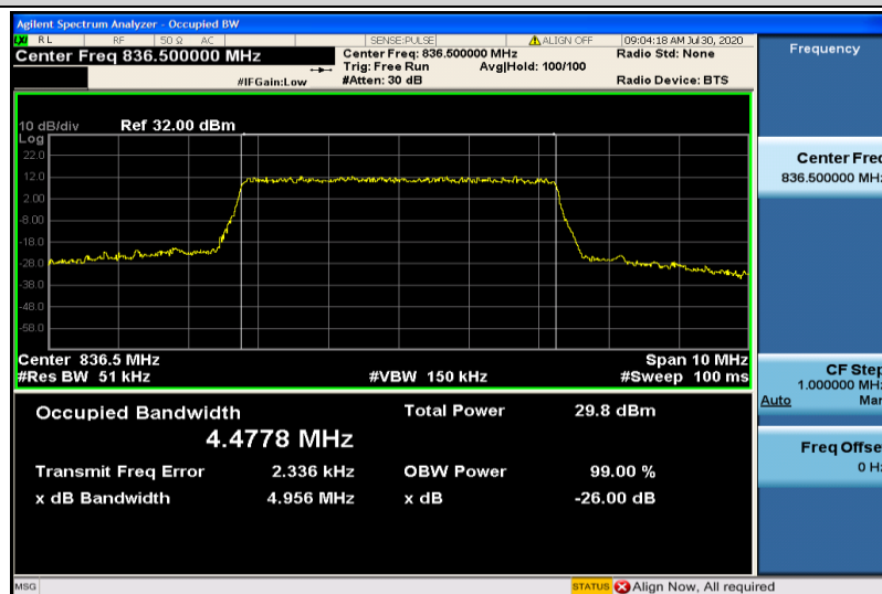
Band5-5MHz-16QAM-20525-25RB#0-4.4778
