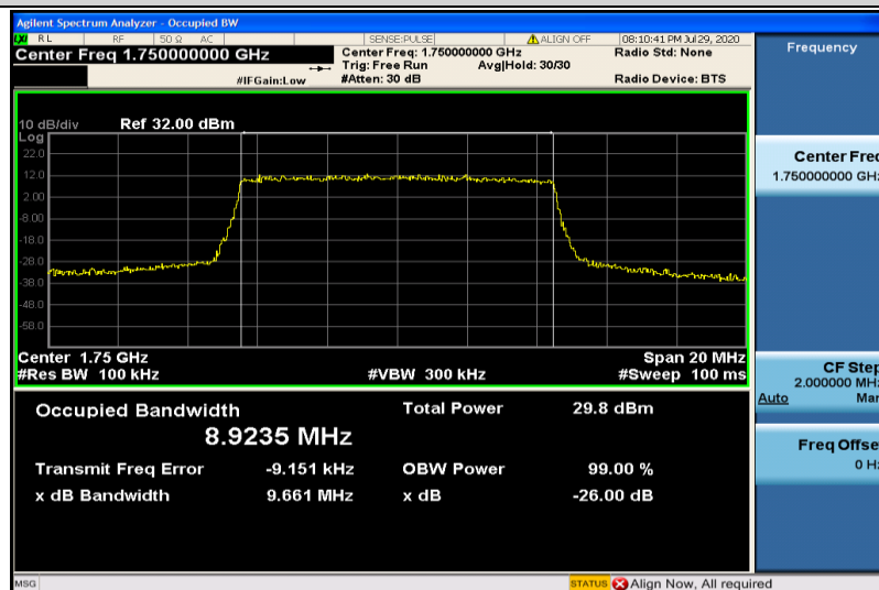
Band4-10MHz-16QAM-20350-50RB#0-8.9235
