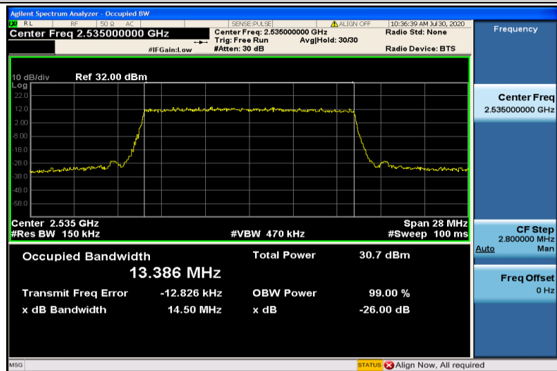
Band7-15MHz-QPSK-21100-75RB#0-13.386
