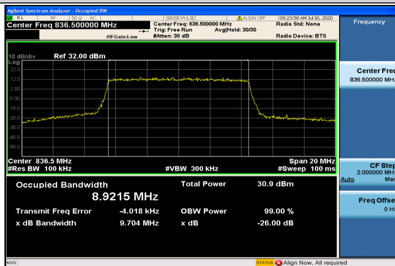
Band5-10MHz-QPSK-20525-50RB#0-8.9215
