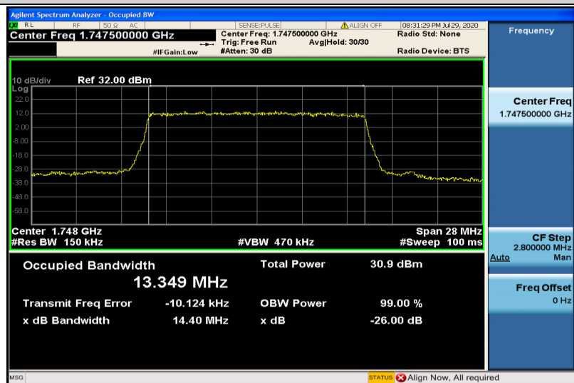
Band4-15MHz-QPSK-20325-75RB#0-13.349
