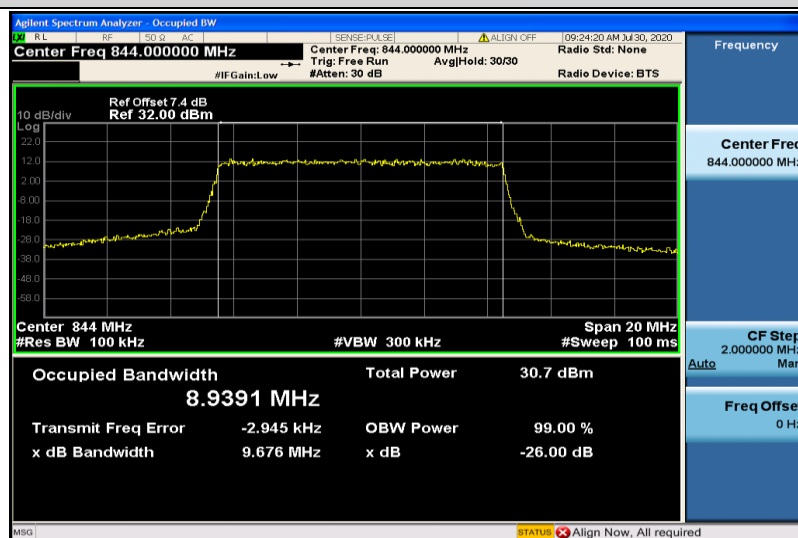
Band5-10MHz-QPSK-20600-50RB#0-8.9391
