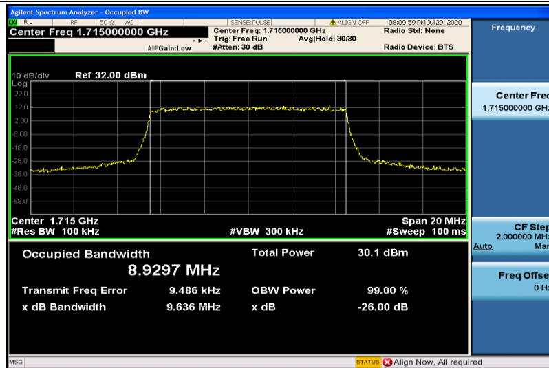
Band4-10MHz-16QAM-20000-50RB#0-8.9297
