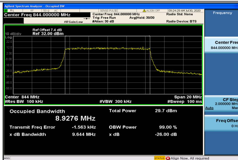
Band5-10MHz-16QAM-20600-50RB#0-8.9276
