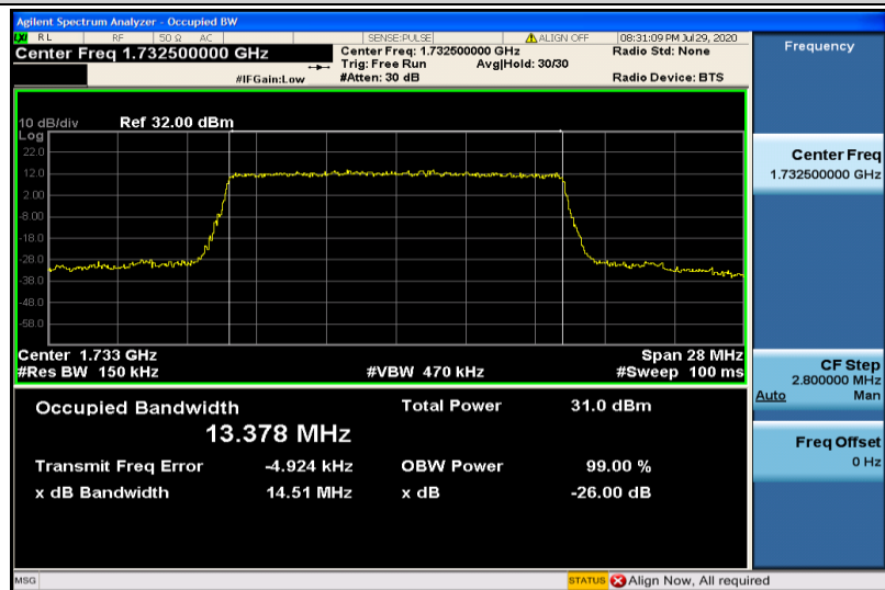
Band4-15MHz-QPSK-20175-75RB#0-13.378
