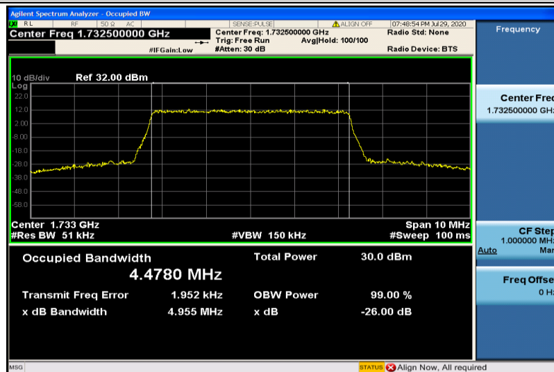
Band4-5MHz-16QAM-20175-25RB#0-4.4780
