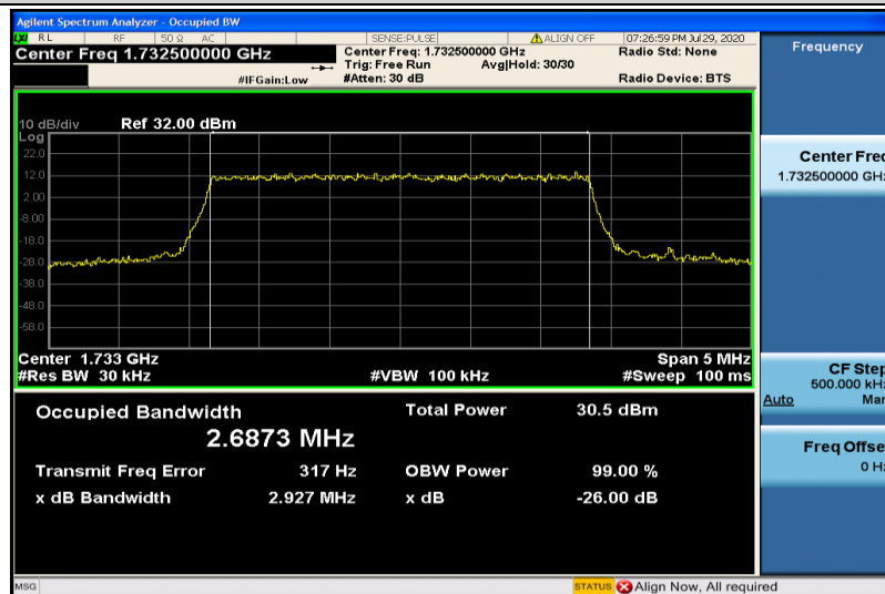
Band4-3MHz-QPSK-20175-15RB#0-2.6873
