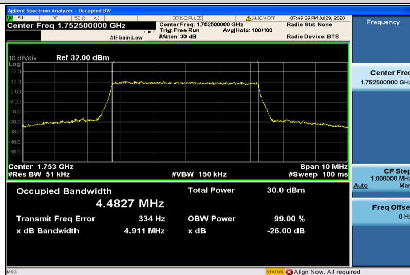
Band4-5MHz-16QAM-20375-25RB#0-4.4827
