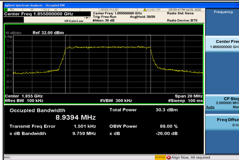
Band2-10MHz-QPSK-18650-50RB#0-8.9394
