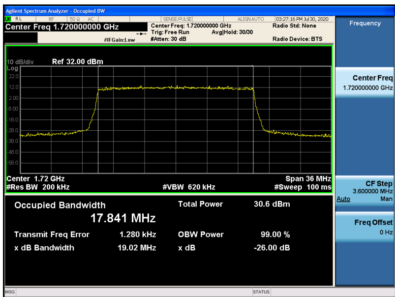
Band4-20MHz-QPSK-20050-100RB#0-17.841
