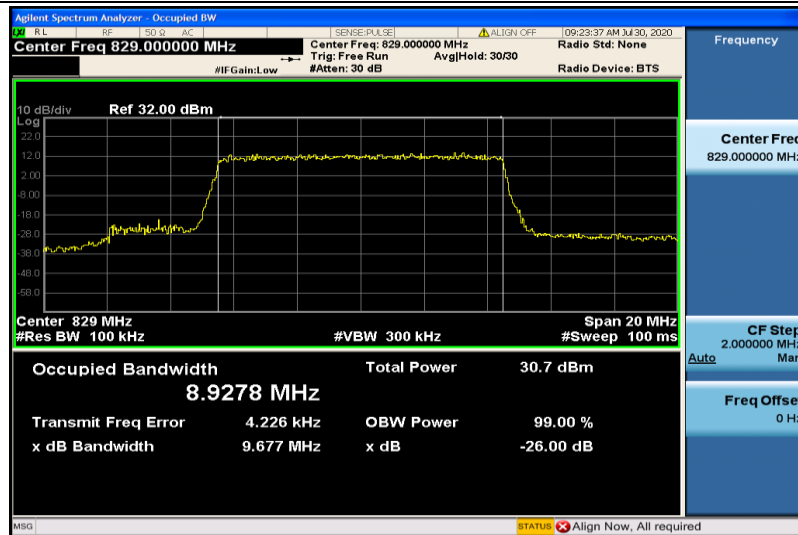
Band5-10MHz-QPSK-20450-50RB#0-8.9278
