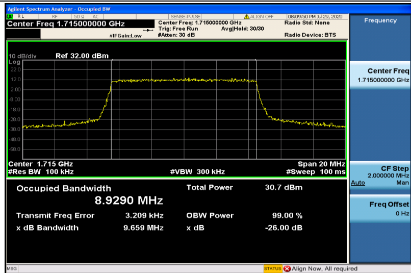
Band4-10MHz-QPSK-20000-50RB#0-8.9290
