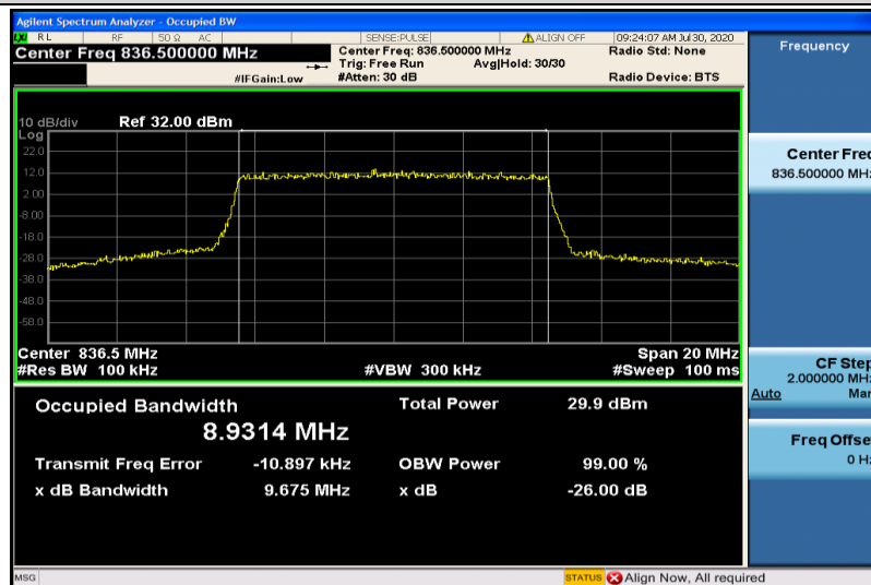
Band5-10MHz-16QAM-20525-50RB#0-8.9314
