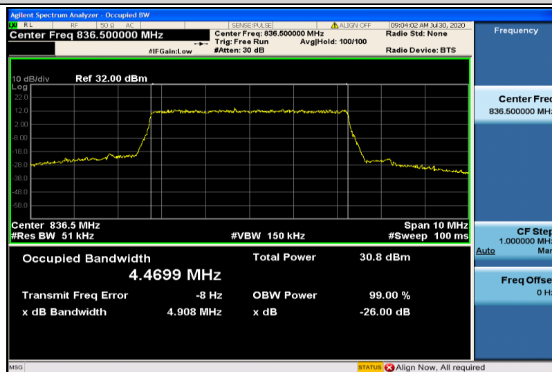
Band5-5MHz-QPSK-20525-25RB#0-4.4699
