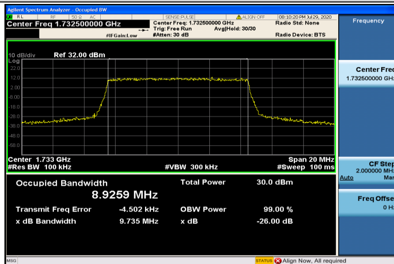
Band4-10MHz-16QAM-20175-50RB#0-8.9259
