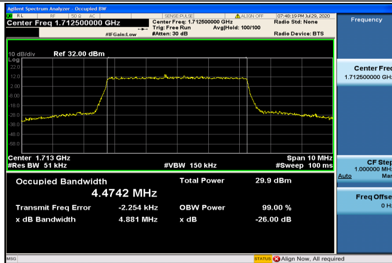
Band4-5MHz-16QAM-19975-25RB#0-4.4742
