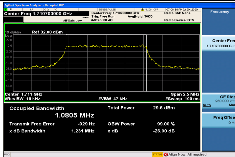
Band4-1.4MHz-QPSK-19957-6RB#0-1.0805
