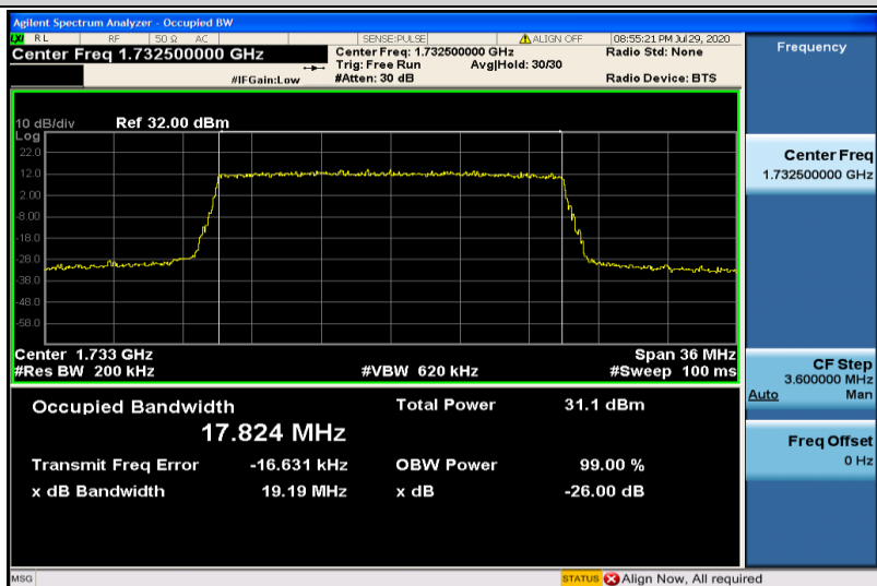
Band4-20MHz-QPSK-20175-100RB#0-17.824
