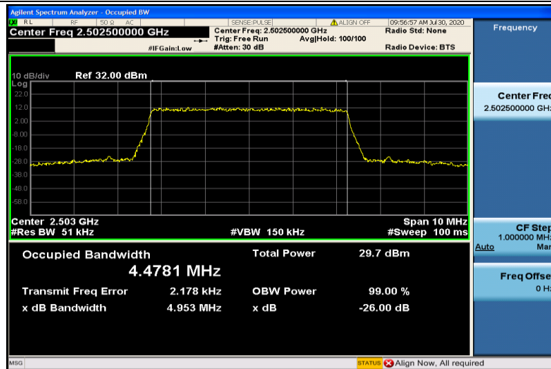
Band7-5MHz-16QAM-20775-25RB#0-4.4781
