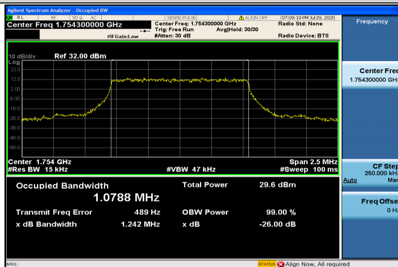
Band4-1.4MHz-QPSK-20393-6RB#0-1.0788
