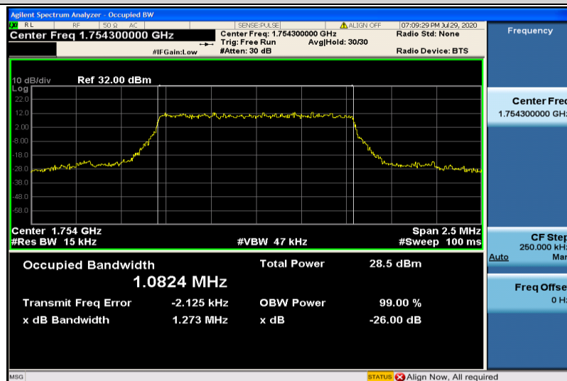
Band4-1.4MHz-16QAM-20393-6RB#0-1.0824
