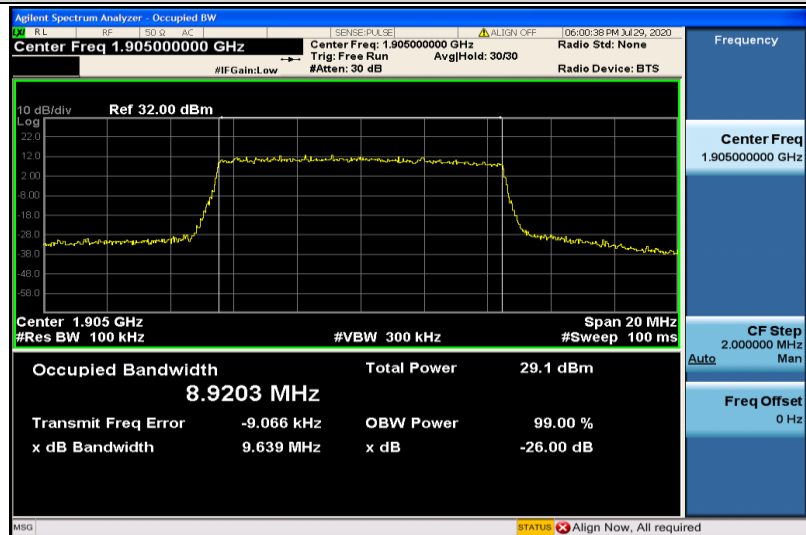
Band2-10MHz-16QAM-19150-50RB#0-8.9203
