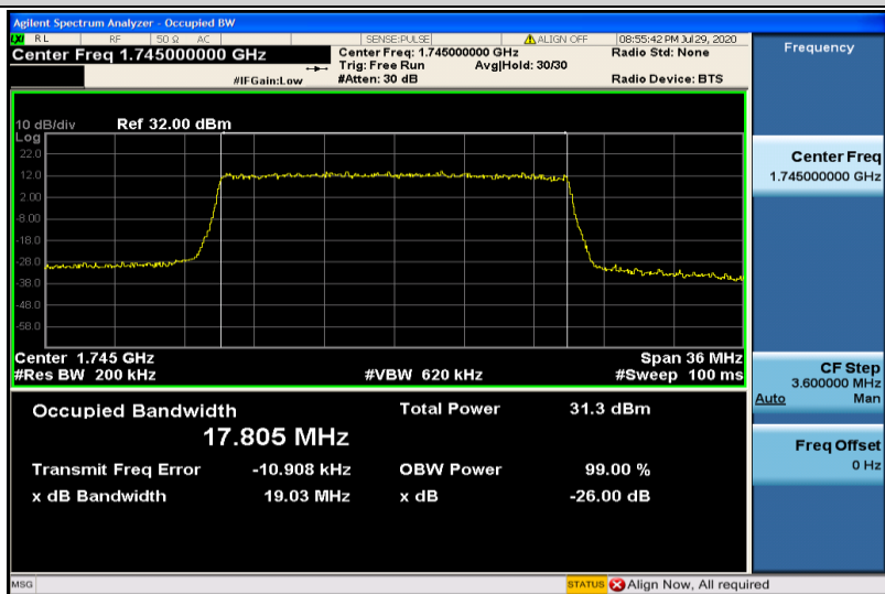
Band4-20MHz-QPSK-20300-100RB#0-17.805
