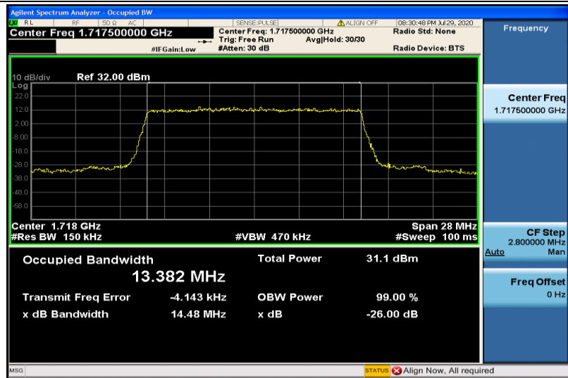
Band4-15MHz-QPSK-20025-75RB#0-13.382
