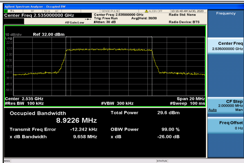
Band7-10MHz-16QAM-21100-50RB#0-8.9226
