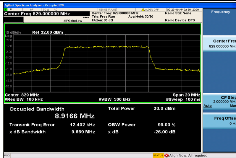
Band5-10MHz-16QAM-20450-50RB#0-8.9166
