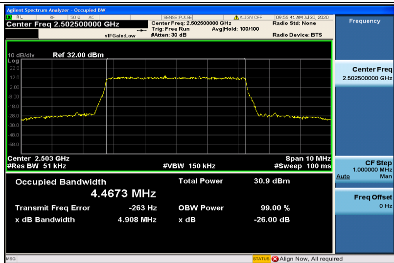
Band7-5MHz-QPSK-20775-25RB#0-4.4673
