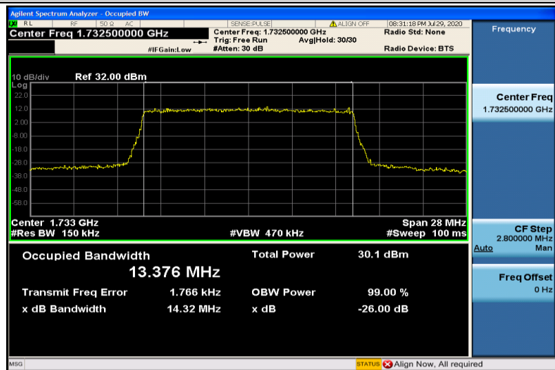
Band4-15MHz-16QAM-20175-75RB#0-13.376
