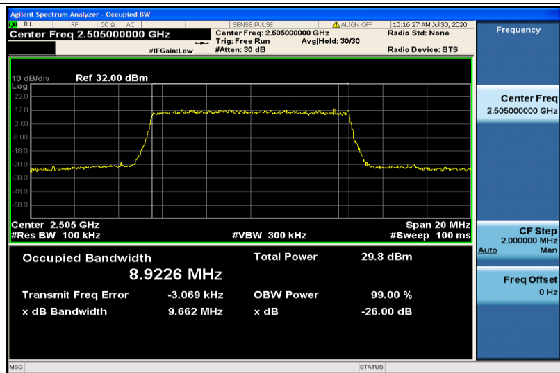
Band7-10MHz-16QAM-20800-50RB#0-8.9226
