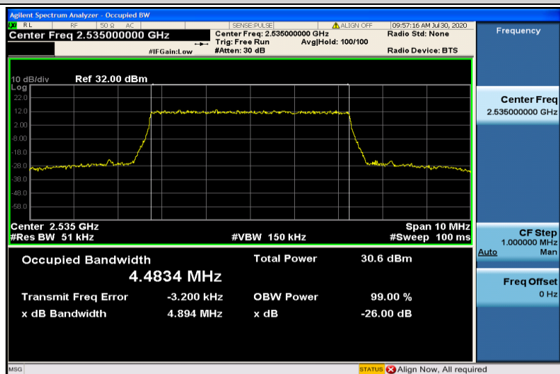
Band7-5MHz-QPSK-21100-25RB#0-4.4834
