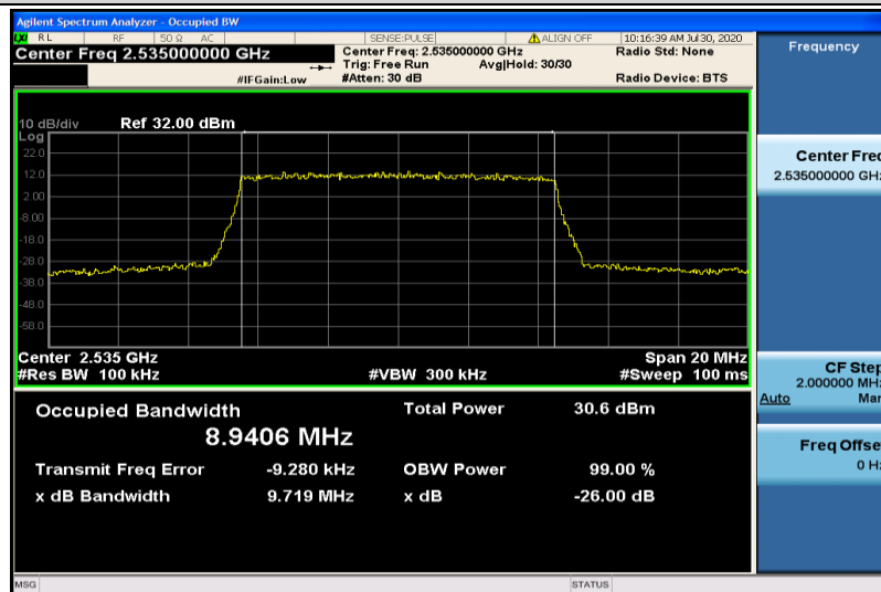
Band7-10MHz-QPSK-21100-50RB#0-8.9406
