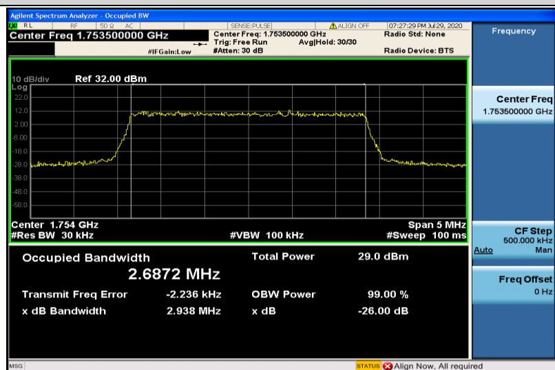
Band4-3MHz-16QAM-20385-15RB#0-2.6872
