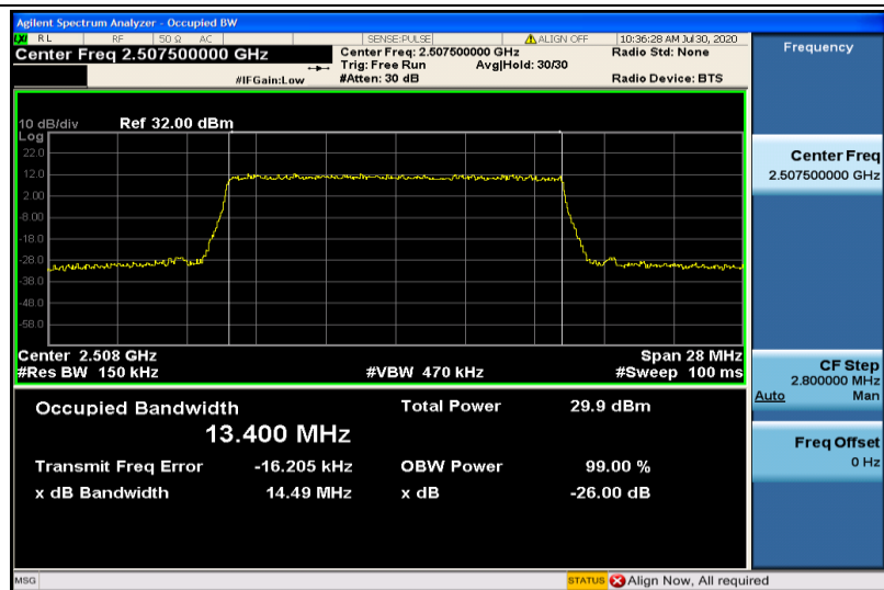
Band7-15MHz-16QAM-20825-75RB#0-13.400
