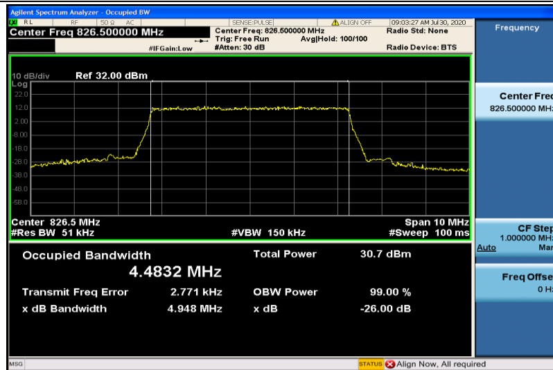
Band5-5MHz-QPSK-20425-25RB#0-4.4832
