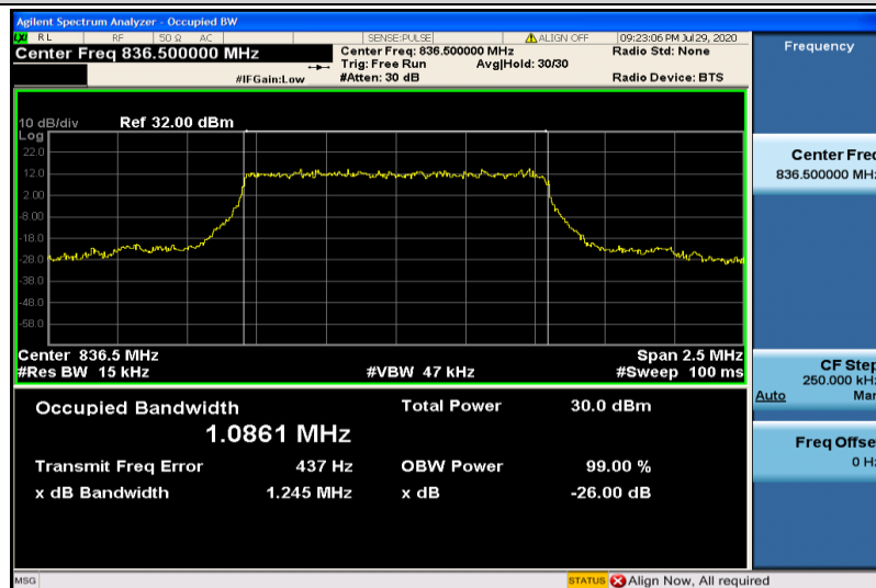
Band5-1.4MHz-QPSK-20525-6RB#0-1.0861
