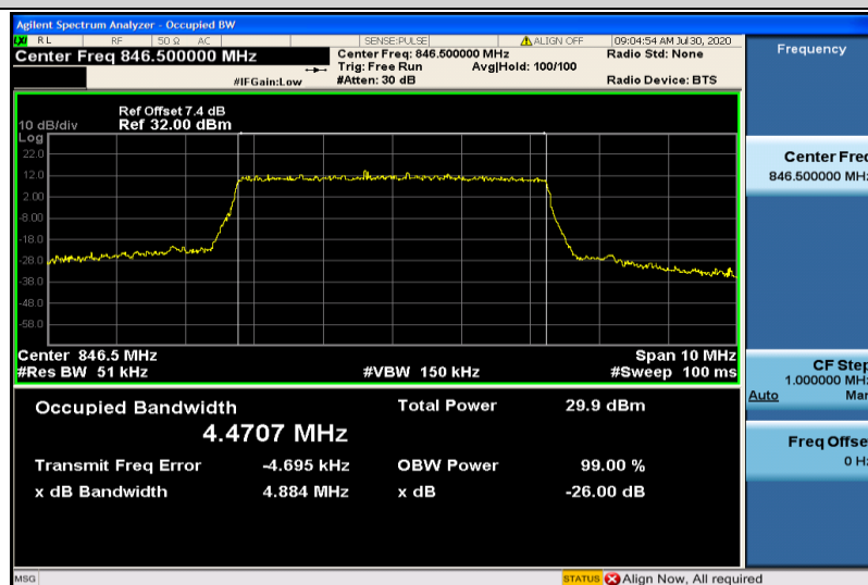
Band5-5MHz-16QAM-20625-25RB#0-4.4707
