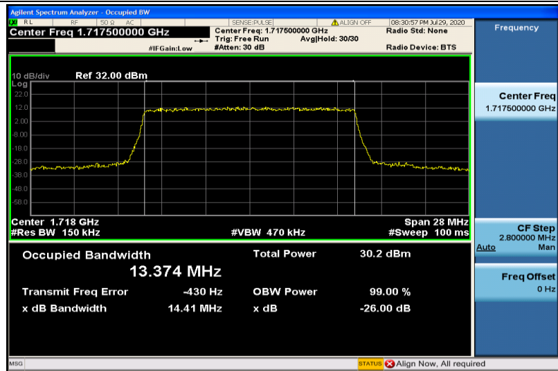
Band4-15MHz-16QAM-20025-75RB#0-13.374
