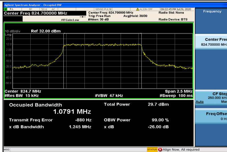
Band5-1.4MHz-QPSK-20407-6RB#0-1.0791
