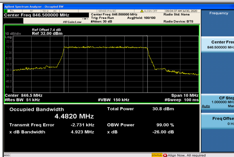
Band5-5MHz-QPSK-20625-25RB#0-4.4820
