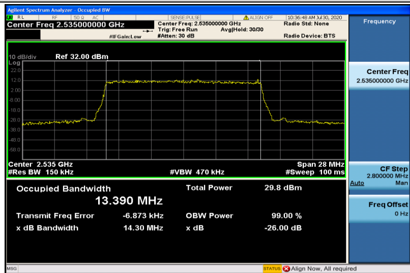
Band7-15MHz-16QAM-21100-75RB#0-13.390
