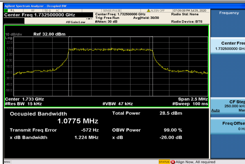
Band4-1.4MHz-16QAM-20175-6RB#0-1.0775
