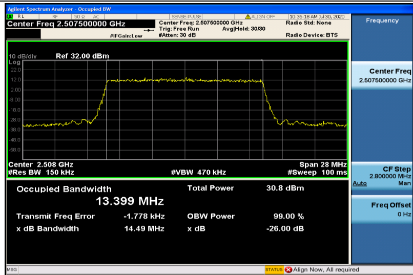
Band7-15MHz-QPSK-20825-75RB#0-13.399
