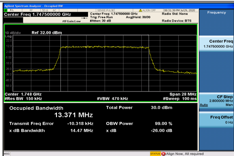
Band4-15MHz-16QAM-20325-75RB#0-13.371
