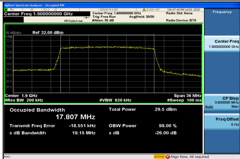
Band2-20MHz-16QAM-19100-100RB#0-17.807
