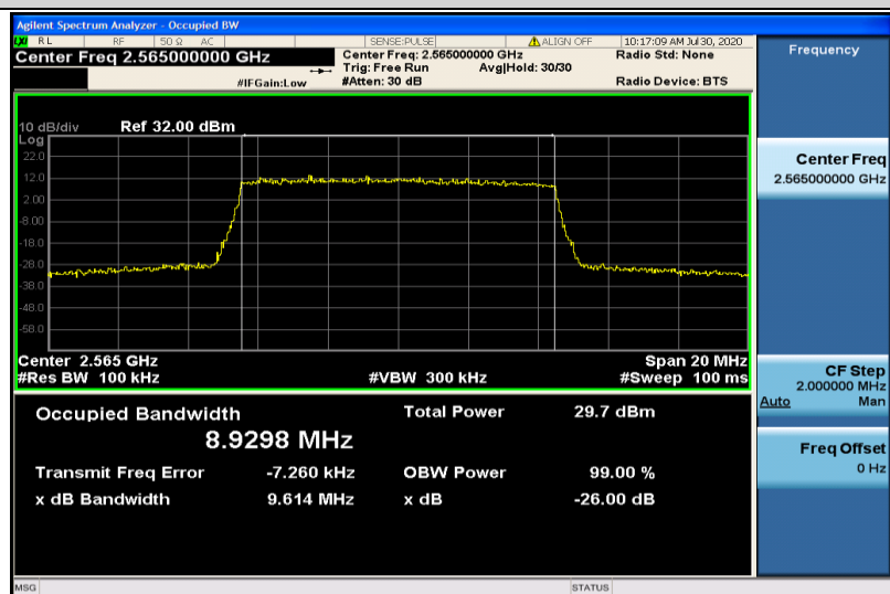
Band7-10MHz-16QAM-21400-50RB#0-8.9298
