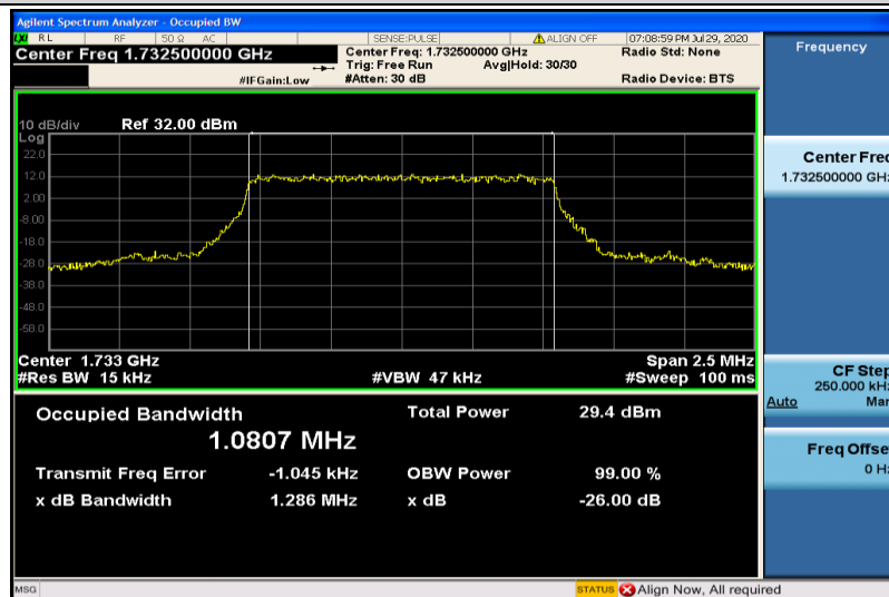
Band4-1.4MHz-QPSK-20175-6RB#0-1.0807
