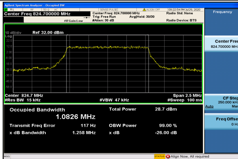
Band5-1.4MHz-16QAM-20407-6RB#0-1.0826
