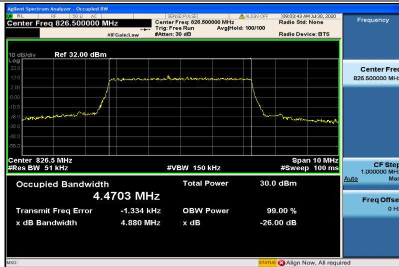
Band5-5MHz-16QAM-20425-25RB#0-4.4703
