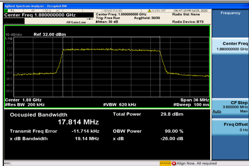
Band2-20MHz-16QAM-18900-100RB#0-17.814
