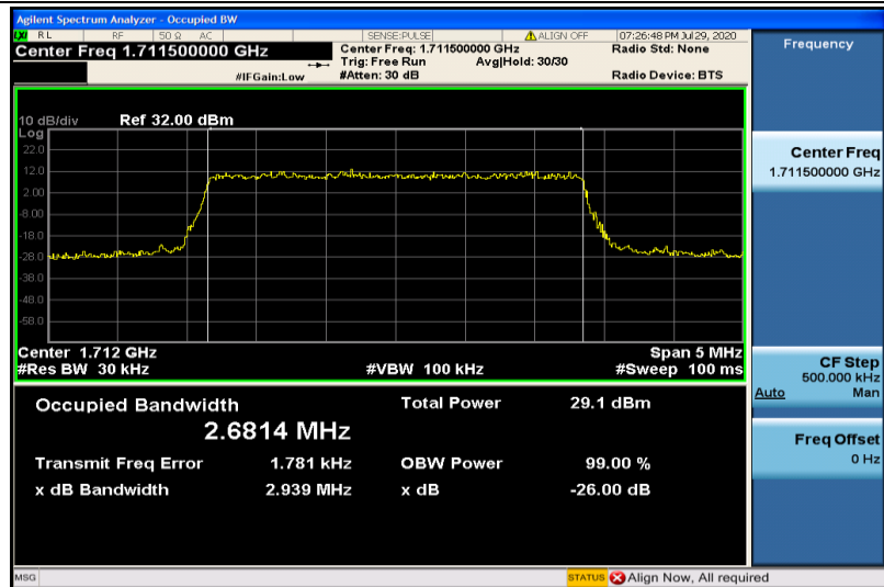
Band4-3MHz-16QAM-19965-15RB#0-2.6814
