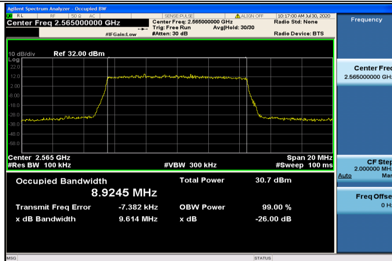
Band7-10MHz-QPSK-21400-50RB#0-8.9245
