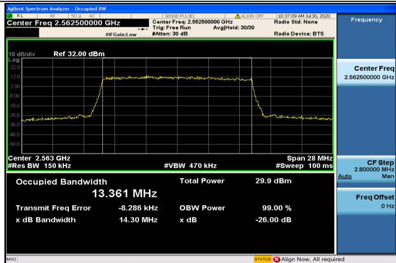
Band7-15MHz-16QAM-21375-75RB#0-13.361
