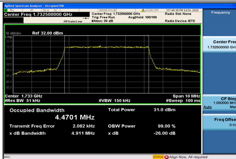
Band4-5MHz-QPSK-20175-25RB#0-4.4701
