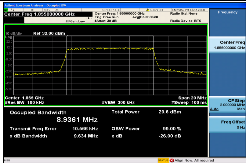
Band2-10MHz-16QAM-18650-50RB#0-8.9361
