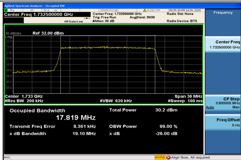
Band4-20MHz-16QAM-20175-100RB#0-17.819
