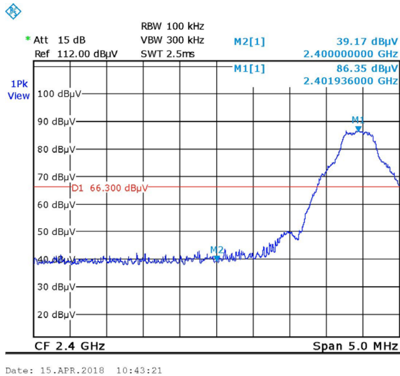
Figure 22 —Lower Band Edge
