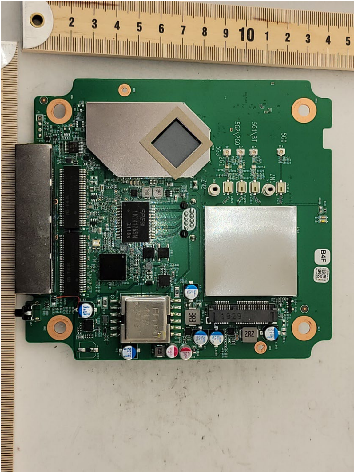
Main PCB Top EMI can(s) installed
