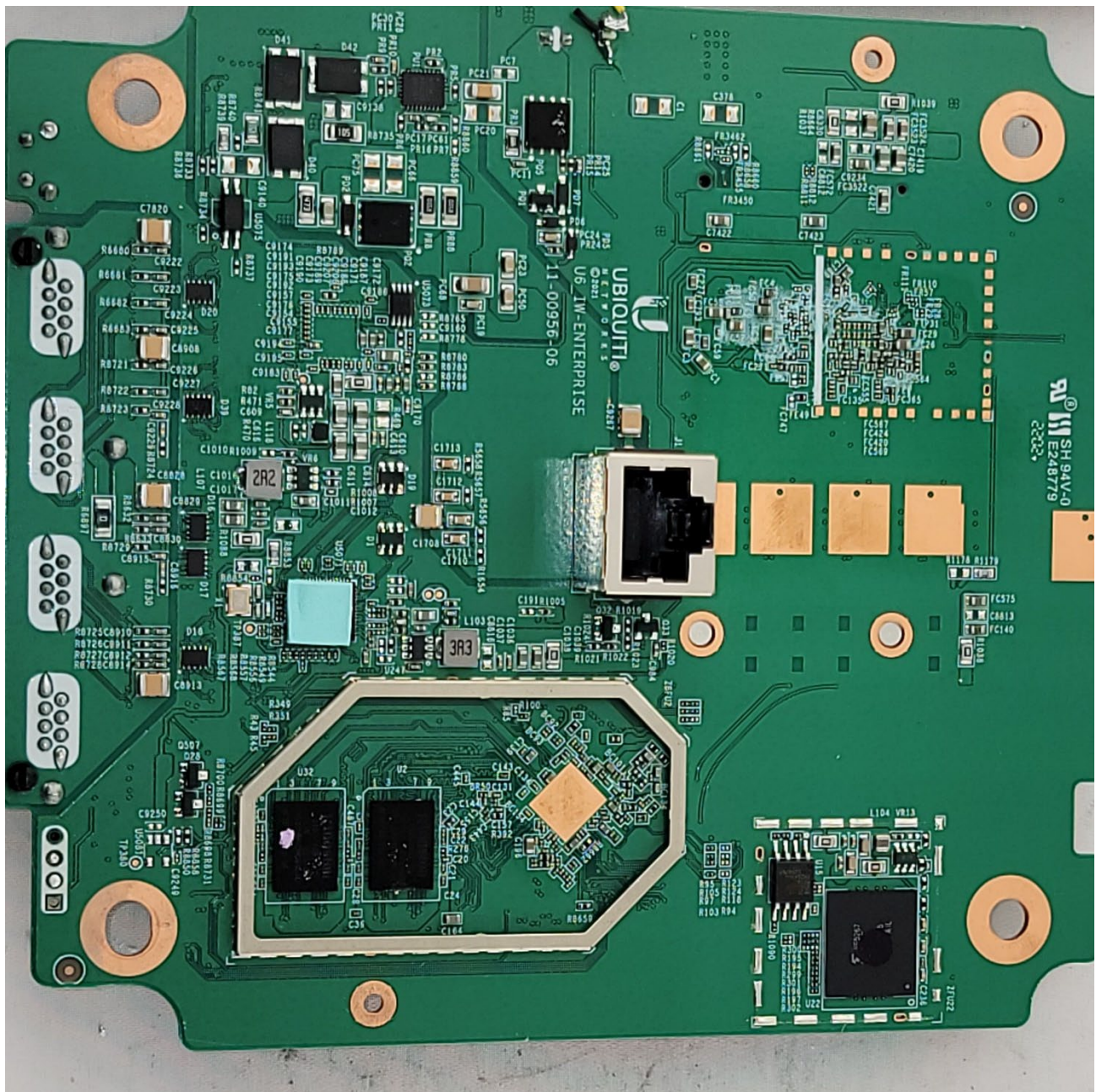
Main PCB Bottom EMI can(s) removed
