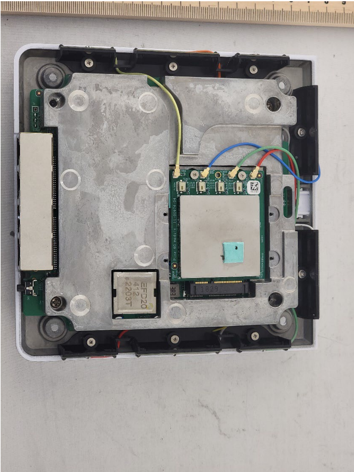
DUT Faceplate removed
