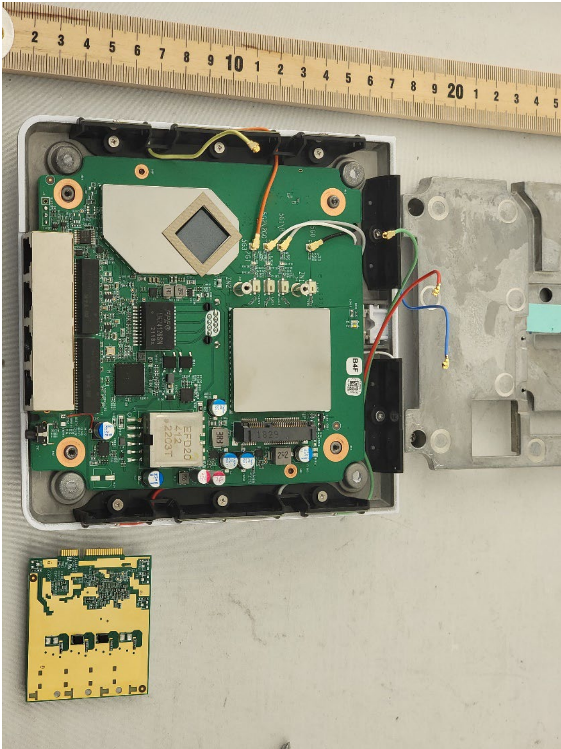
Top Heatsink Removed
