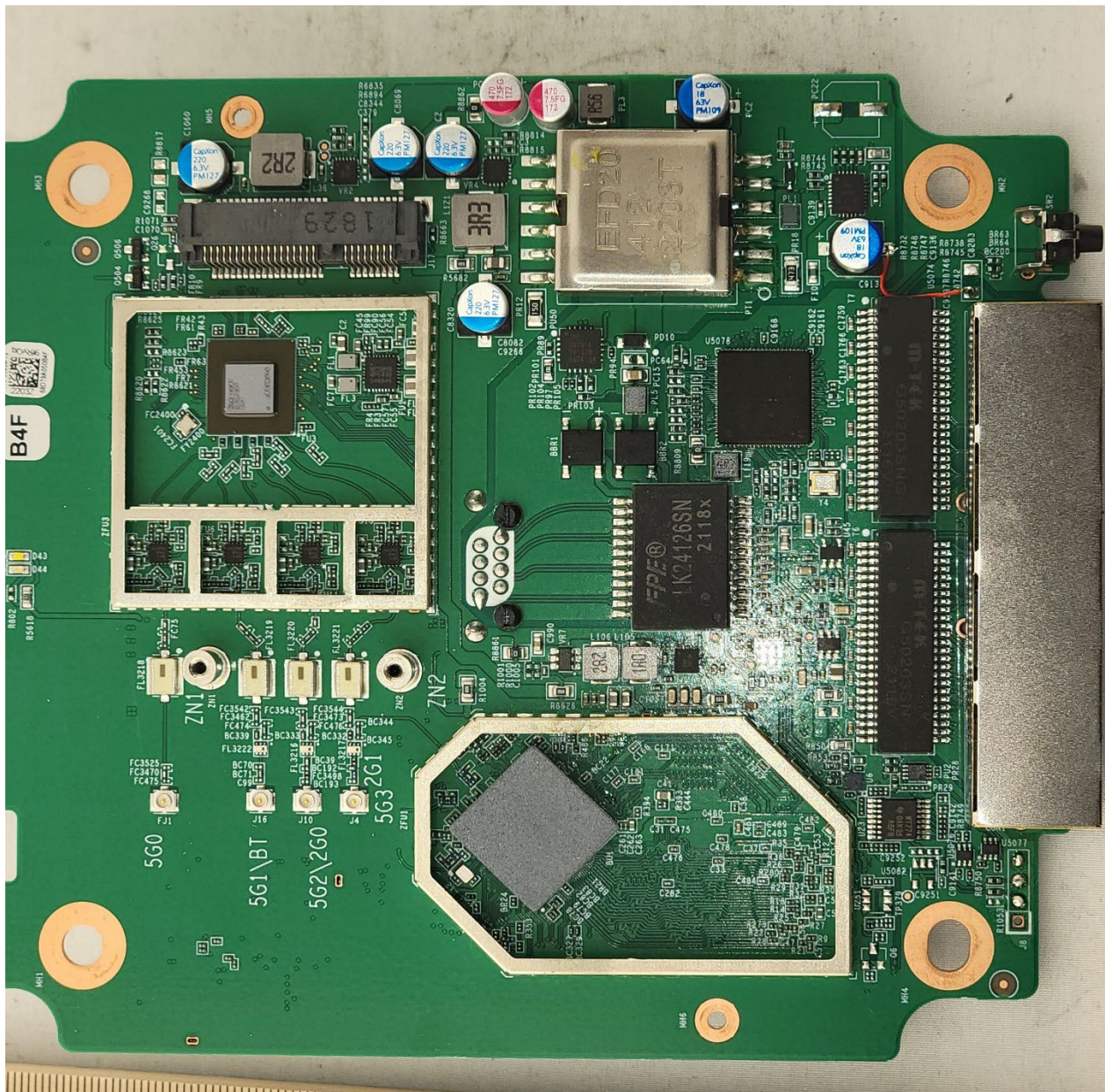
Main PCB Top EMI can(s) removed
