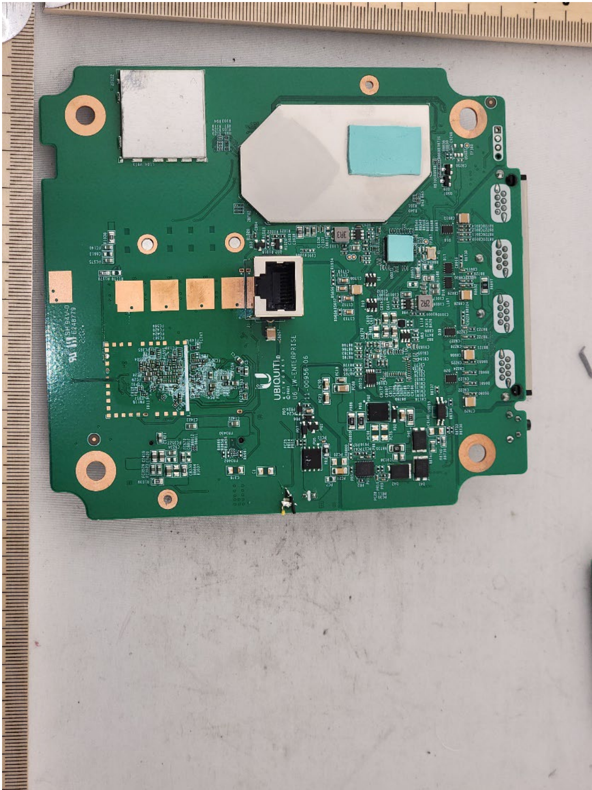
Main PCB Bottom EMI can(s) installed
