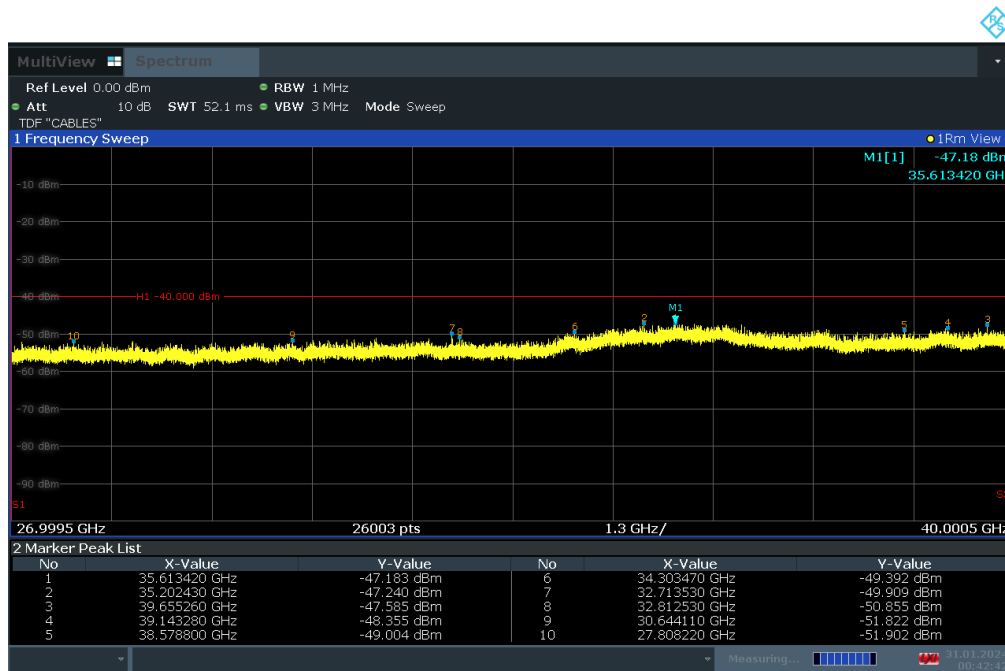
Plot 7-65. Conducted Spurious Plot (LTE Band 48 - 20MHz QPSK - Mid Channel)
