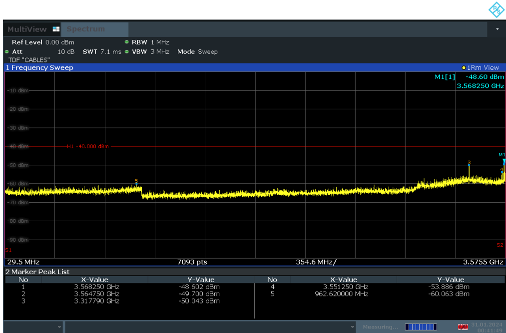
Plot 7-62. Conducted Spurious Plot (LTE Band 48 - 20MHz QPSK - Mid Channel)
