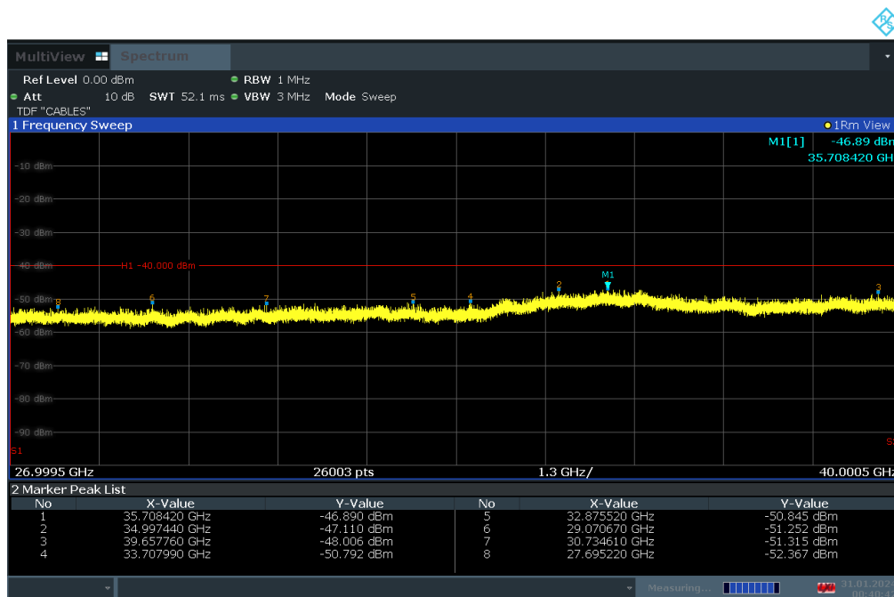
Plot 7-61. Conducted Spurious Plot (LTE Band 48 - 20MHz QPSK - Low Channel)
