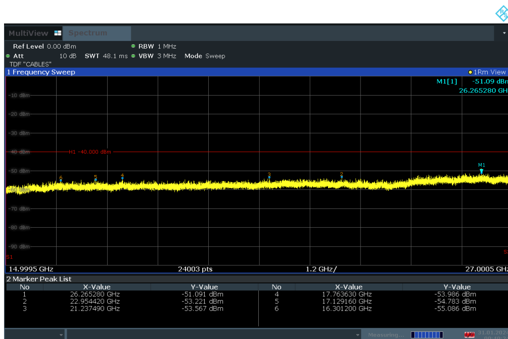
Plot 7-60. Conducted Spurious Plot (LTE Band 48 - 20MHz QPSK - Low Channel)
