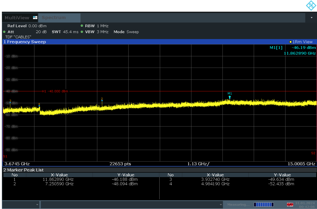
Plot 7-63. Conducted Spurious Plot (LTE Band 48 - 20MHz QPSK - Mid Channel)
