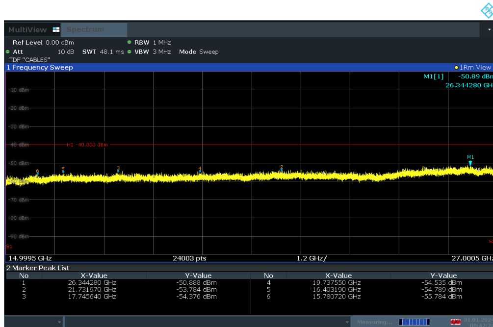
Plot 7-64. Conducted Spurious Plot (LTE Band 48 - 20MHz QPSK - Mid Channel)
