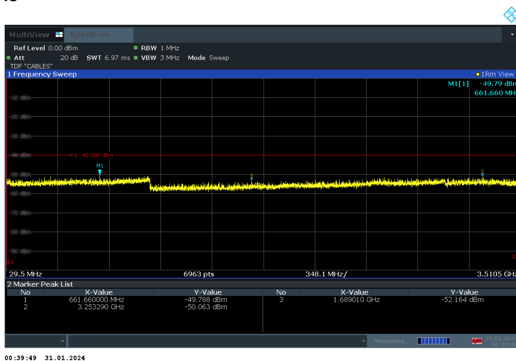
Plot 7-58. Conducted Spurious Plot (LTE Band 48 - 20MHz QPSK - Low Channel)
