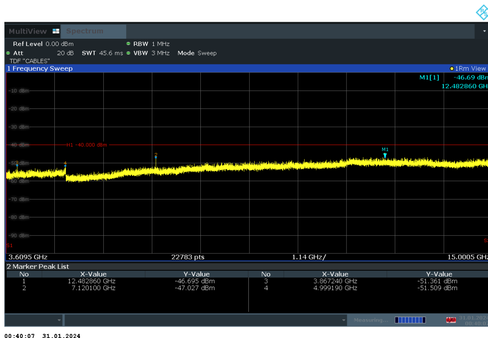
Plot 7-59. Conducted Spurious Plot (LTE Band 48 - 20MHz QPSK - Low Channel)
