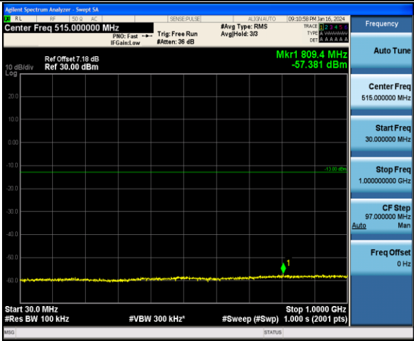
Band4_10MHz_QPSK_20175_1RB#0_30~1000_30~1000
