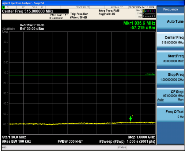
Band4_15MHz_16QAM_2025_1RB#0_30~1000_30~1000
