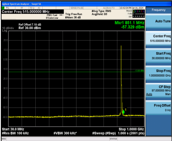
Band5_5MHz_QPSK_20525_1RB#0_30~1000_30~1000
