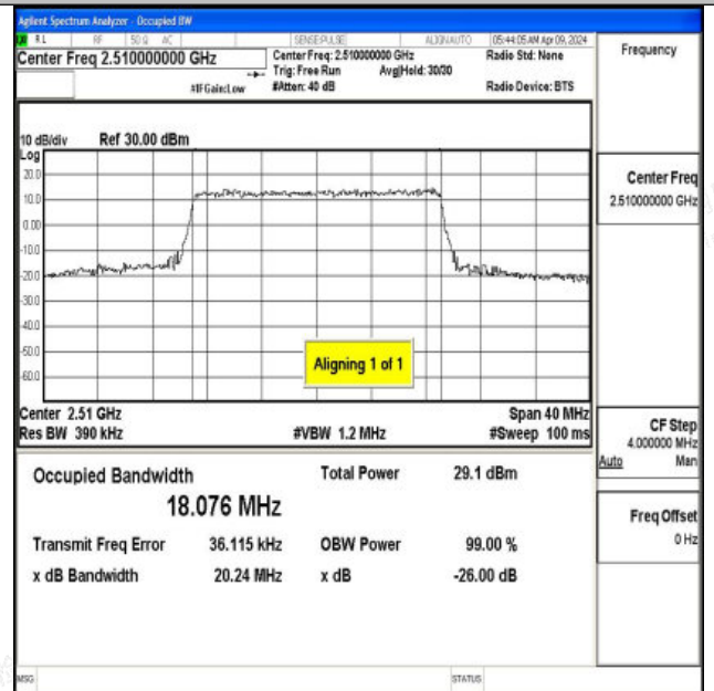
Band7-20MHz-16QAM-20850-100RB#0-PASS
