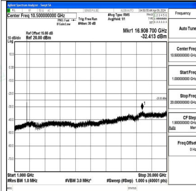
Band7_5MHz_16QAM_21100_1RB#0_1000~20000_1000~20000
