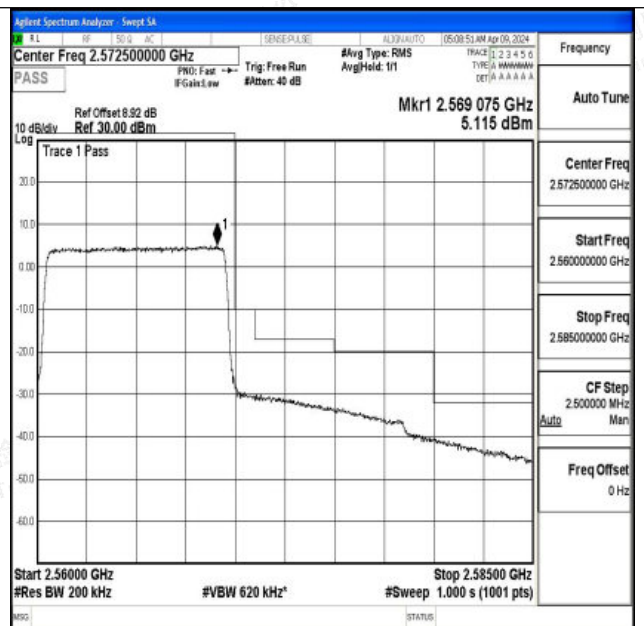
Band7_10MHz_16QAM_21400_50RB#0
