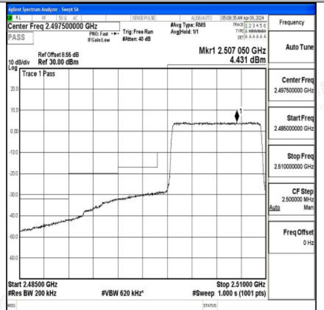
Band7_10MHz_16QAM_20800_50RB#0
