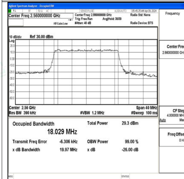
Band7-20MHz-QPSK-21350-100RB#0-PASS
