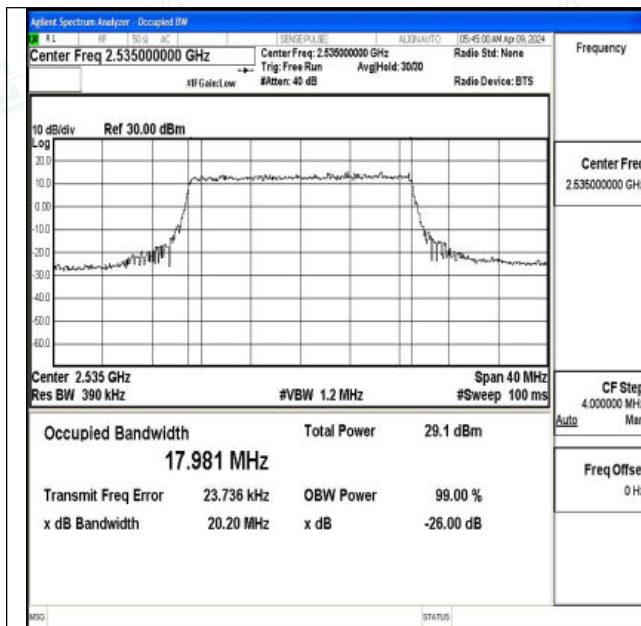
Band7-20MHz-QPSK-21100-100RB#0-PASS
