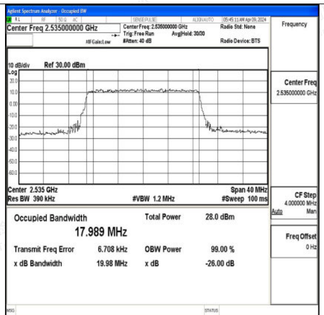
Band7-20MHz-16QAM-21100-100RB#0-PASS
