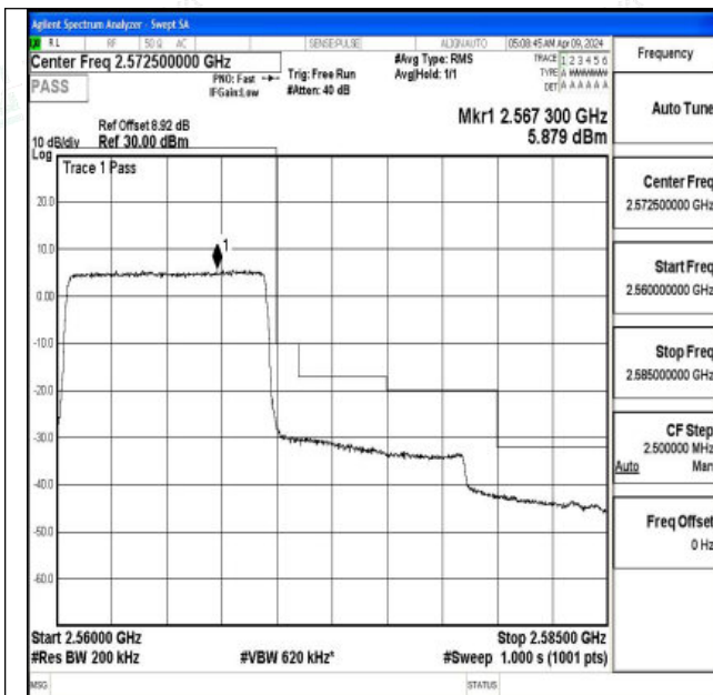
Band7_10MHz_QPSK_21400_50RB#0
