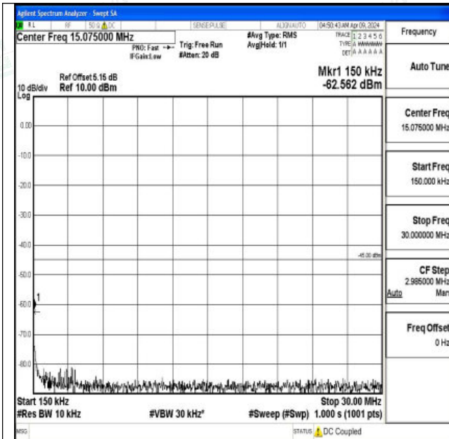
Band7_5MHz_16QAM_21100_1RB#0_0.15~30_0.15~30
