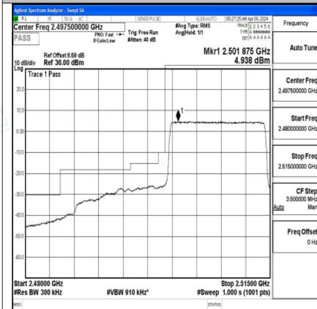
Band7_15MHz_QPSK_20825_75RB#0
