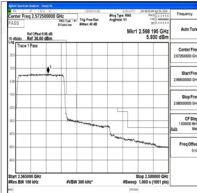
Band7_5MHz_QPSK_21425_25RB#0
