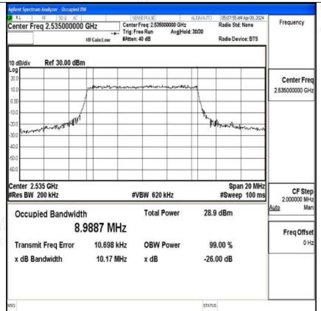
Band7-10MHz-16QAM-21100-50RB#0-PASS
