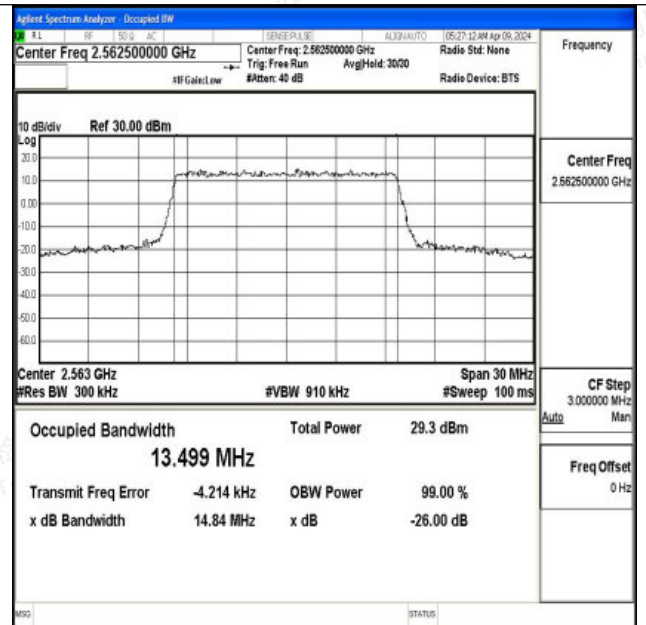
Band7-15MHz-16QAM-21375-75RB#0-PASS
