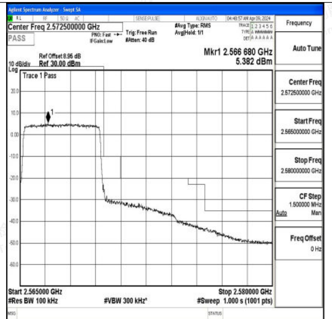
Band7_5MHz_16QAM_21425_25RB#0
