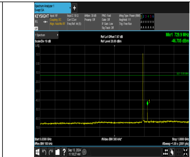
Band12_1.4MHz_16QAM_23017_6RB#0_30~1000_30~1000
