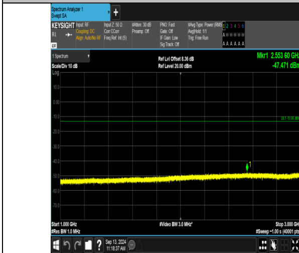
Band12_1.4MHz_16QAM_23017_6RB#0_1000~3000_1000~3000
