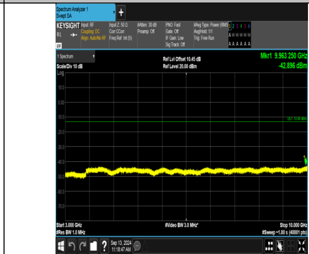
Band12_1.4MHz_16QAM_23017_6RB#0_3000~10000_3000~10000
