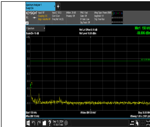
Band12_1.4MHz_16QAM_23017_6RB#0_0.15~30_0.15~30
