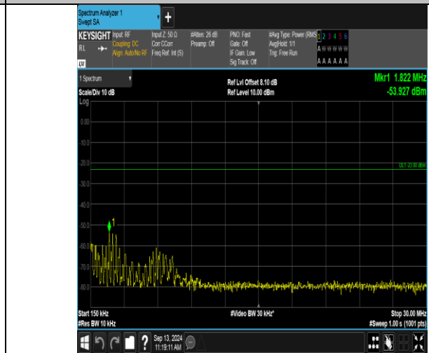
Band12_1.4MHz_QPSK_23095_1RB#0_0.15~30_0.15~30
