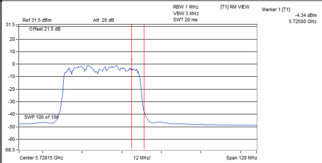
802.11ax (HE40)_Chain 0 / CH142 (U-NII-3 Band)
