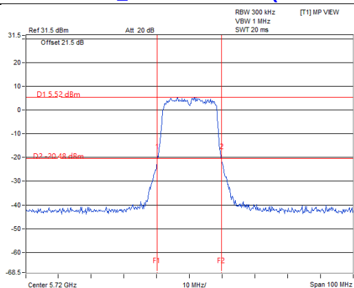
802.11a_Chain 2 / CH144 (U-NII-3 Band)
