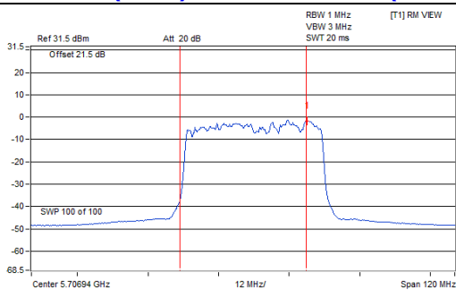
802.11ax (HE40)_Chain 1 / CH142 (U-NII-2C Band)
