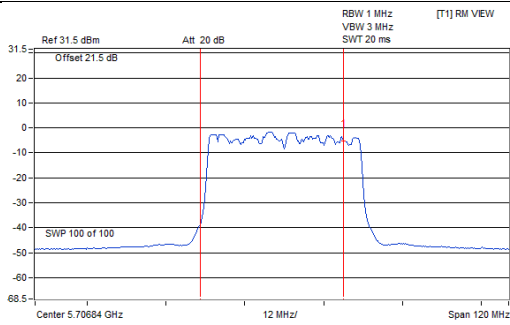
802.11ax (HE40)_Chain 0 / CH142 (U-NII-2C Band)
