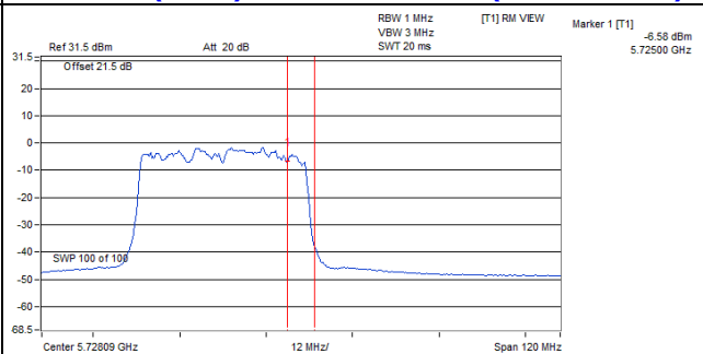
802.11ax (HE40)_Chain 1 / CH142 (U-NII-3 Band)
