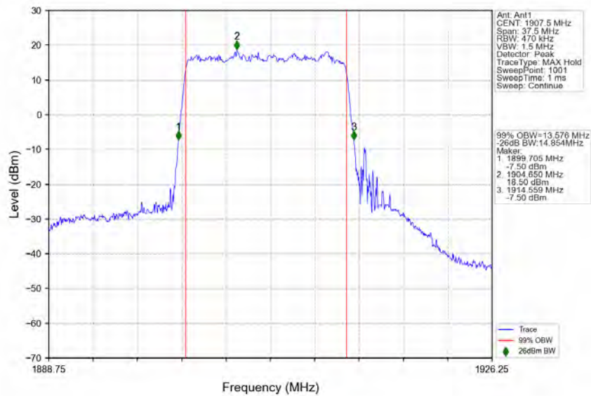
n25_15kHz_SISO_NTNV_15MHz_DFT-s-OFDM_QPSK_1907.5MHz_Outer_Full
