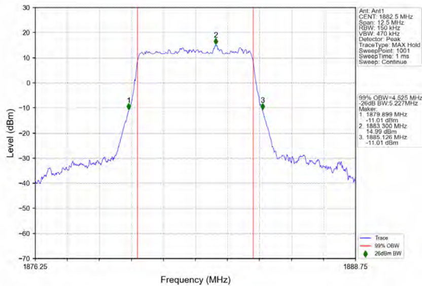
n25_15kHz_SISO_NTNV_5MHz_DFT-s-OFDM_256_QAM_1882.5MHz_Outer_Full
