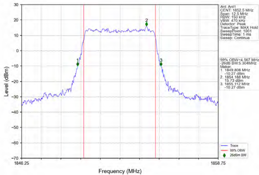
n25_15kHz_SISO_NTNV_5MHz_CP-OFDM_64_QAM_1852.5MHz_Outer_Full
