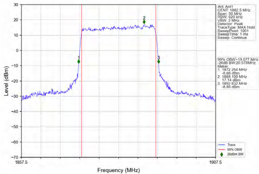
n25_15kHz_SISO_NTNV_20MHz_CP-OFDM_16_QAM_1882.5MHz_Outer_Full
