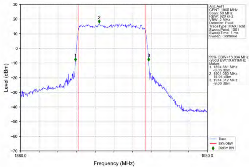
n25_15kHz_SISO_NTNV_20MHz_DFT-s-OFDM_64_QAM_1905MHz_Outer_Full
