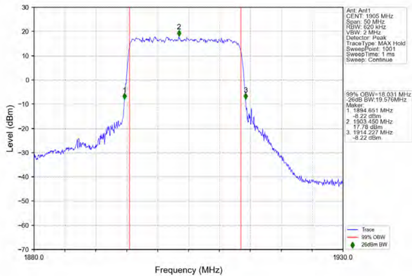
n25_15kHz_SISO_NTNV_20MHz_DFT-s-OFDM_QPSK_1905MHz_Outer_Full
