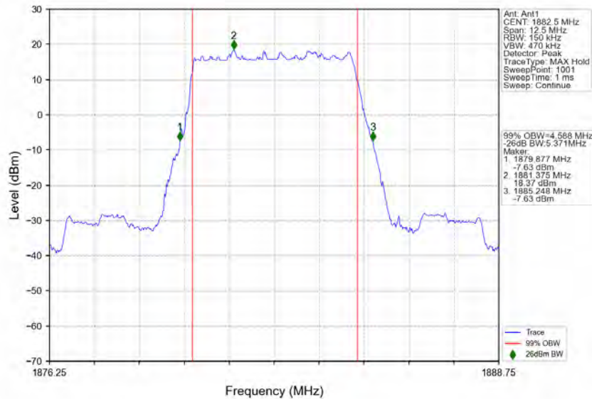
n25_15kHz_SISO_NTNV_5MHz_DFT-s-OFDM PI/2 BPSK_1882.5MHz_Outer_Full
