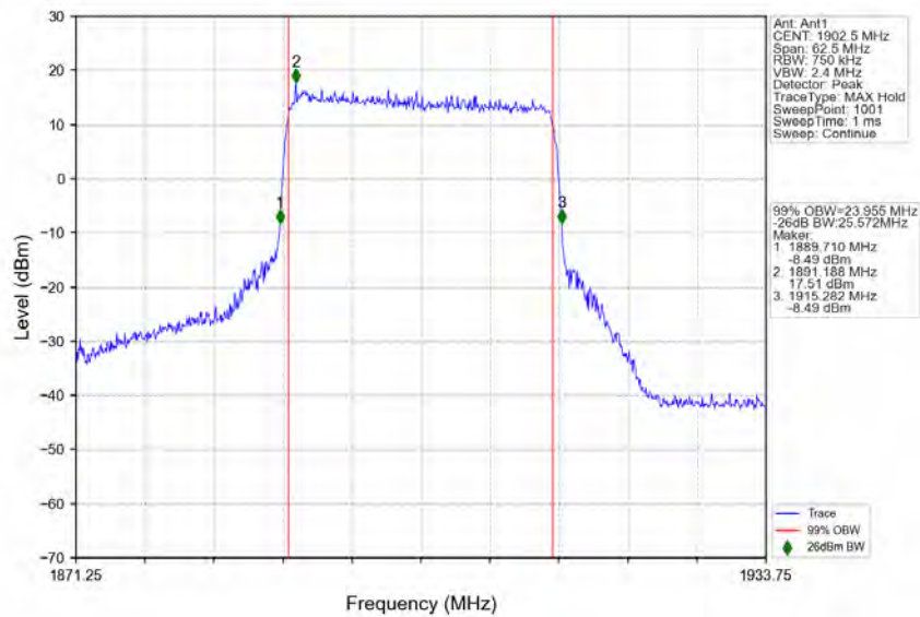
n25_15kHz_SISO_NTNV_25MHz_CP-OFDM_64_QAM_1902.5MHz_Outer_Full
