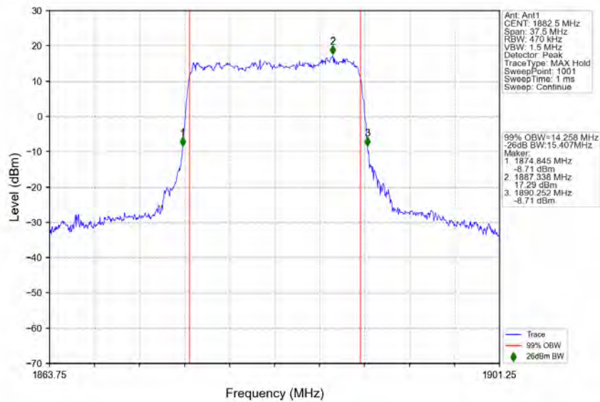
n25_15kHz_SISO_NTNV_15MHz_CP-OFDM_16_QAM_1882.5MHz_Outer_Full
