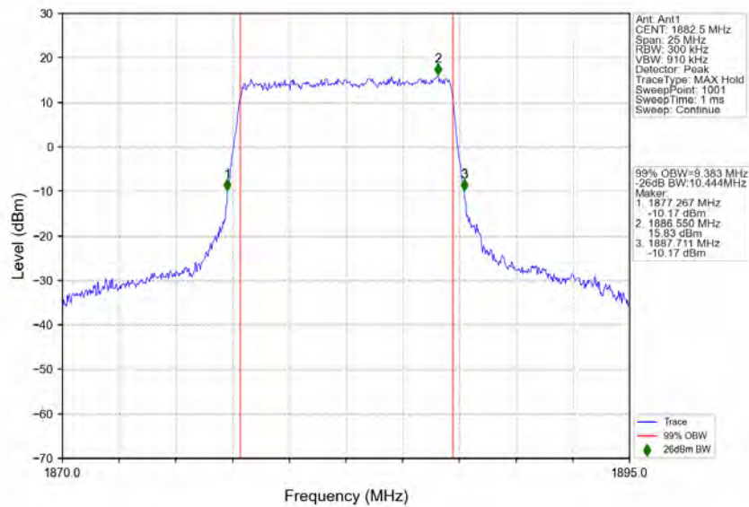
n25_15kHz_SISO_NTNV_10MHz_CP-OFDM_16_QAM_1882.5MHz_Outer_Full
