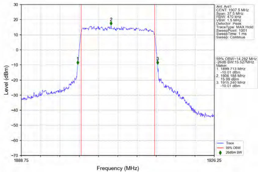
n25_15kHz_SISO_NTNV_15MHz_CP-OFDM_64_QAM_1907.5MHz_Outer_Full
