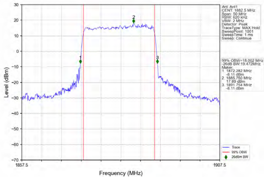
n25_15kHz_SISO_NTNV_20MHz_DFT-s-OFDM_16_QAM_1882.5MHz_Outer_Full
