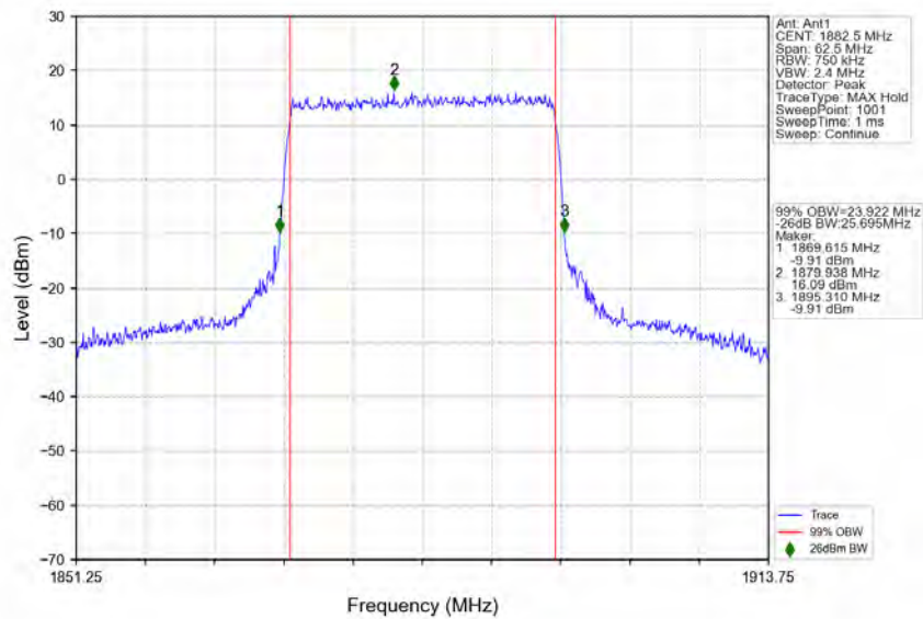
n25_15kHz_SISO_NTNV_25MHz_CP-OFDM_16_QAM_1882.5MHz_Outer_Full
