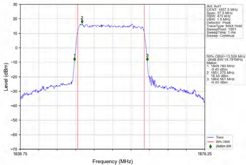
n25_15kHz_SISO_NTNV_15MHz_DFT-s-OFDM_64 QAM_1857.5MHz_Outer_Full
