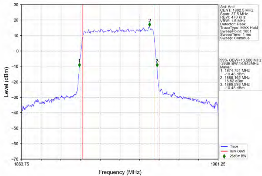
n25_15kHz_SISO_NTNV_15MHz_DFT-s-OFDM_256_QAM_1882.5MHz_Outer_Full
