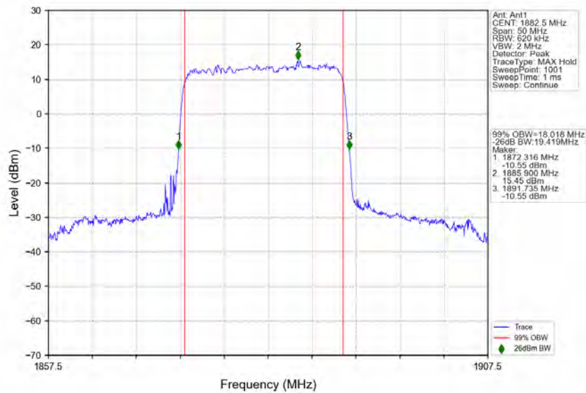
n25_15kHz_SISO_NTNV_20MHz_DFT-s-OFDM_256_QAM_1882.5MHz_Outer_Full
