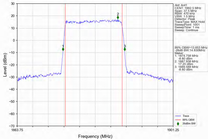
n25_15kHz_SISO_NTNV_15MHz_DFT-s-OFDM_16_QAM_1882.5MHz_Outer_Full
