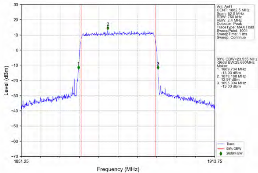
n25_15kHz_SISO_NTNV_25MHz_CP-OFDM_256_QAM_1882.5MHz_Outer_Full
