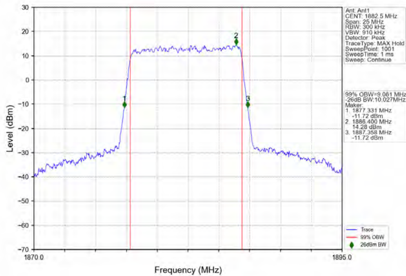
n25_15kHz_SISO_NTNV_10MHz_DFT-s-OFDM_256_QAM_1882.5MHz_Outer_Full
