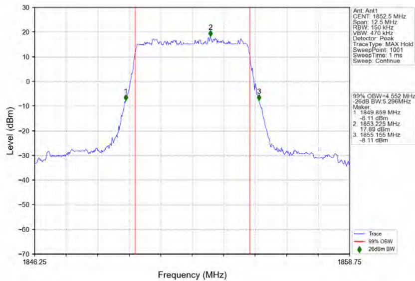
n25_15kHz_SISO_NTNV_5MHz_DFT-s-OFDM_QPSK_1852.5MHz_Outer_Full
