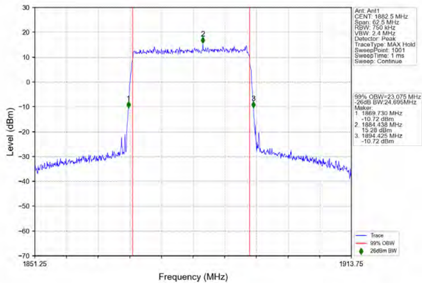
n25_15kHz_SISO_NTNV_25MHz_DFT-s-OFDM_256_QAM_1882.5MHz_Outer_Full
