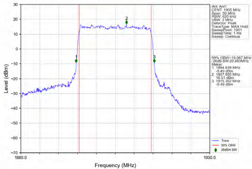
n25_15kHz_SISO_NTNV_20MHz_CP-OFDM_QPSK_1905MHz_Outer_Full
