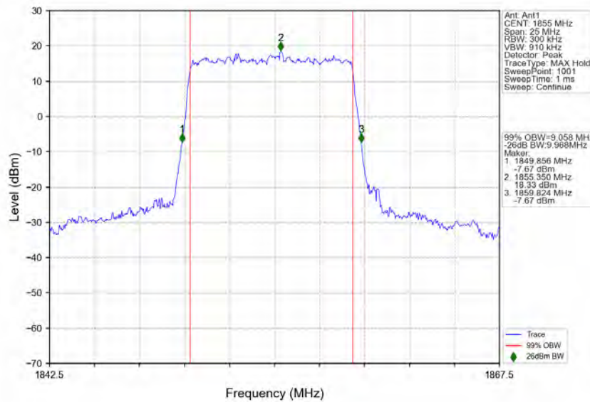
n25_15kHz_SISO_NTNV_10MHz_DFT-s-OFDM_QPSK_1855MHz_Outer_Full
