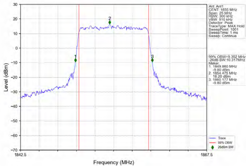
n25_15kHz_SISO_NTNV_10MHz_CP-OFDM_64 QAM_1855MHz_Outer_Full
