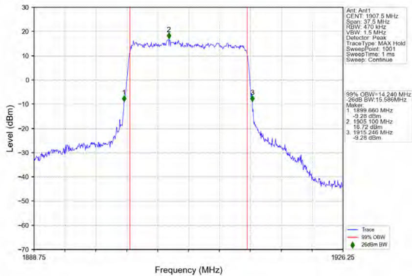
n25_15kHz_SISO_NTNV_15MHz_CP-OFDM_QPSK_1907.5MHz_Outer_Full
