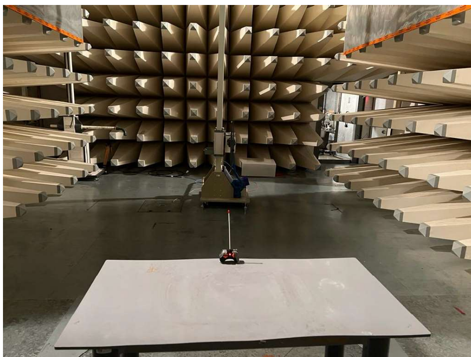
Set-up of Radiation Emission from 200 – 1000MHz
