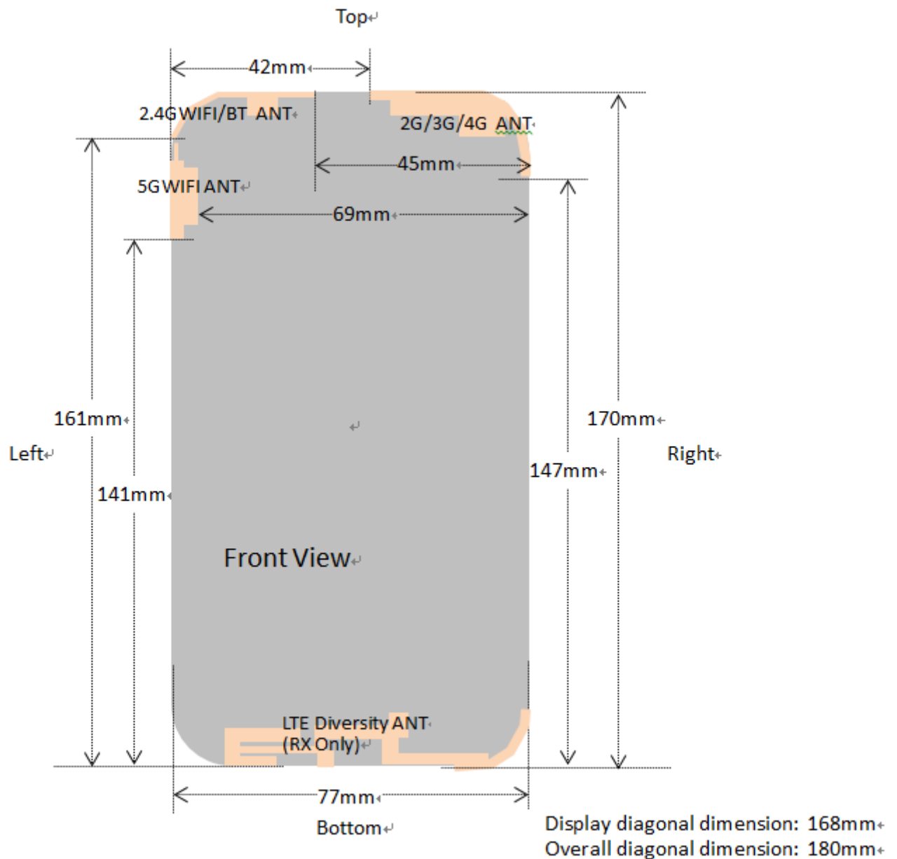
Fig.14.1 EUT Antenna Locations
