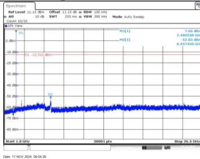
BLE_1M-Ant1-2480-1000~26500-PASS
