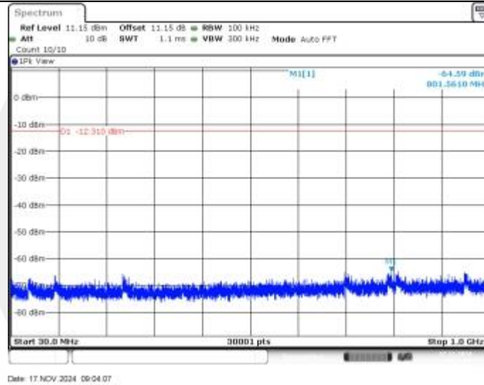
BLE_1M-Ant1-2480-30~1000-PASS
