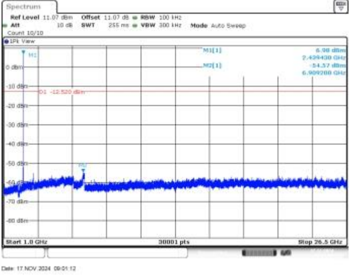
BLE_1M-Ant1-2440-1000~26500-PASS
