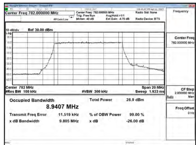
LTE Band 13_256QAM_CH23230_10M_50RB0
