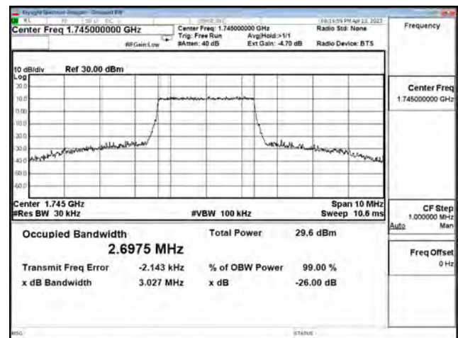
LTE Band 66_256QAM_CH131987_3M_15RB0
