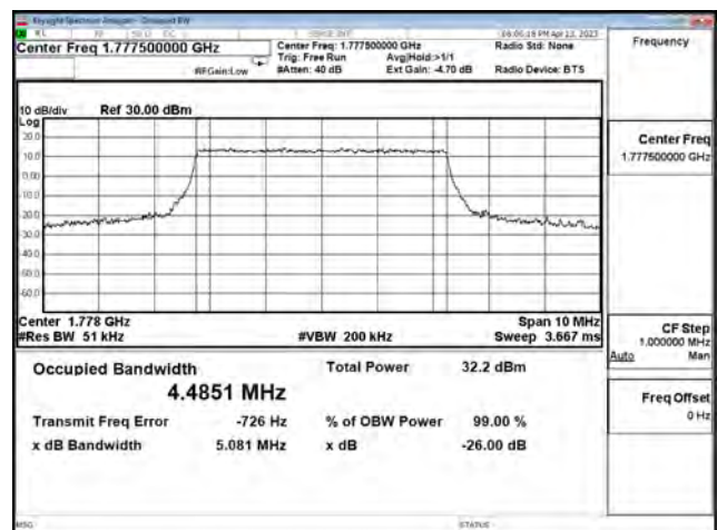
LTE Band 66_16QAM_CH132647_5M_25RB0
