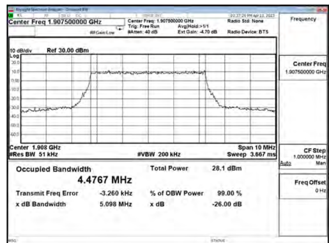
LTE Band 2_256QAM_CH19175_5M_25RB0
