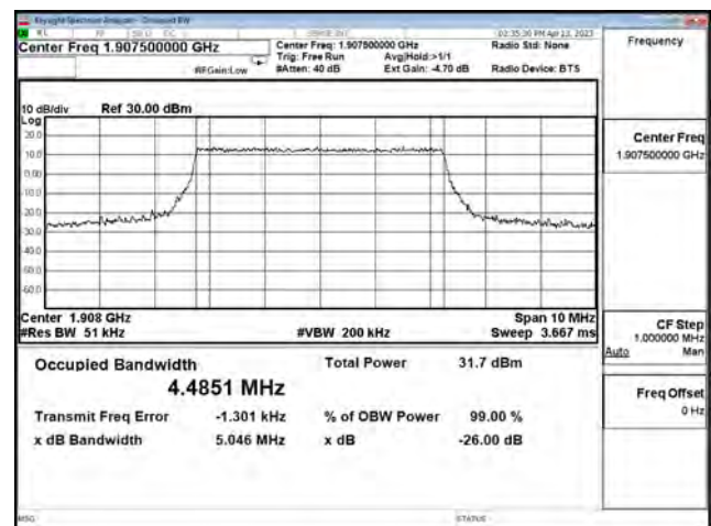
LTE Band 2_16QAM_CH19175_5M_25RB0
