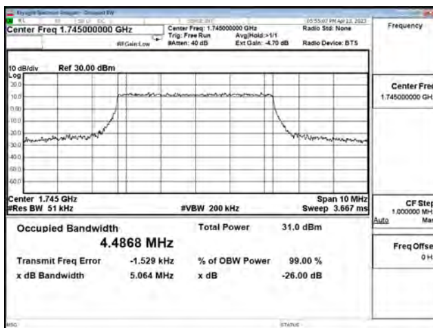
LTE Band 66_16QAM_CH132322_5M_25RB0
