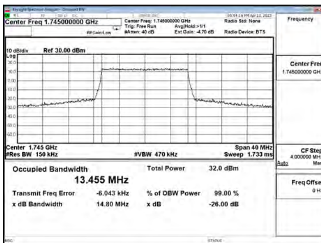
LTE Band 66_16QAM_CH132322_15M_75RB0
