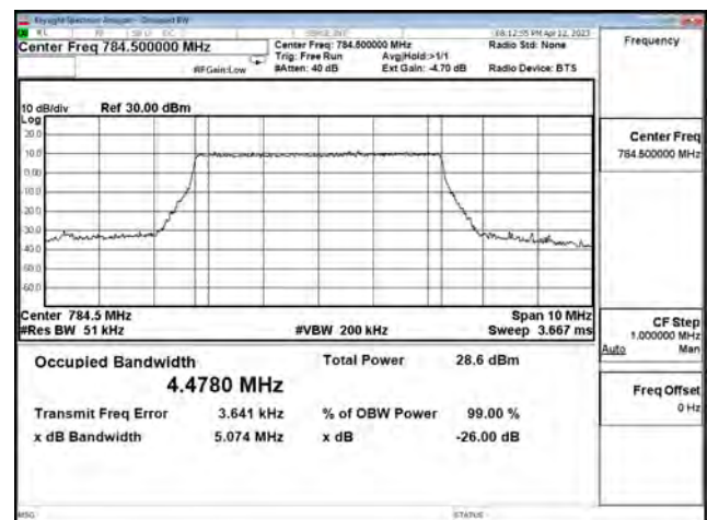
LTE Band 13_256QAM_CH23255_5M_25RB0
