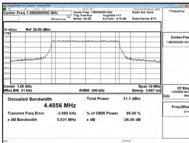
LTE Band 2_16QAM_CH18900_5M_25RB0
