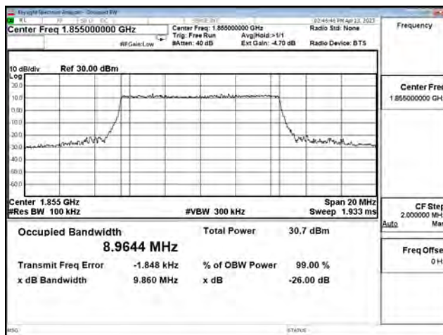
LTE Band 2_64QAM_CH18650_10M_50RB0
