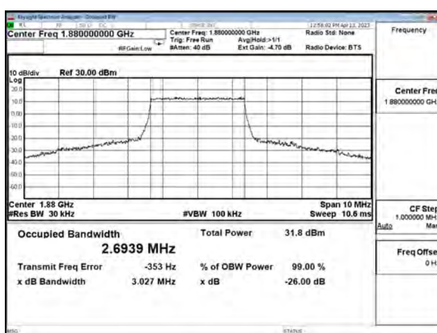
LTE Band 2_16QAM_CH18900_3M_15RB0
