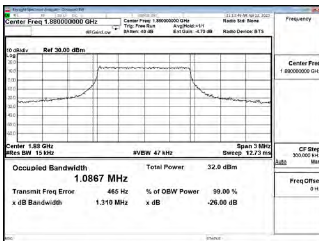
LTE Band 2_16QAM_CH18900_1.4M_6RB0
