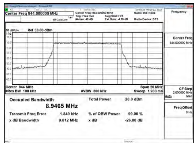
LTE Band 5_256QAM_CH20600_10M_50RB0
