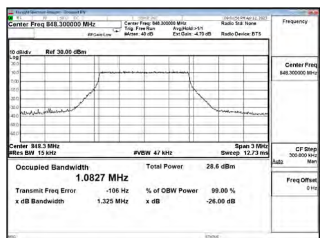
LTE Band 5_256QAM_CH20643_1.4M_6RB0
