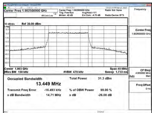
LTE Band 2_16QAM_CH 19125_15M_75RB0
