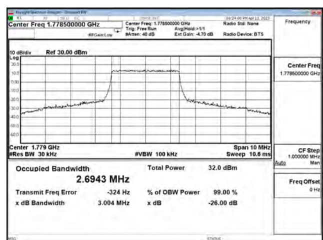
LTE Band 66_16QAM_CH132657_3M_15RB0
