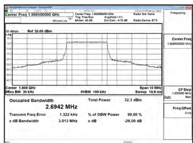
LTE Band 2_16QAM_CH19185_3M_15RB0
