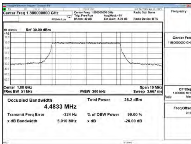
LTE Band 2_256QAM_CH18900_5M_25RB0
