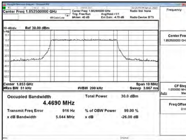
LTE Band 2_64QAM_CH19175_5M_25RB0
