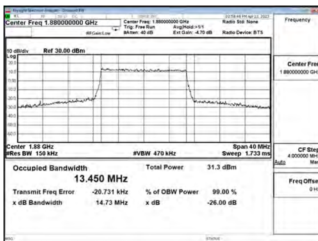
LTE Band 2_16QAM_CH18900_15M_75RB0
