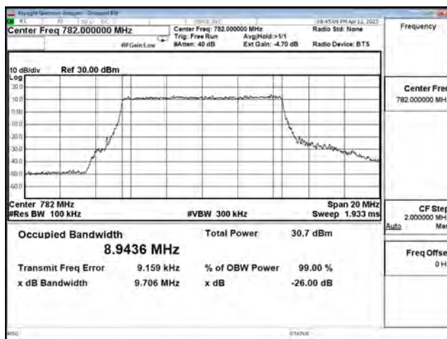
LTE Band 13_64QAM_CH23230_10M_50RB0
