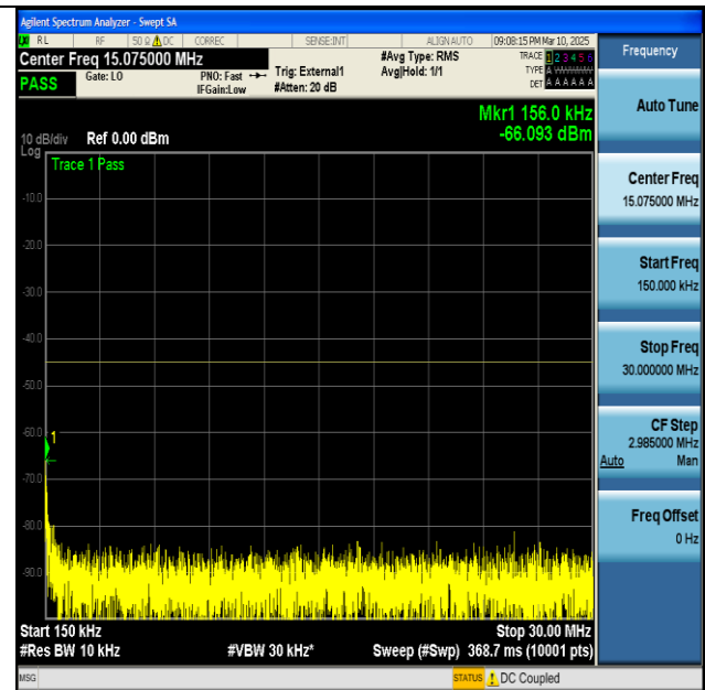
NTNV-n41-PC2-30-100-M-DFT-BPSK-Edge_1RB_Left- 0.15-30-PASS
