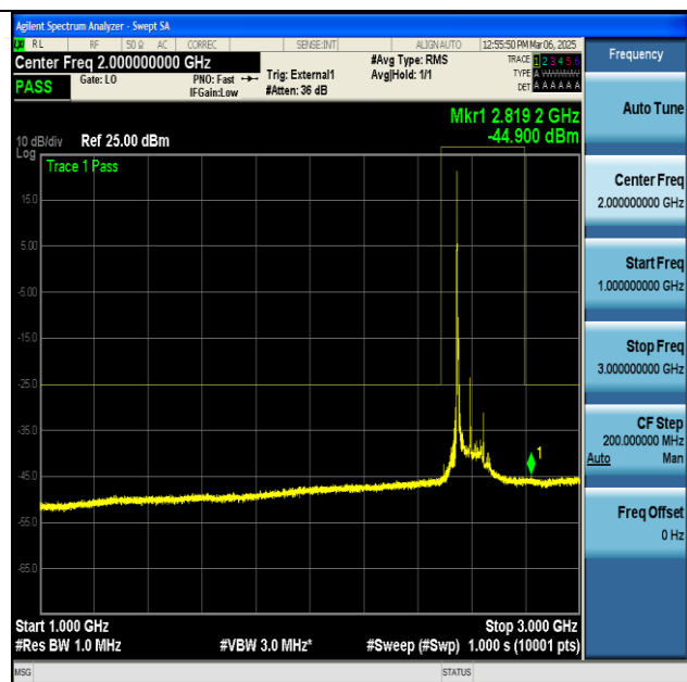
NTNV-n41-PC2-30-100-M-CP-QPSK-Edge_1RB_Left-1000-3000-PASS
