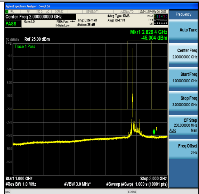
NTNV-n41-PC2-30-100-M-DFT-BPSK-Edge_1RB_Left- 1000-3000-PASS
