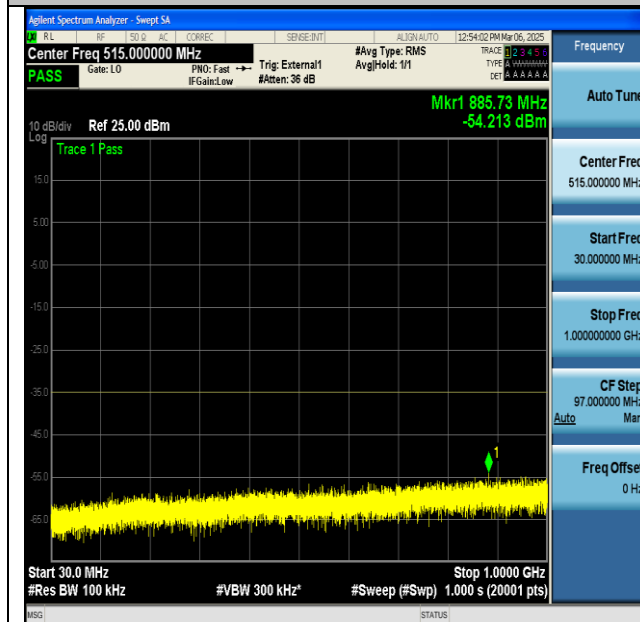
NTNV-n41-PC2-30-100-M-DFT-BPSK-Edge_1RB_Left-30- 1000-PASS
