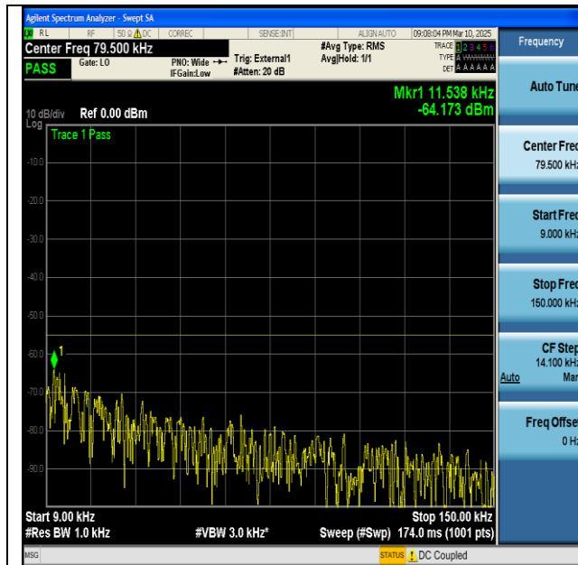
NTNV-n41-PC2-30-100-M-DFT-BPSK-Edge_1RB_Left- 0.009-0.15-PASS
