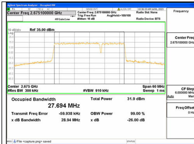
41C / 20+10MHz / 16QAM/ High CH
