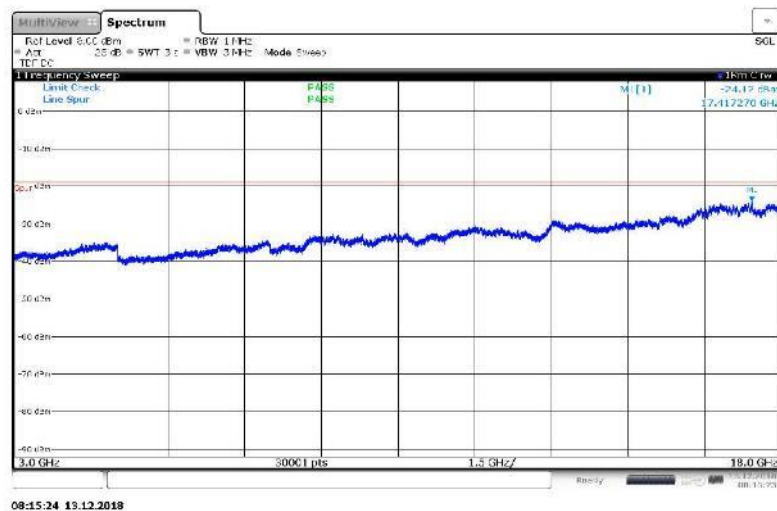
Figure 193 Spurious Emissions (3 GHz – 18GHz) – 256QAM (2645 MHz, 2665 MHz, 2x20 MHz Channel BW)
