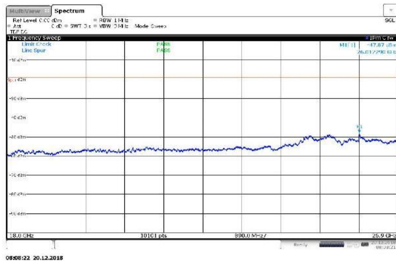
Figure 194 Spurious Emissions (18GHz – 26.9GHz) – 256QAM (2645 MHz, 2665 MHz, 2x20 MHz Channel BW)
