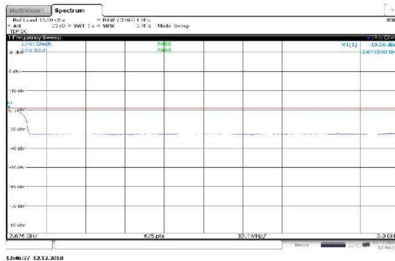
Figure 174 Spurious Emissions (2.676 GHz – 3 GHz) – QPSK (2645 MHz, 2665 MHz, 2x20 MHz Channel BW)
