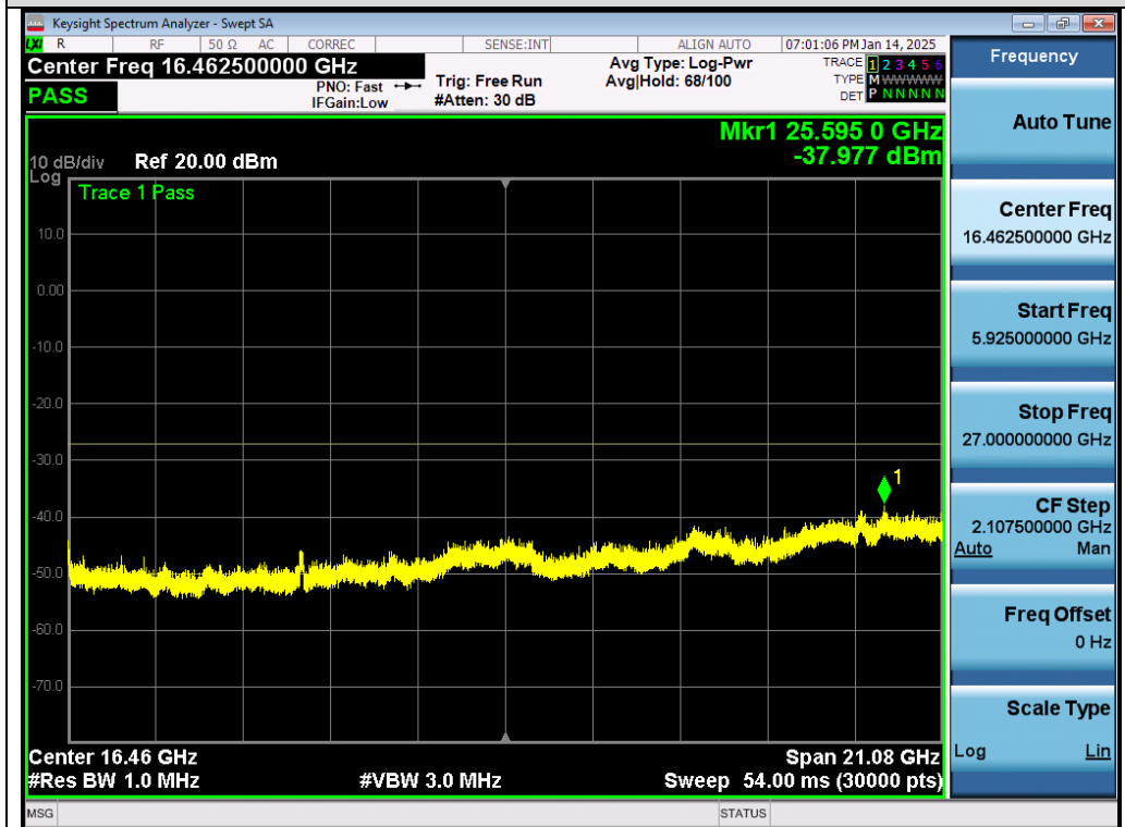
Test_Graph_802.11ac80_Chain A_5775_MCS0_Frequency Band4
