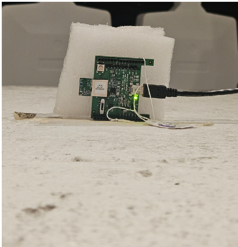
Figure 1. Radiated Emissions Test Setup, Front
