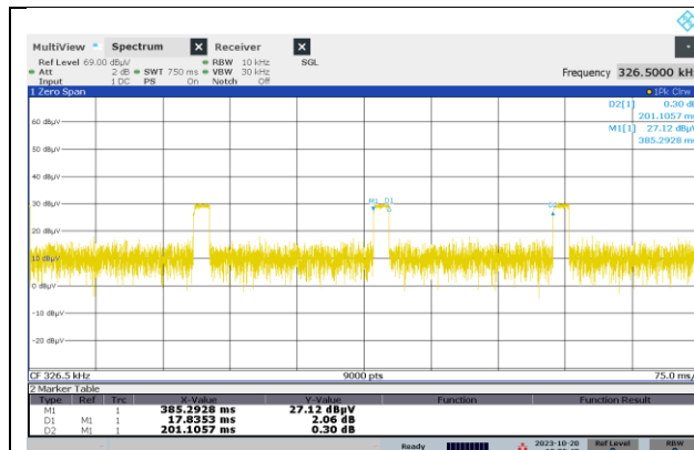
CONFIGURATION 1 (326.5kHz)
