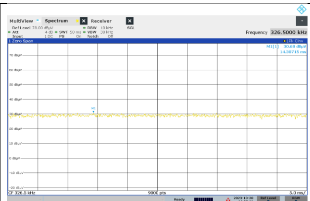
CONFIGURATION 2 (326.5kHz)
