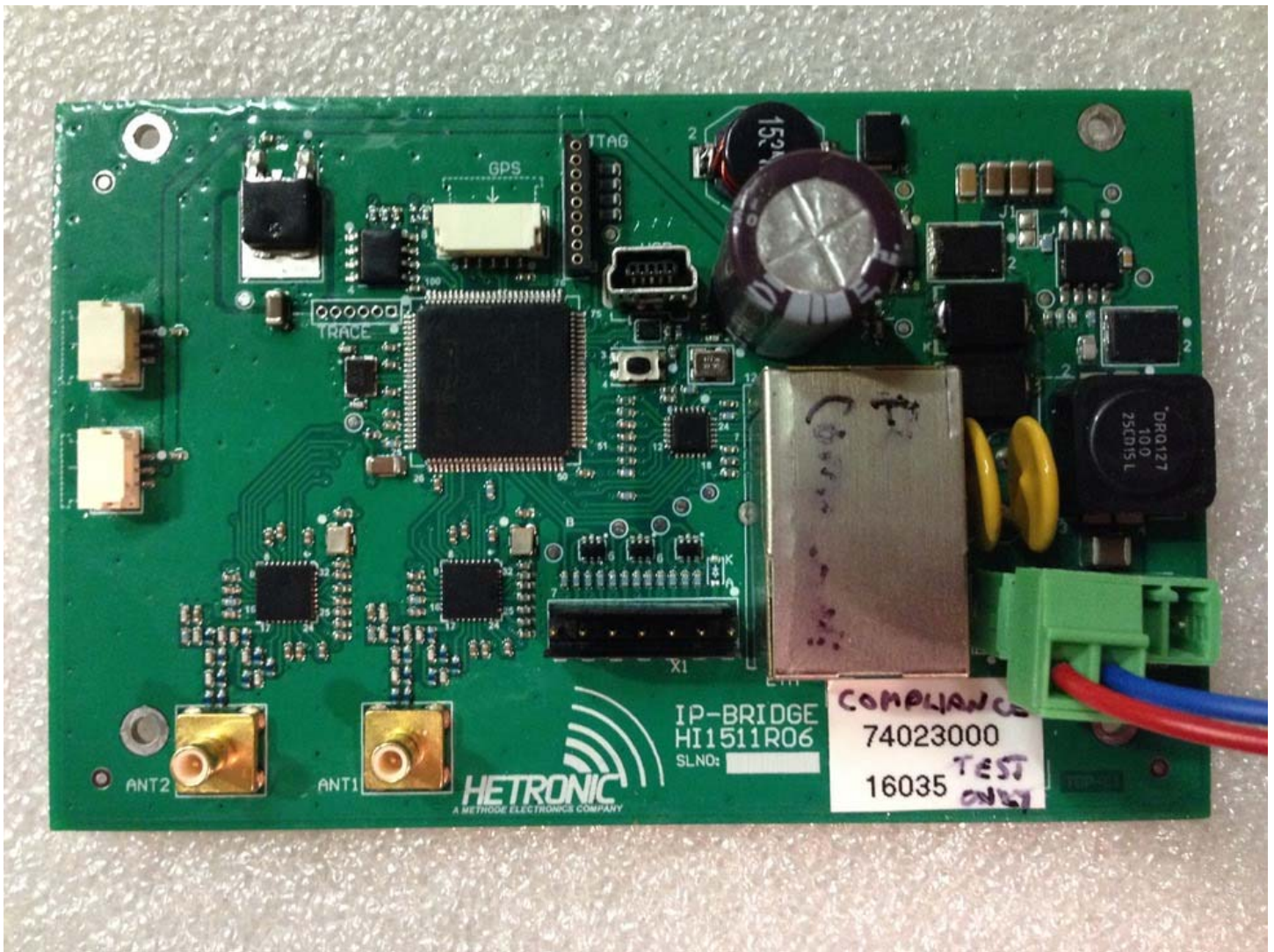
IP-Bridge Board, Side 1
