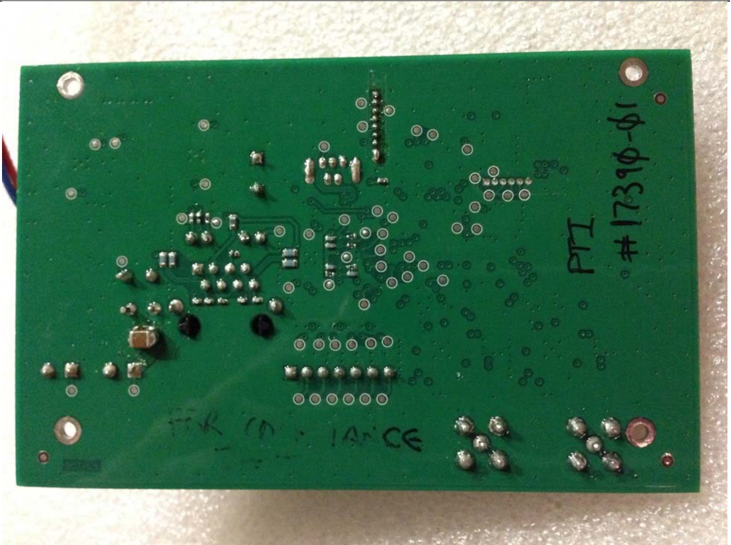
IP-Bridge Board, Side 2
