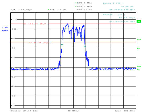
Frequency: 24.15
