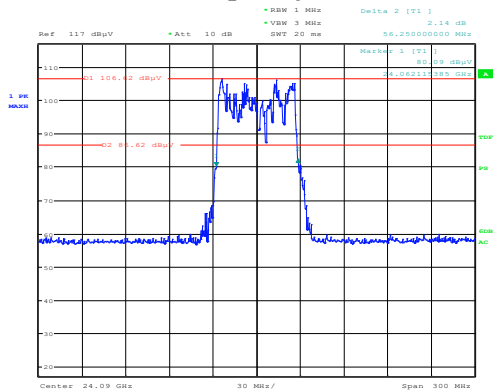
Frequency: 24.09
