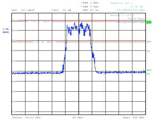
Frequency: 24.21
